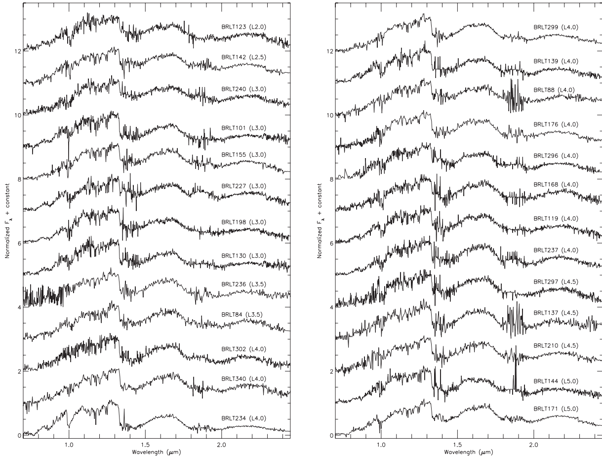
Figure 3. The X-shooter spectra of the objects presented here, sorted in ascending order of spectral type (L2.0–L5.0). All spectra are normalized at 1.28 \mu\text{m} and offset vertically by increments of one flux unit.
