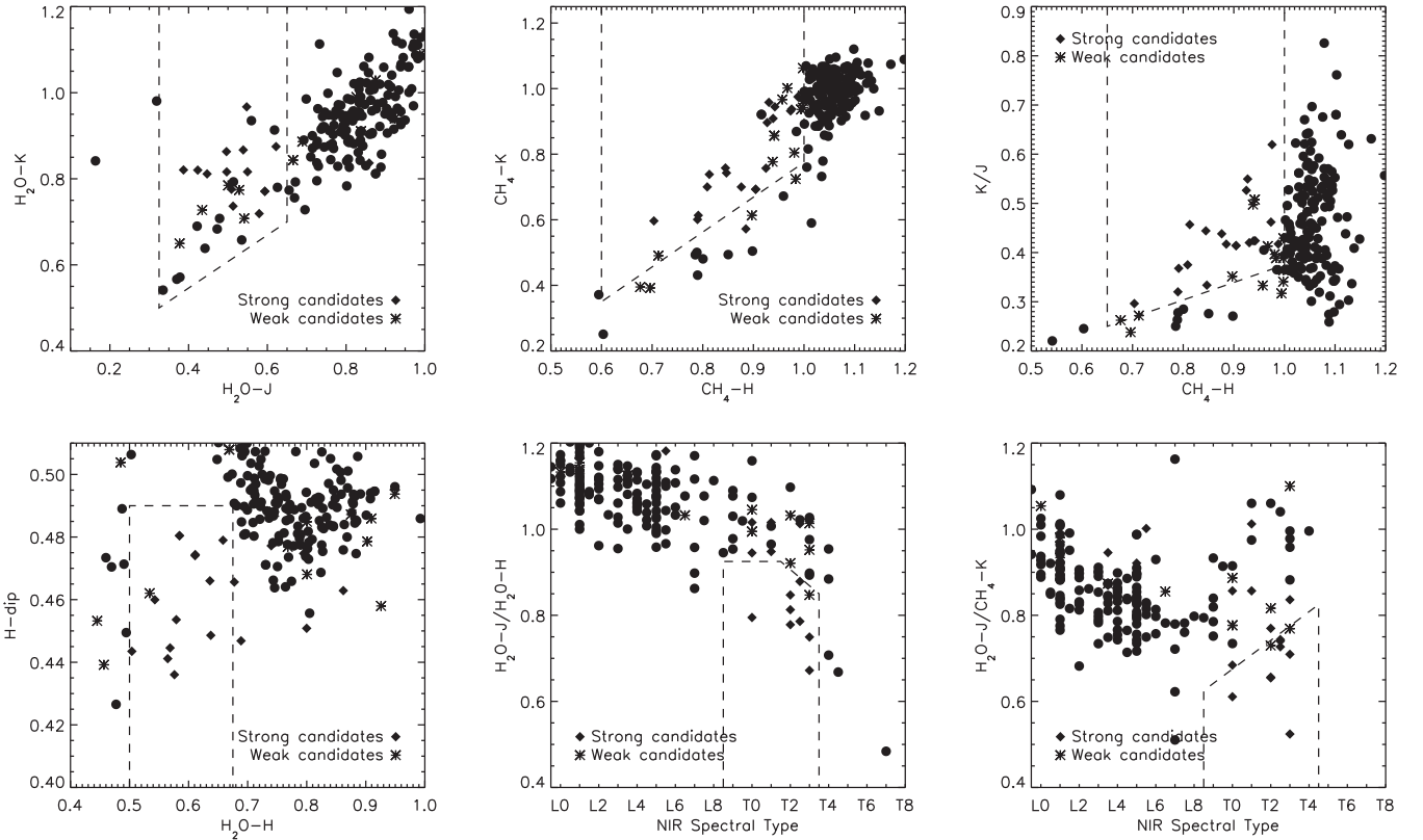
Figure 6. The index–index and index–spectral type plots used for binary candidate selection. The dashed lines enclose the selection areas, as defined in Table 3. Weak candidates are marked with stars, while strong candidates are marked with diamonds.
