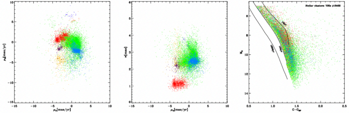
Fig. C.4. Proper motions in RA and Dec, parallaxes, and CAMDs of the YSOs associated with the Orion complex. The symbol colours of the sub-clusters are the same as in Fig. C.3. Three representative solar metallicity isochrones from the Pisa models are also shown.
