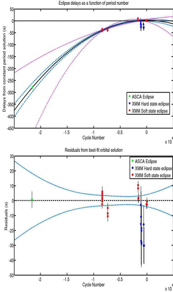
Figure 2. (Top panel) Eclipse time delays (egress times) with respect to a constant orbital period model plotted versus orbital cycle. T_0 (therefore cycle one) corresponds to MJD = 57114.66871. The red and blue circles show the eclipse egress delays corresponding to soft and hard states of the source, respectively, which were observed with XMM-Newton whereas the green circle shows the eclipse egress delay derived from the single eclipse in the ASCA data (1994). The black solid and blue dashed lines show the best-fitting orbital solution of the combined XMM-Newton and ASCA data and the 68 per cent confidence region. The magenta dashed lines show the 68 per cent confidence uncertainty on the best-fitting orbital solution obtained by fitting the XMM-Newton data only. (Bottom panel) Residuals of the best-fitting orbital solution. Significant scatter is observed.
