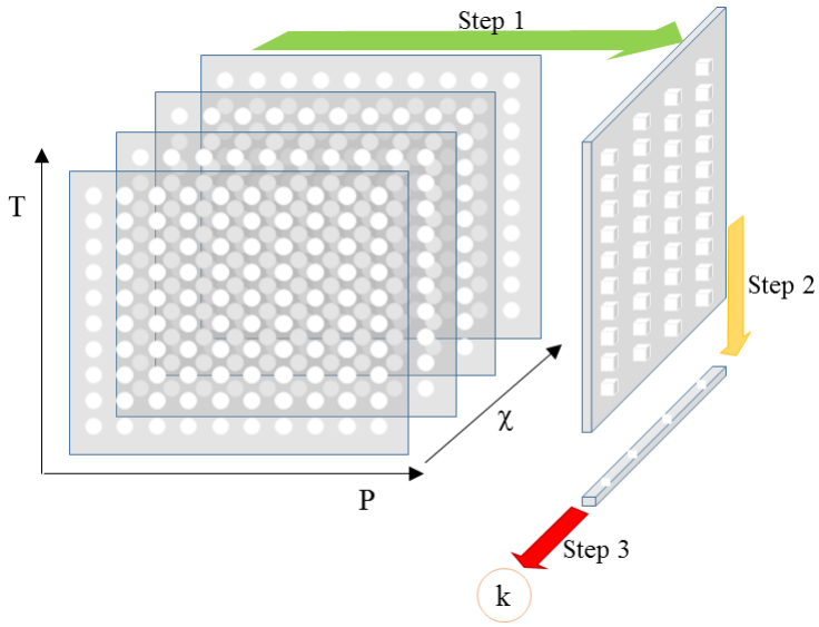
224 Figure 1: Representation in the space of the parameters of the 3-steps interpolation scheme described 225 in Section 2.2 to obtain the absorption coefficients at the desired T and P for a given value of \chi .
