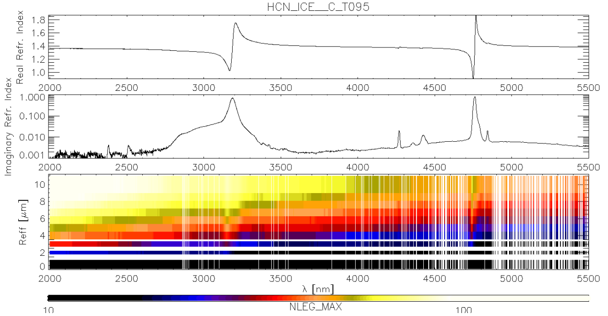
Figure 4: Top and middle panels: real and imaginary parts of HCN ice refractive index. Lower panel: Minimum number of Legendre coefficients required to describe the phase function of a lognormal size distribution of spherical particles with v_{\text{eff}} = 0.3 computed according to Wiscombe (1980). Blank regions represent wavelengths and radii removed after the optimization process (see Section 3.2).
