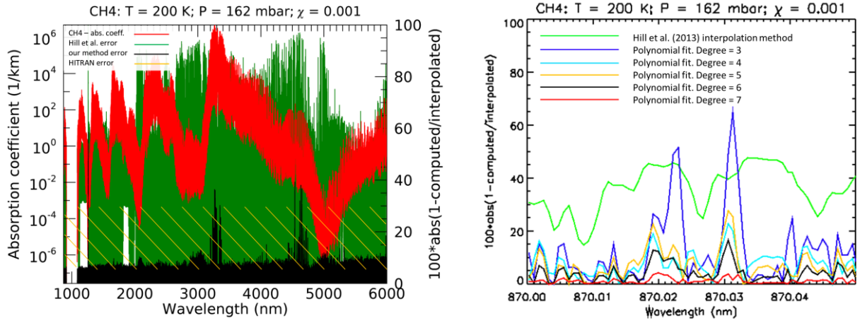
Figure 2: At left: relative differences (right axis) between \text{CH}_4 absorption coefficients computed with P = 162 mbar, T = 200 K, \chi = 0.001 between 870 nm and 6000 nm (red line, left ordinate axis) and those interpolated with our method (black line) and with that from Hill et al. (2013) (green line). The orange oblique lines indicate the range of uncertainty due to HITRAN line intensity error (Section 2.1). At right: zoom in the range 870.00 nm – 870.05 nm of the relative differences between the computed absorption coefficients (left panel, red line) and the ones interpolated with polynomial fits of different degree: 3 rd degree (blue line), 4 th degree (cyan line), 5 th degree (orange lines), 6 th degree (black line) and 7 th degree (red line). The relative difference obtained with Hill et al. (2013) interpolation method is shown in green.
