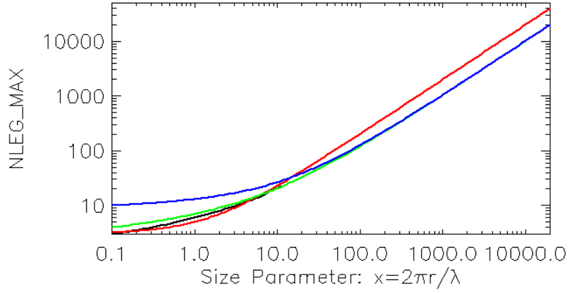
Figure 3: Minimum number of Legendre coefficients required to describe the phase function of a single homogeneous spherical particle of HCN ice, computed according to Wiscombe (1980) (Black), Lenoble (1993) (Red), Bohren and Huffman (1983) (Green) and Mishchenko et al (2002) (Blue).
