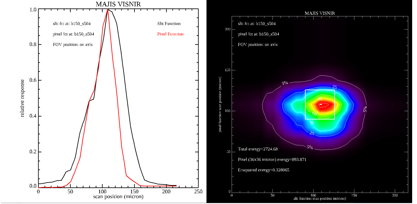
FIG. 8. Ensquared Energy Distribution computed for the VISNIR channel at b=150 and physical sample=504 (on axis position). Left panel: normalized slit and pixel functions as a function of spatial scan. Right panel: EED derived from the normalized slit and pixel functions. The colors run from white ( =1 ) to green ( =0.5 ) to black ( =0 ). The total energy value corresponds to the integral computed on the entire distribution while the nominal pixel energy refers to the integral limited to the 36 \times 36 \mu\text{m} (white square) area. The ensquared energy value (32.8%) is the ratio between the total energy and the energy effectively measured by the pixel.
