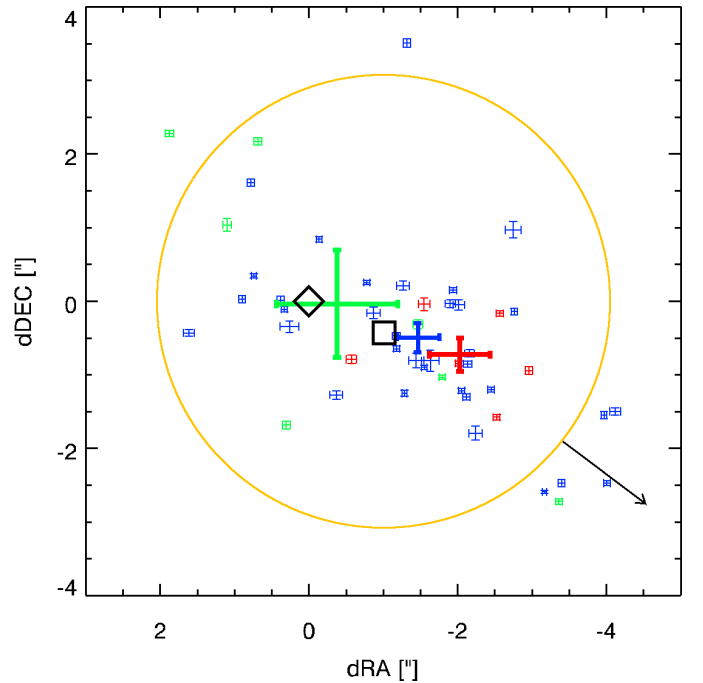
Fig. 3. (NEO)WISE coordinate offsets relative to an origin at MM1 (from Brogan et al. 2019). Pre-burst, burst, and post-burst data are shown in blue, red and green. Thick error bars represent mean positions while individual appear thin. Positions of MM1 and MM3 (measured with ALMA) are marked by the diamond and the square, respectively. The arrow points toward the bright 2MASS J17431001–2951460, which is at a distance of 9''.9 from the (0,0) position. The yellow circle indicates the W1 image FWHM of 6''.1 .
