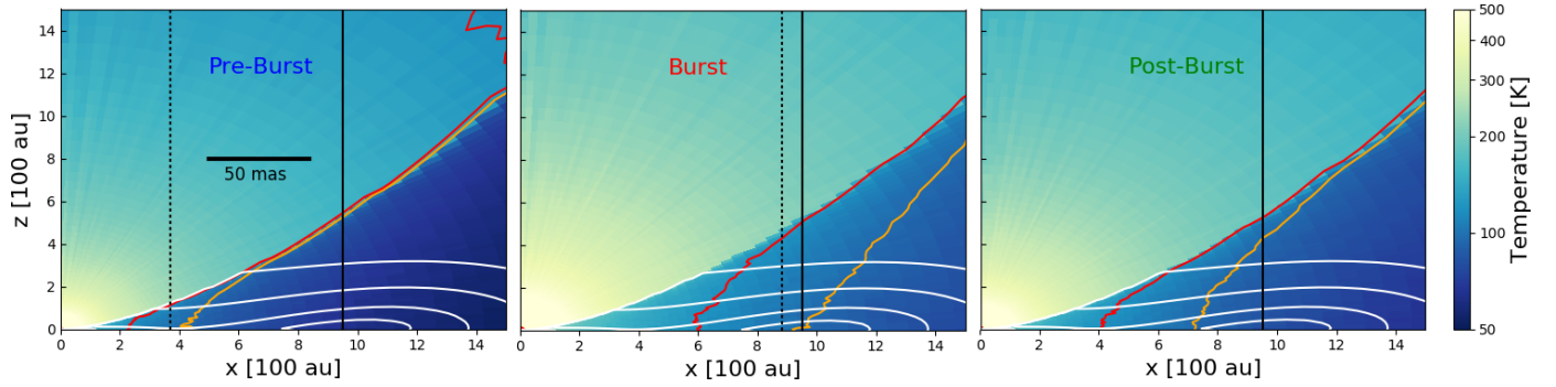
Fig. 8. Temperature distribution of the mean model in the x - z plane (innermost part of first quadrant) for the pre-burst (left), burst- (center) and post-burst epochs (right). The orange and red lines enclose the temperature range from 94 K (orange) to 120 K (red) during the pre- and burst epochs, respectively. The white contours mark gas particle volume densities of n_{\text{H}_2} = [0.2, 0.3, 0.5, 1] \times 10^8 \text{ cm}^{-3} which decrease with increasing z . The vertical solid black line indicates the outer radius of the disk. The dashed black lines mark the radius of the maser ring from the first and 4th epoch of the VLBI observations (Burns et al. 2020, and in prep.). The length of the black bar corresponds to 50 mas.
