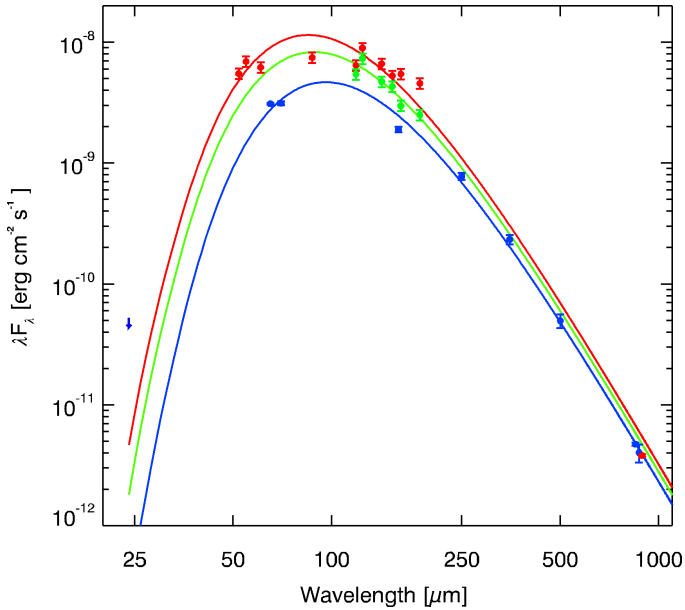
Fig. 4. Observed FIR/(sub)mm SEDs showing pre-burst Herschel / AKARI data (blue) and FIFI-LS burst values (red) together with the corresponding (sub)mm fluxes from Brogan et al. (2019). The upper 24 \mu\text{m} MIPS limit is indicated as well. The solid lines represent the red-dened graybody fits (cf. Sect. 4.1). The second epoch FIFI-LS data and the corresponding fit appear in green.
