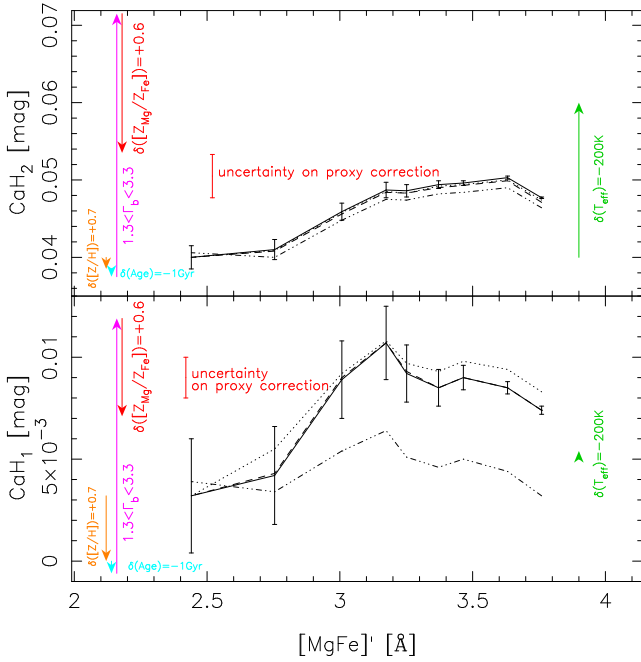
Figure B3. \text{CaH}_1 (bottom) and \text{CaH}_2 (top) radial gradients for NGC 4552, i.e. the same as Fig. B1 but for CaH, rather than Na, features. The telluric contamination of these indices does not allow us to trust the index absolute values. However, the radial gradient for \text{CaH}_2 is robust, while for \text{CaH}_1 we can exclude an increase of the index with radius (leftwards in the plot), as it would be the case for a constant IMF (see the text). Notice that \text{CaH}_2 is fully consistent with our results of a varying IMF for NGC 4552. In general, because of the different sensitivity of the two indices to a variation in T_{\text{eff}} (green arrows), one cannot explain the behaviour of both CaH features without a varying IMF with radius.
