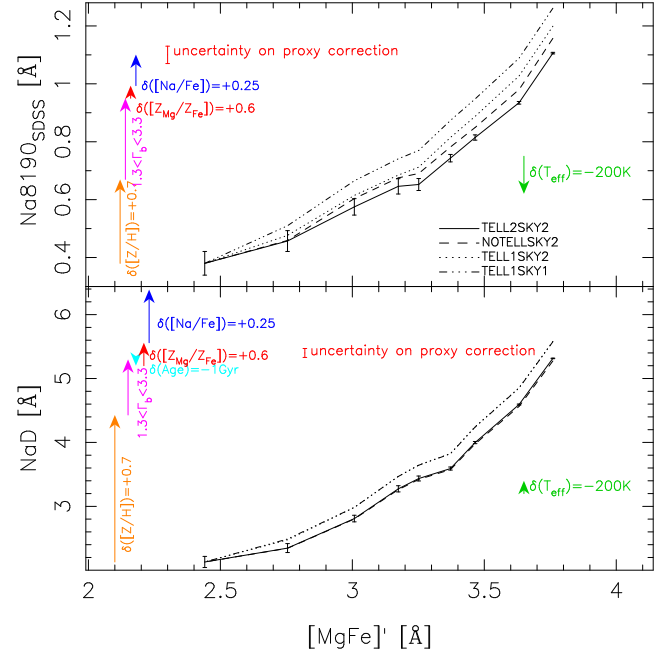
Figure B1. The Na I 8190 (top panel) and NaD (bottom panel) index radial profiles of NGC 4552 are plotted as a function of the total metallicity indicator [MgFe]' . The black curves with different line types (see the black legend in the upper panel) correspond to different methods to treat telluric absorption, i.e. methods TELL1 and TELL2 (see the text) and no telluric correction ( NOTELL ), as well as different sky subtraction procedures (methods SKY1 and SKY2 , see the text). The black error bars are the maximum uncertainties (among different methods), quoted at the 1\sigma level. In both panels, arrows show the expected variation of the indices (for SSP models) because of the metallicity (orange), IMF (magenta), age (cyan), and [Z_{Mg}/Z_{Fe}] (red) gradients for NGC 4552 (Section 4.2). Notice that the effect of varying age is not shown for Na I 8190, as it is completely negligible for this index. The effect of varying [Na/Fe] abundance and T_{eff} are also shown as blue and green arrows, respectively.
