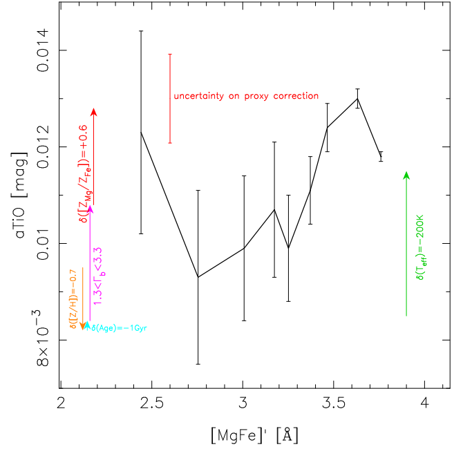
Figure B4. Radial profile of the interpolated aTiO index for NGC 4552 (see the text). Notice the large error bars, in the outer radial bins (left in the plot) preventing us to use this index to significantly constrain the IMF gradient. Notice that because the index is not affected by telluric absorption, while airglow contamination is avoided by our interpolation procedure, no difference exists among different reduction procedures and we did not apply any rigid shift to the line strengths (as, e.g. in Figs B1 and B3).
