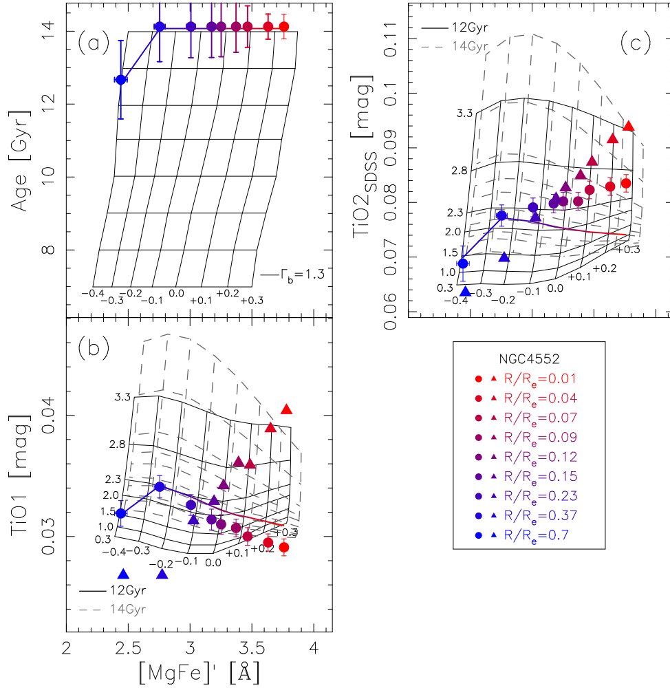
Figure 6. Fitting results for our reference high-mass galaxy, NGC 4552, obtained by leaving age, metallicity, and \delta Ti as free parameters, but assuming a fixed, standard (Kroupa-like), IMF. Panel (a): coloured dots, with error bars, are age estimates from spectral fitting, for a Kroupa IMF. The grid shows the effect of varying metallicity on the [MgFe]' index, for SSPs with a Kroupa-like IMF ( \Gamma_b = 1.35 ) and different ages. Panels (b) and (c): the solid and dashed grids show line strengths for SSP models with varying \Gamma_b and [Z/H] , for two representative ages of 12 (outermost radial bin; see panel a) and 14 Gyr (innermost bins), respectively. The filled circles, with error bars, are the [\alpha/Fe] -corrected and \delta Ti -shifted line strengths, while triangles plot raw line strengths (as measured on the spectra). Notice that triangles are the same as in panels (b) and (c) of Fig. 3. Since \delta Ti is a free-fitting parameter, the \delta Ti values are not the same when assuming a fixed, relative to a varying, IMF. Hence, coloured dots in panels (b) and (c) are not the same as those in Fig. 3. In all panels, solid-coloured curves show the best-fitting solutions, with colour varying from red, in the galaxy centre, through blue, at larger galactocentric distances. The same colour coding applies to dots and triangles (see the legend in the lower-right corner of the plot). For the two outermost bins, the best-fitting Kroupa-like models (coloured curves) match the [\alpha/Fe] -corrected and \delta Ti -shifted line strengths (filled circles). On the contrary, in the five innermost bins, the model TiO_2 deviates by more than 3\sigma from the observations, while significant deviations (at 2\sigma ) are also seen for TiO_1 .
