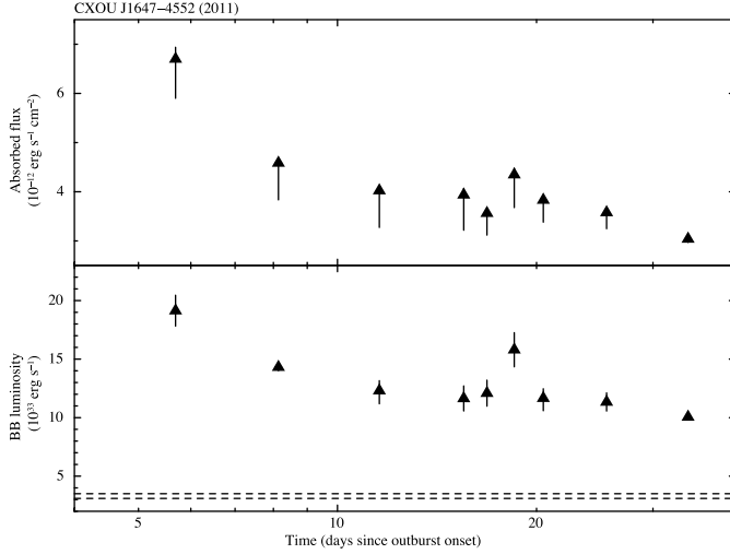
Figure D14. Left-hand panel: temporal evolution of the fluxes and luminosities for the BB model applied to the X-ray data of the 2011 outburst of CXOU J164710.2–455216. The dashed lines mark the 1\sigma c.l. range for the quiescent luminosity (see Table 4). A distance of 4 kpc was assumed. Right-hand panel: temporal evolution of the bolometric luminosity with the best-fitting decay model superimposed.
