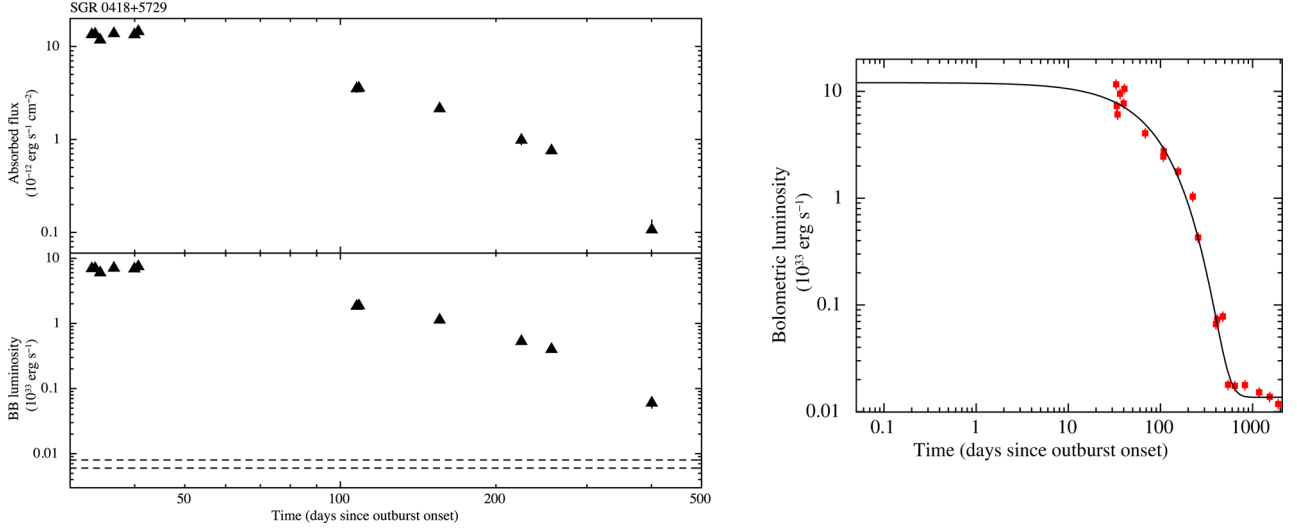
Figure D10. Left-hand panel: temporal evolution of the fluxes and luminosities for the BB model applied to the Swift XRT data of the outburst of SGR 0418+5729. The dashed lines mark the 1-\sigma c.l. range for the quiescent luminosity (see Table 4). A distance of 2 kpc was assumed. Right-hand panel: temporal evolution of the bolometric luminosity with the best-fitting decay model superimposed.
