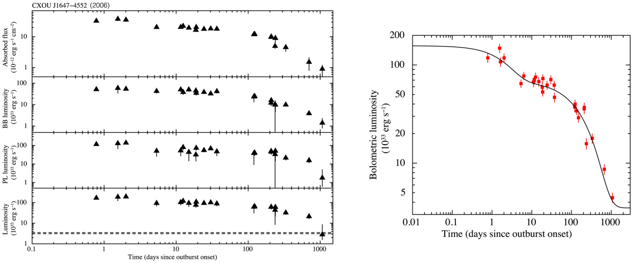
Figure D5. Left-hand panel: temporal evolution of the fluxes and luminosities for the BB+PL model applied to the X-ray data of CXOU J164710.2–455216. The dashed lines mark the 1\sigma c.l. range for the quiescent luminosity (see Table 4). A distance of 4 kpc was assumed. Right-hand panel: temporal evolution of the bolometric luminosity with the best-fitting decay model superimposed.
