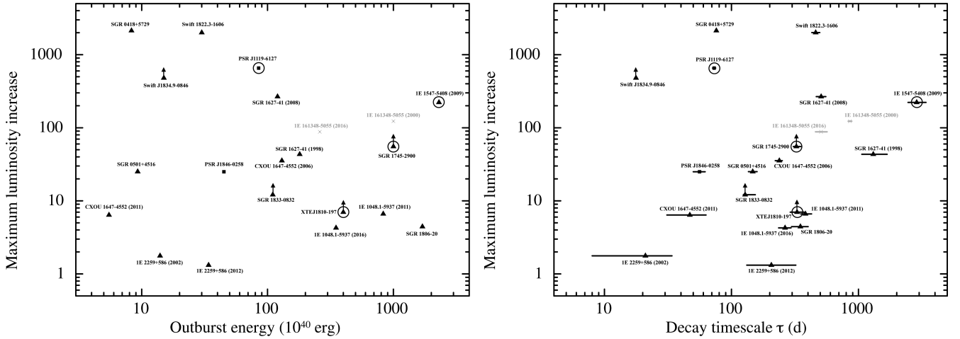
Figure 8. Left-hand panel: maximum luminosity increase as a function of the total energy released during the outburst. Right-hand panel: maximum luminosity increase as a function of the decay time-scale.
