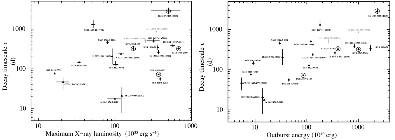
Figure 7. Left-hand panel: decay time-scale as a function of the maximum X-ray luminosity at the peak of the outburst. Right-hand panel: decay time-scale as a function of the total energy released during the outburst.
