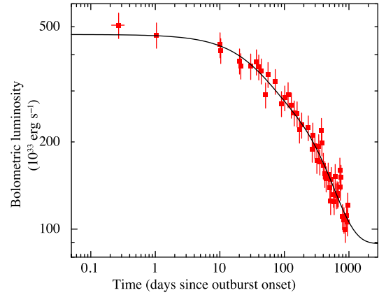
Figure D15. Left-hand panel: temporal evolution of the fluxes and luminosities for the BB model applied to the Swift XRT data of the 2011 outburst of 1E 1048.1–5937. The dashed lines mark the 1\sigma c.l. range for the quiescent luminosity (see Table 4). A distance of 9 kpc was assumed. Right-hand panel: temporal evolution of the bolometric luminosity with the best-fitting decay model superimposed.
