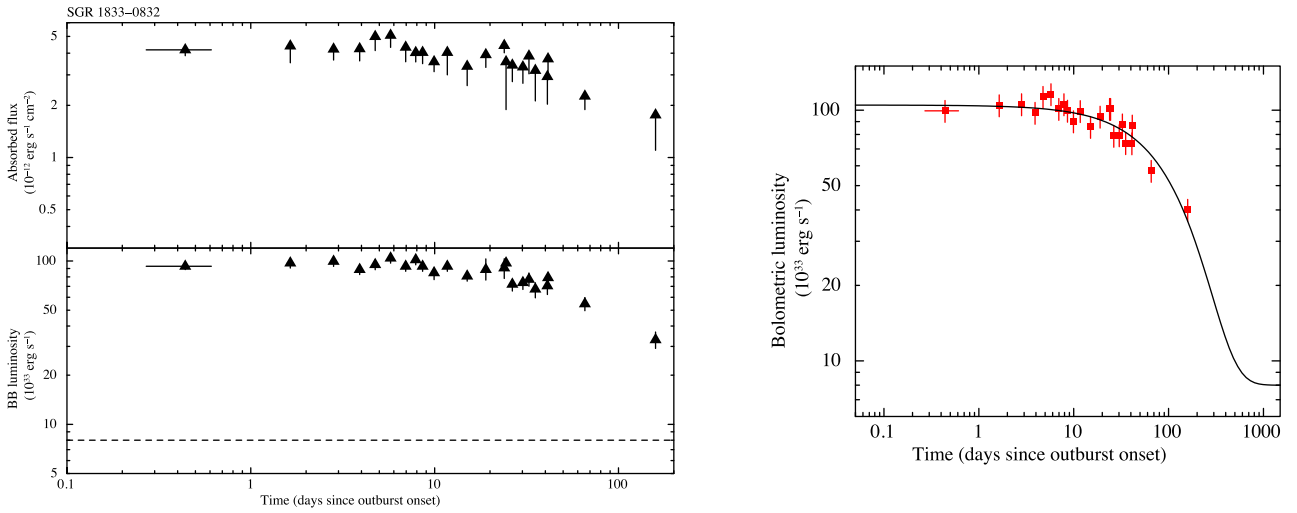
Figure D11. Left-hand panel: temporal evolution of the fluxes and luminosities for the BB+PL model applied to the Swift XRT data of the outburst of SGR 1833-0832. The dashed line marks the upper limit (at the 3\sigma c.l.) for the quiescent luminosity (see Table 4). A distance of 10 kpc was assumed. Right-hand panel: temporal evolution of the bolometric luminosity with the best-fitting decay model superimposed.
