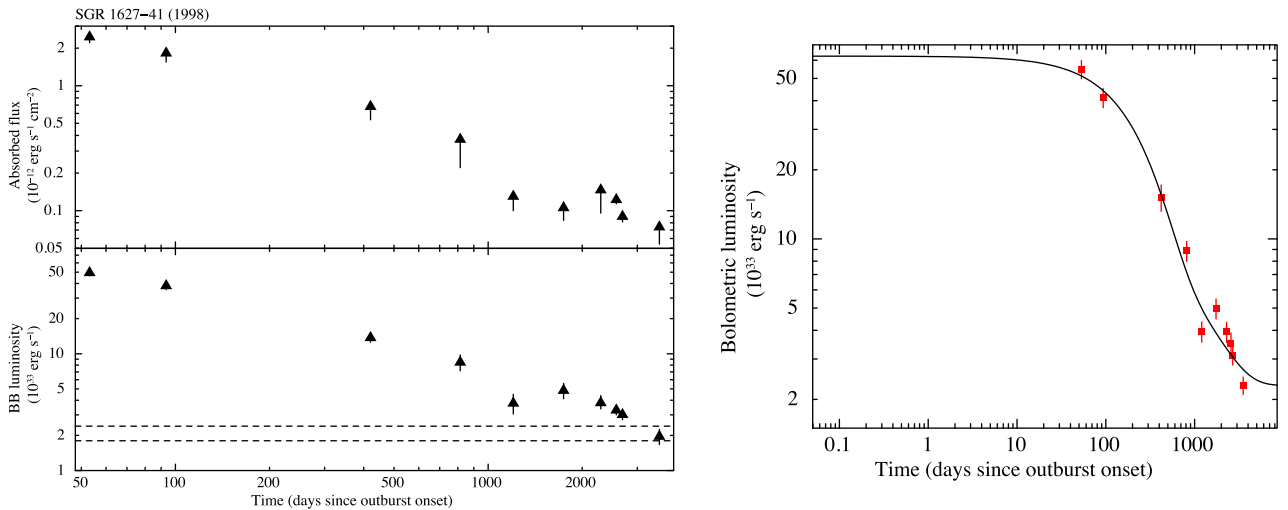
Figure D1. Left-hand panel: temporal evolution of the fluxes and luminosities for the BB model applied to the X-ray data of the 1998 outburst of SGR 1627–41. The dashed lines mark the 1\sigma c.l. range for the quiescent luminosity (see Table 4). A distance of 11 kpc was assumed. Right-hand panel: temporal evolution of the bolometric luminosity with the best-fitting decay model superimposed.
