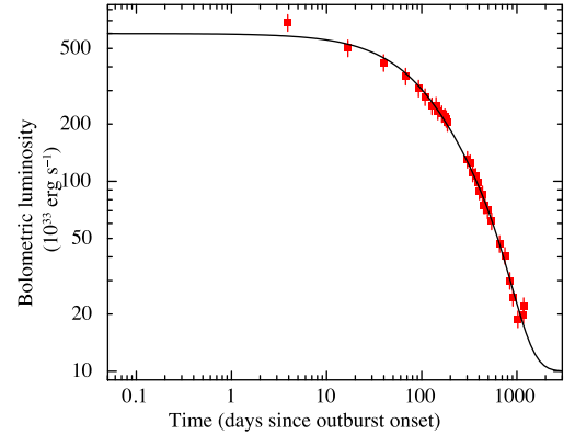
Figure D17. Left-hand panel: temporal evolution of the fluxes and luminosities for the BB+PL model applied to the Chandra data of the outburst of SGR 1745-2900. A distance of 8.3 kpc was assumed. Right-hand panel: temporal evolution of the bolometric luminosity with the best-fitting decay model superimposed.
