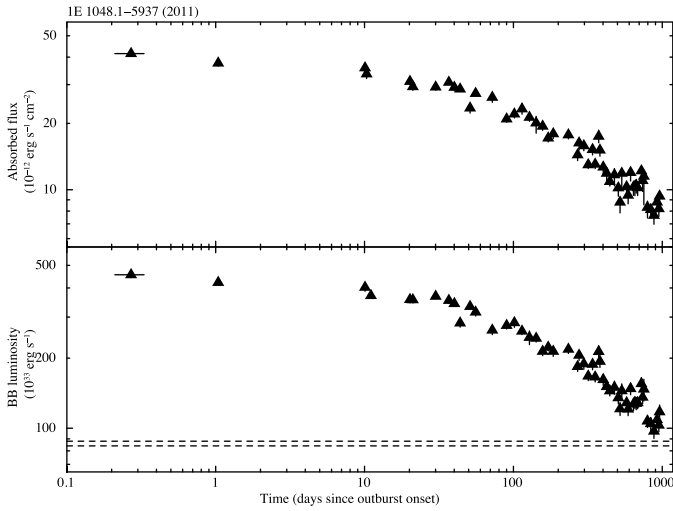
Figure D15. Left-hand panel: temporal evolution of the fluxes and luminosities for the BB model applied to the Swift XRT data of the 2011 outburst of 1E 1048.1–5937. The dashed lines mark the 1\sigma c.l. range for the quiescent luminosity (see Table 4). A distance of 9 kpc was assumed. Right-hand panel: temporal evolution of the bolometric luminosity with the best-fitting decay model superimposed.
