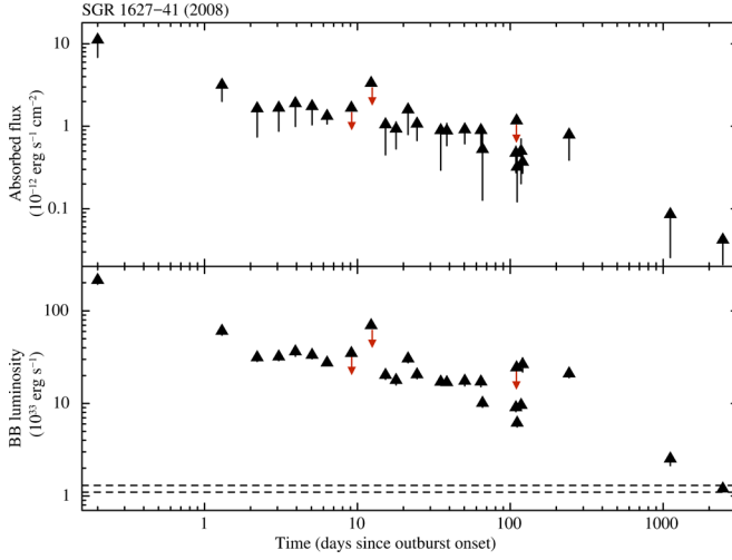
Figure D6. Left-hand panel: temporal evolution of the fluxes and luminosities for the BB model applied to the X-ray data of the 2008 outburst of SGR 1627–41. The dashed lines mark the 1\sigma c.l. range for the quiescent luminosity (see Table 4). The red downward arrowheads indicate the 3\sigma upper limits. A distance of 11 kpc was assumed. Right-hand panel: temporal evolution of the bolometric luminosity with the best-fitting decay model superimposed.
