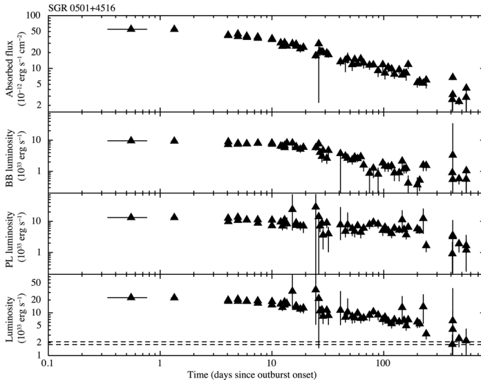
Figure D7. Left-hand panel: temporal evolution of the fluxes and luminosities for the BB+PL model applied to the Swift XRT data of SGR 0501+4516. The dashed line marks the approximate value for the quiescent luminosity (see Table 4). A distance of 1.5 kpc was assumed. Right-hand panel: temporal evolution of the bolometric luminosity with the best-fitting decay model superimposed.
