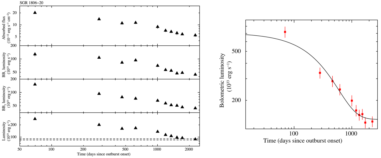
Figure D4. Left-hand panel: temporal evolution of the fluxes and luminosities for the 2BB model applied to the XMM-Newton data of SGR 1806–20. The dashed lines mark the 1\sigma c.l. range for the quiescent luminosity (see Table 4). A distance of 8.7 kpc was assumed. Right-hand panel: temporal evolution of the bolometric luminosity with the best-fitting decay model superimposed.
