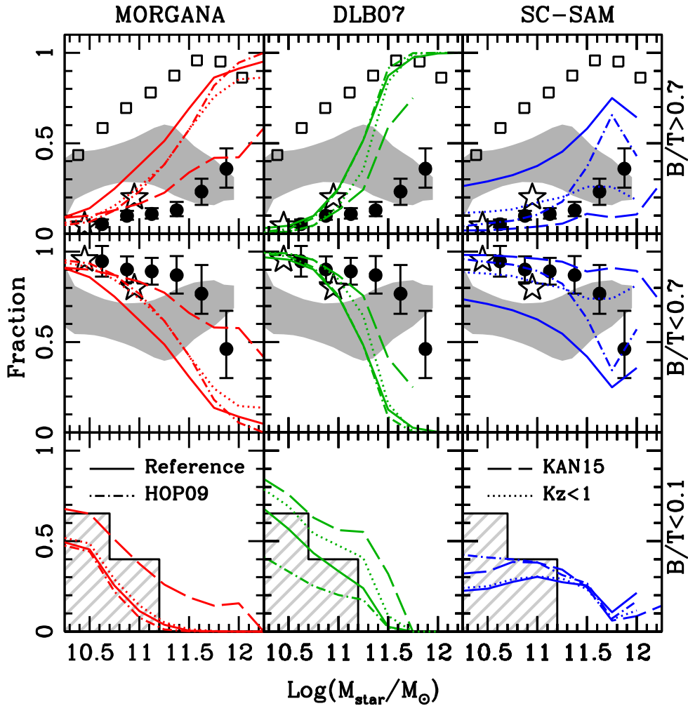
Figure 4. Distribution of galaxies among morphological types as a function of stellar mass. Filled circles refer to the total fraction of ellipticals in Wilman et al. (2013), while open squares to the total fraction of early-type galaxies from the sample of Hyde & Bernardi (2009). Shaded areas represent the results from the Mendel et al. (2014) decomposition, while stars and hatched histograms refer to Fisher & Drory (2011) sample. See the main text for more details on the observational samples considered. Line types and colours refer to SAM predictions as in Fig. 2. Right-hand labels indicate the model galaxy B/T range considered in each row.
