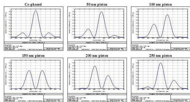
Figure 6. Overview of the expected PSF as measured by the SPL camera corresponding to various differential piston between the shells.
