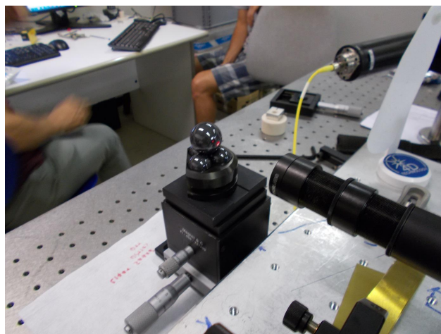
Figure 9. Commercial random ball on its mount during the test measurement of the lens system (the optical tube on the right side).
