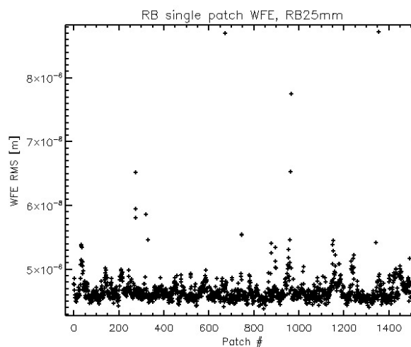
Figure 10. WFE of the measurement patches of the random ball.
