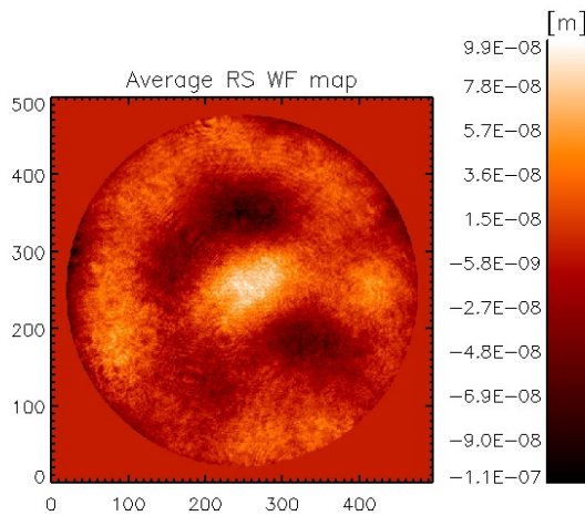
Figure 11. WF of the lens system, obtained after averaging 1500 frames while the RB was rotated
