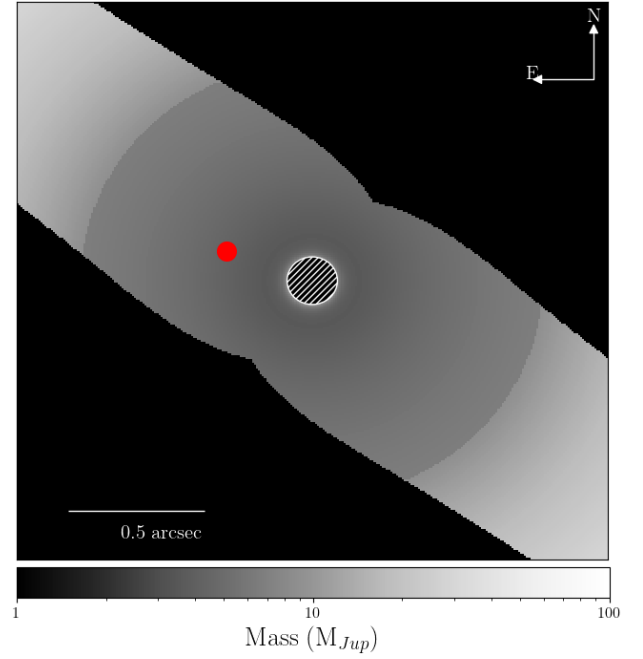
Fig. 3. 2D maps, obtained with FORECAST showing in grey the sky area compatible with the PMA reported in Table 1. The intensity of the grey areas changes according to the dynamical mass (in M_{\text{Jup}} ) responsible for the PMA at a given distance with the scale given by the lower color bar. The position of AF Lep b for the first SPHERE epoch is shown as a red circle. To avoid overlapping between the two positions we did not plot the position of the companion in the second epoch.
