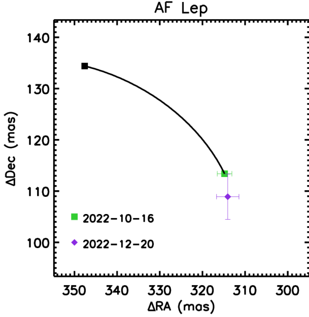
Fig. 2. Relative astrometry plot for the candidate companion of AF Lep. The green square represents the relative position of the companion at the first observing epoch while the violet diamond represents the relative position of the companion at the second epoch. The solid black line represents the expected motion relative to the host star of a background object while the black square is the expected position for a background object at the epoch of the second observation.
