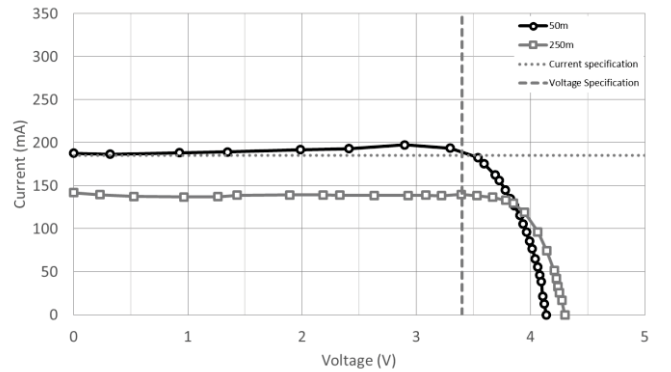
Figure 11. JDSU PPC-4E I-V curve versus fibre length.
