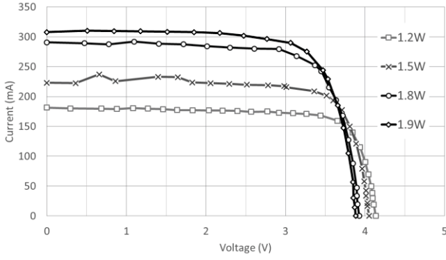
Figure 6. L2W OPI-4G I-V curves vs optical power.
