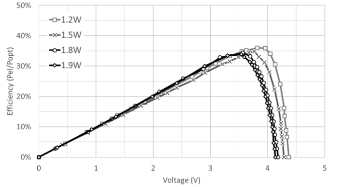
Figure 9. JDSU PPC-4E conversion efficiency vs optical power.
