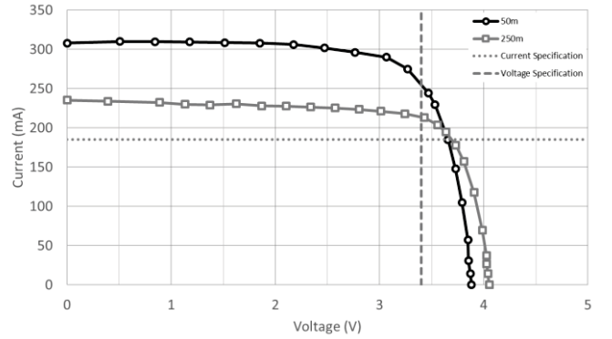
Figure 10. L2W OPI-4G I-V curve versus fibre length.
