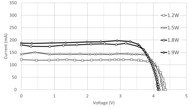
Figure 8. JDSU PPC-4E I-V curves vs optical power.
