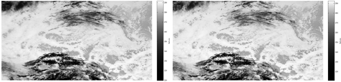
Figure 6: MSG stereo pair for band 10.8: MSG-2 image (left), and MSG-3 image (right)
