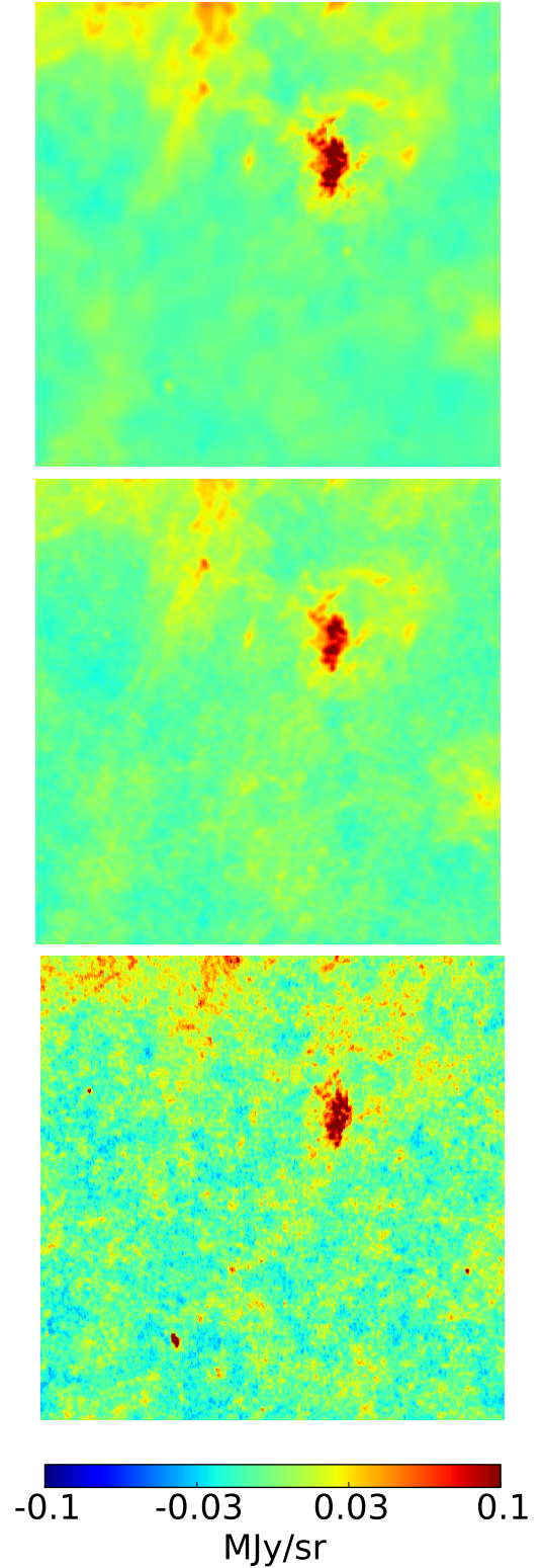
Fig. 7. 12.5 \times 12.5 gnomonic projection of dust intensity templates centred at high latitude (l, b) = (90^\circ, -80^\circ) at a map resolution of 5' . Top: new PSM dust from multi-dimensional GNILC ( Remazeilles et al. 2011 ). Middle: original PSM dust ( Delabrouille et al. 2013 ) based on the model of Finkbeiner et al. (1999) . Bottom: Planck 2013 dust model ( Planck Collaboration XI 2014 ). Comparing the top and bottom panels, the improvement in reducing the contamination of the dust by small-scale CIB anisotropies at high Galactic latitude is clearly visible.
