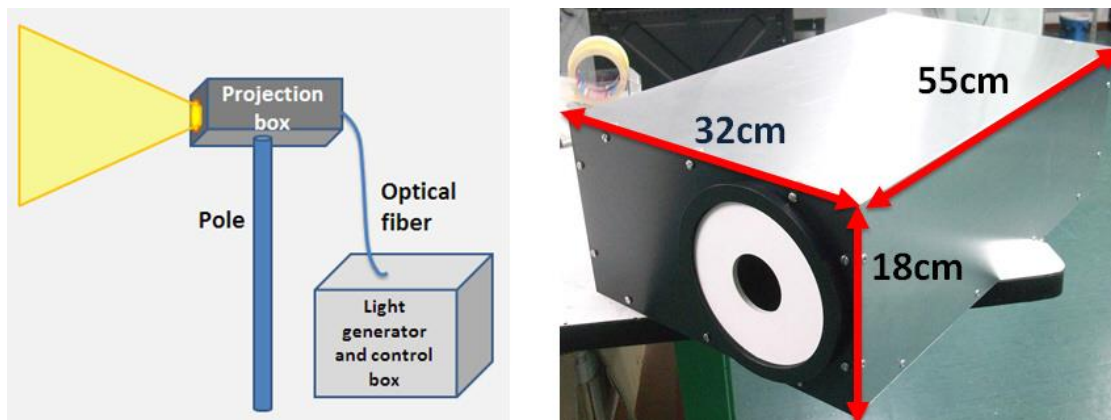
Figure 5. Illuminator. Basic design of the overall system (left) and aluminum case of the Projection Box (right).
