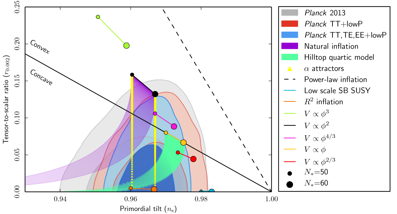
Fig. 12. Marginalized joint 68 % and 95 % CL regions for n_s and r at k = 0.002 \text{ Mpc}^{-1} from Planck compared to the theoretical predictions of selected inflationary models. Note that the marginalized joint 68 % and 95 % CL regions have been obtained by assuming dn_s/d \ln k = 0 .
