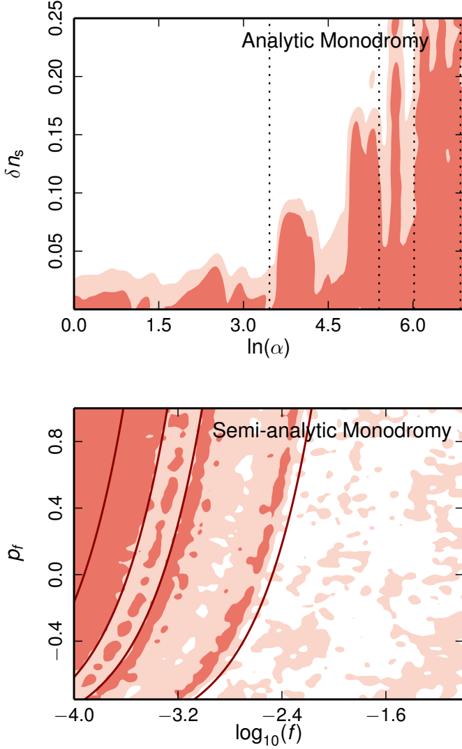
Fig. 41. Constraints on the parameters of the analytic (top) and semi-analytic (bottom) templates with EE -only high- \ell polarization data plus low- \ell temperature and polarization data, showing joint 68 % and 95 % CL. The lines mark the frequencies showing the highest-likelihood improvements identified in the baseline temperature-only analysis.
