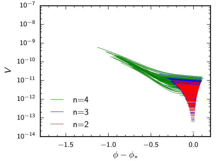
Fig. 15. Observable range of the best-fit inflaton potentials, when V(\phi) is Taylor expanded to the n th order around the pivot value \phi_* in natural units (where \sqrt{8\pi}M_{\text{pl}} = 1 ) assuming a flat prior on \epsilon_V , \eta_V , \xi_V^2 , and \omega_V^3 and using Planck TT+lowP+BAO. Potentials obtained under the transformation (\phi - \phi_*) \rightarrow (\phi_* - \phi) leave the same observable signature and are also allowed. The sparsity of potentials with a small V_0 = V(\phi_*) is due to our use of a flat prior on \epsilon_V rather than on \ln(V_0) ; in fact, V_0 is unbounded from below in the n = 2 and 3 results. The axis ranges are identical to those in Fig. 20, to make the comparison easier.
