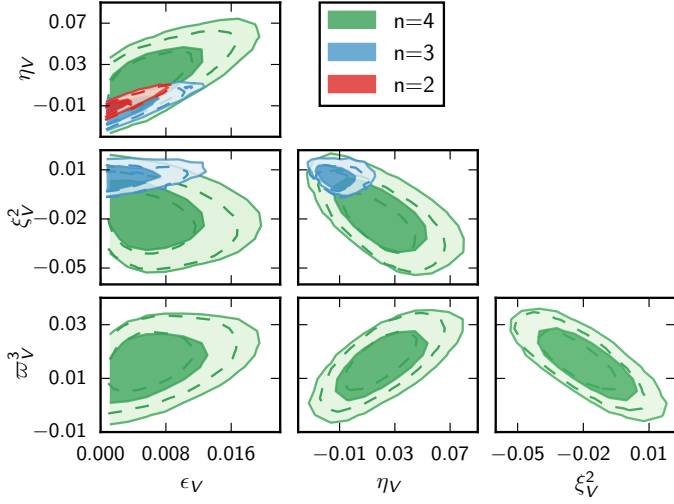
Fig. 13. Posterior distributions for the first four potential slow-roll parameters when the potential is Taylor expanded to n th order using Planck TT+lowP+BAO (filled contours) or TT,TE,EE+lowP (dashed contours). The primordial spectra are computed beyond the slow-roll approximation.
