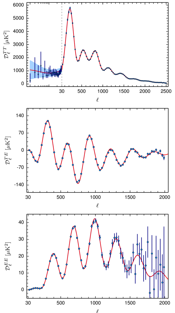
Fig. 2. Planck TT (top), high- \ell TE (centre), and high- \ell EE (bottom) angular power spectra. Here \mathcal{D}_\ell \equiv \ell(\ell + 1)C_\ell/(2\pi) .
