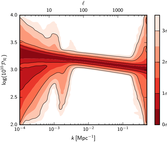
Fig. 26. Bayesian reconstruction of the primordial power spectrum averaged over different values of N_{\text{int}} (as shown in Fig. 24), weighted according to the Bayesian evidence. The region 30 < \ell < 2300 is highly constrained, but the resolution is lacking to say anything precise about higher \ell . At lower \ell , cosmic variance reduces our knowledge of \mathcal{P}_{\mathcal{R}}(k) . The weights assigned to the lower N_{\text{int}} models outweigh those of the higher models, so no oscillatory features are visible here.
