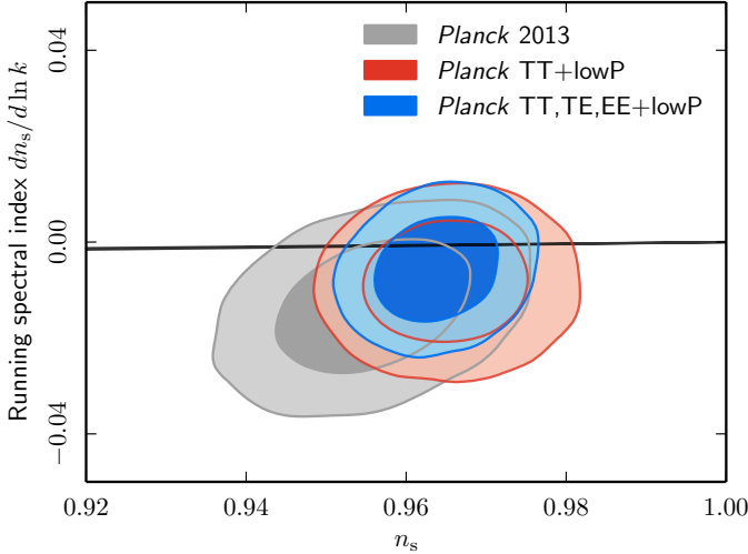
Fig. 4. Marginalized joint 68 % and 95 % CL for (n_s, dn_s/d \ln k) using Planck TT+lowP and Planck TT,TE,EE+lowP. Constraints from the Planck 2013 data release are also shown for comparison. For comparison, the thin black stripe shows the prediction for single-field monomial chaotic inflationary models with 50 < N_* < 60 .
