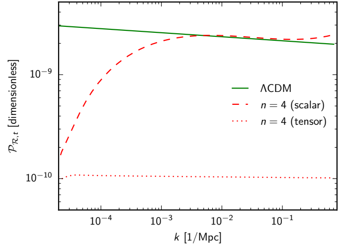
Fig. 17. Primordial spectra (scalar and tensor) of the best-fit V(\phi) model with n = 4 , for the Planck TT,TE,EE+lowP data set, compared to the primordial spectrum (scalar only) of the best-fit base \Lambda\text{CDM} model. The best-fit potential is initially very steep, as can be seen in Fig. 15 (note the typical shape of the green curves). The transition from “marginal slow roll” ( \epsilon_V(\phi) between 0.01 and 1) to “full slow roll” ( \epsilon_V(\phi) of order 0.01 or smaller) is responsible for the suppression of the large-scale scalar spectrum.
