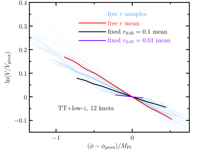
Fig. 32. Reconstructed single-field inflaton potentials from the cubic spline power spectra mode expansion using 12 knots.
