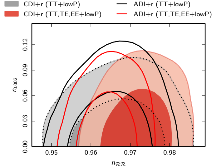
Fig. 50. 68 % and 95 % CL constraints on the primordial adiabatic spectral index n_{\text{RR}} and the primordial tensor-to-scalar ratio r (more accurately, in the CDI+r model, the primordial tensor-to-curvature power ratio) at k = 0.002 \text{ Mpc}^{-1} . Filled contours are for generally-correlated ADI+CDI and solid contours for the pure adiabatic model.
