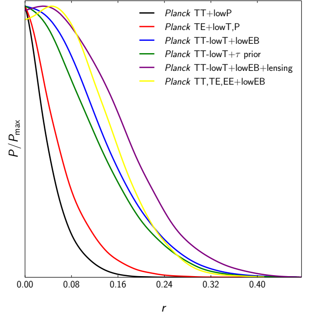
Fig. 8. One-dimensional posterior probabilities for r for various data combinations, either including or not including temperature multipoles for \ell < 30 , and compared with the baseline choice (Planck TT+lowP, black curve).
