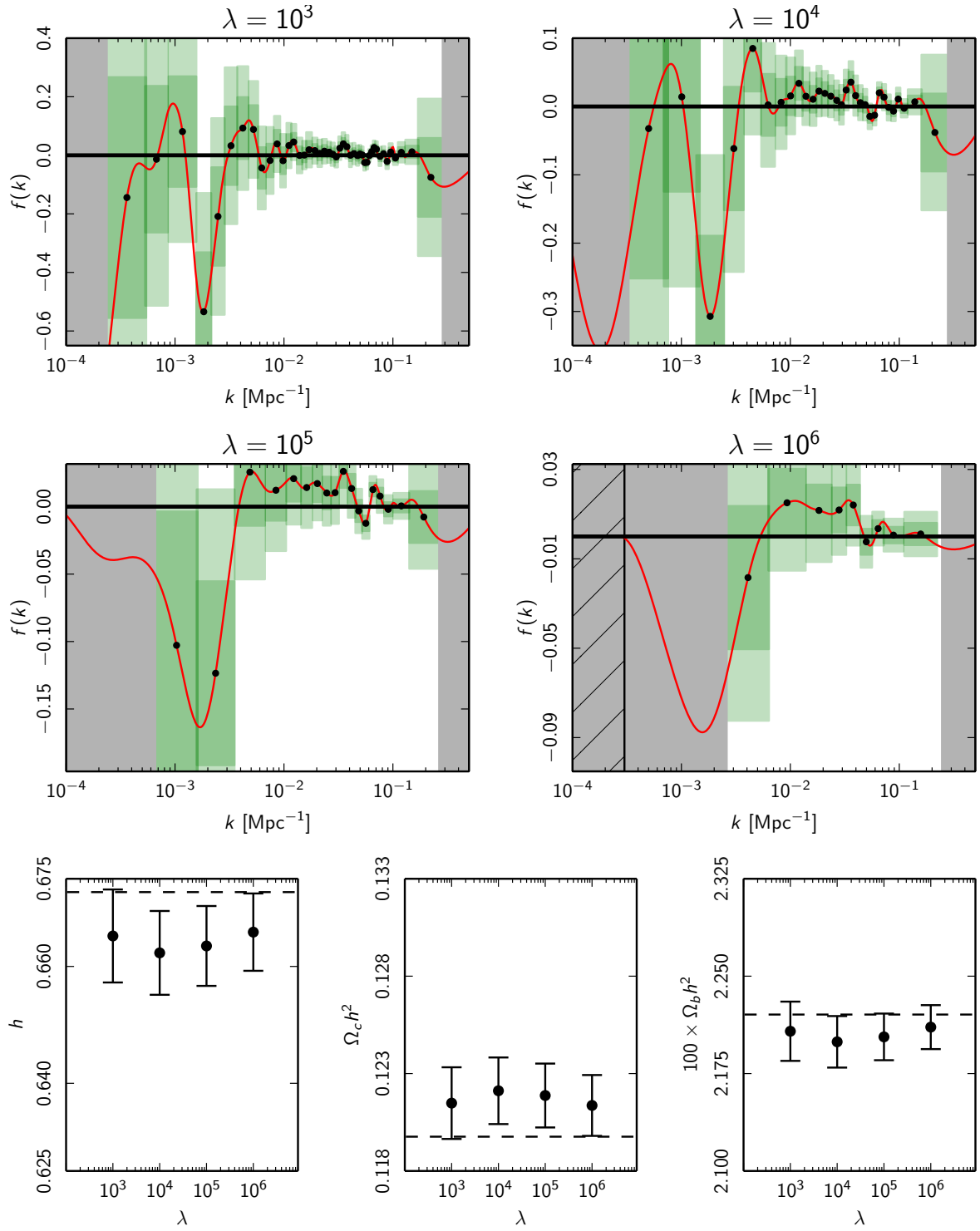
Fig. 22. Planck TT,TE,EE+lowP likelihood primordial power spectrum reconstruction results. Top four panels: Reconstruction of the deviation f(k) using four different roughness penalties. As in Fig. 21, the red curves represent the best-fit deviation f(k) and the height and width of the green error bars represent the error and minimum reconstructible width, respectively. For all values of the roughness penalty, the deviations are consistent with a featureless spectrum. Lower three panels: \pm 1\sigma error bars of the three non-PPS cosmological parameters included in the maximum likelihood reconstruction. All values are consistent with their respective best-fit fiducial model values (indicated by the dashed lines).
