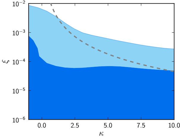
Fig. 54. 68 % and 95 % CL regions in the modulated isocurvature model parameter space using the Planck temperature data up to \ell_{\text{max}} = 1000 (contours). The region above the dashed curve is ruled out by the Planck constraint on an uncorrelated, scale-invariant isocurvature component.
