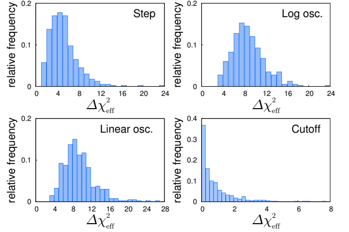
Fig. 34. Distribution of \Delta\chi^2 from 400 simulated Planck TT+lowP data sets.
