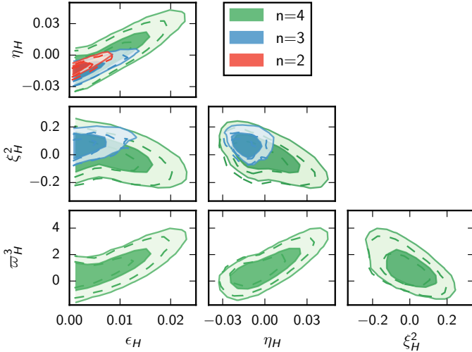
Fig. 19. Posterior distributions for the first four Hubble slow-roll parameters, when H(\phi) is Taylor expanded to n th order, using Planck TT+lowP+BAO (filled contours) or TT,TE,EE+lowP (dashed contours). The primordial spectra are computed beyond the slow-roll approximation.
