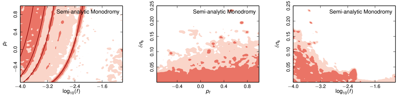
Fig. 38. Constraints on the parameters of the semi-analytic template showing joint 68 % and 95 % CL. The solid lines on the left-hand panel mark the frequencies showing the highest-likelihood improvements (see text).
