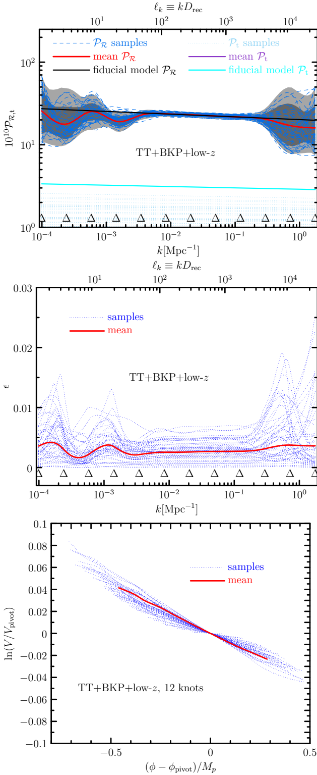
Fig. 56. Impact of BKP likelihood on scalar primordial power spectrum reconstruction. We show how including the BKP likelihood affects the reconstruction in Sect. 8.3. The top panel is to be compared with the reconstructions in Fig. 27, and we observe that including BKP has a minimal impact given the uncertainty in the reconstruction. The middle panel is to be compared with Fig. 31, and here we notice that including BKP excludes the trajectories with large values of \epsilon . The bottom panel shows how the inflationary potential reconstructions are modified by BKP (to be compared with Fig. 32).
