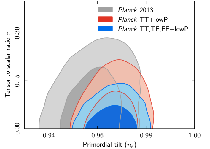
Fig. 6. Marginalized joint confidence contours for (n_s, r) , at the 68 % and 95 % CL, in the presence of running of the spectral indices, and for the same data combinations as in the previous figure.
