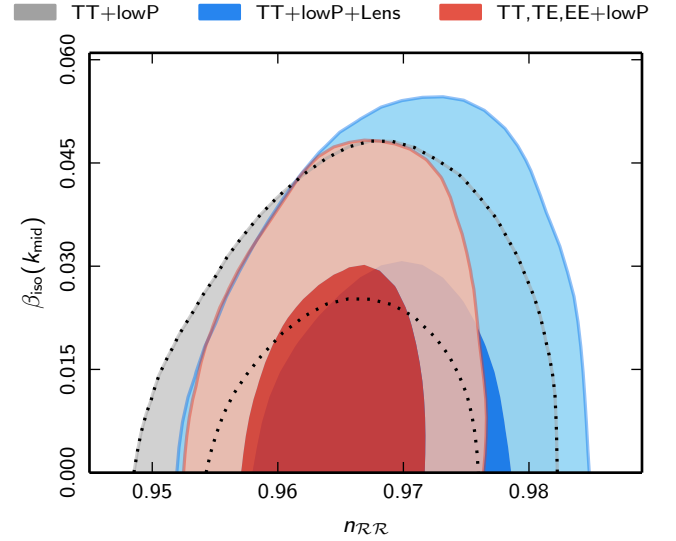
Fig. 51. Uncorrelated ADI+CDI with n_{\text{II}} = 1 (“axion”).
