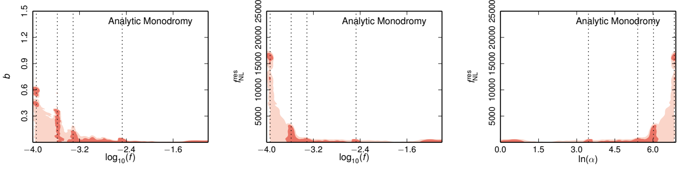
Fig. 42. Derived constraints on the parameters of the potential, Eq. (109), as well as the predicted resonant NG, f_{\text{NL}}^{\text{res}} , using the analytic template, showing joint 68 % and 95 % CL. The dotted lines mark the frequencies showing the highest-likelihood improvements (see text).
