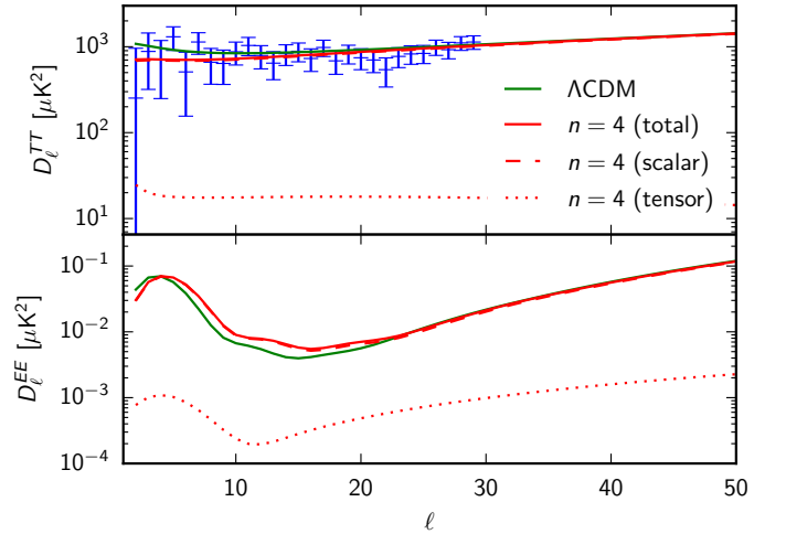
Fig. 18. Temperature and polarization spectra (total, scalar contribution, tensor contribution) of the best-fit V(\phi) model with n = 4 , for the Planck TT,TE,EE+lowP data set, compared to the spectra (scalar contribution only) of the best-fit base model. We also show the Planck low- \ell temperature data, which is driving the small differences between the two best-fit models.
