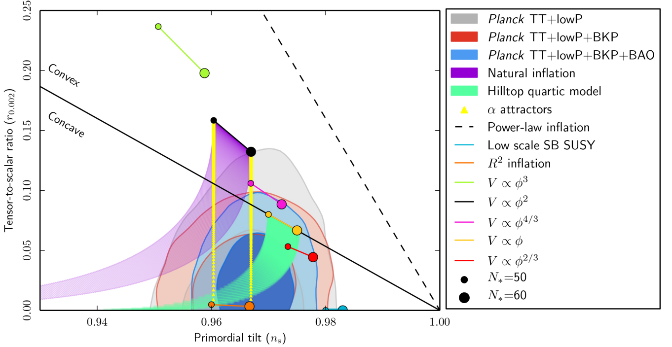
Fig. 55. Marginalized joint 68 % and 95 % CL regions for n_s and r at k = 0.002 \text{ Mpc}^{-1} from Planck alone and in combination with its cross-correlation with BICEP2/Keck Array and/or BAO data compared with the theoretical predictions of selected inflationary models. Note that the marginalized joint 68 % and 95 % CL regions have been obtained by assuming dn_s/d \ln k = 0 .
