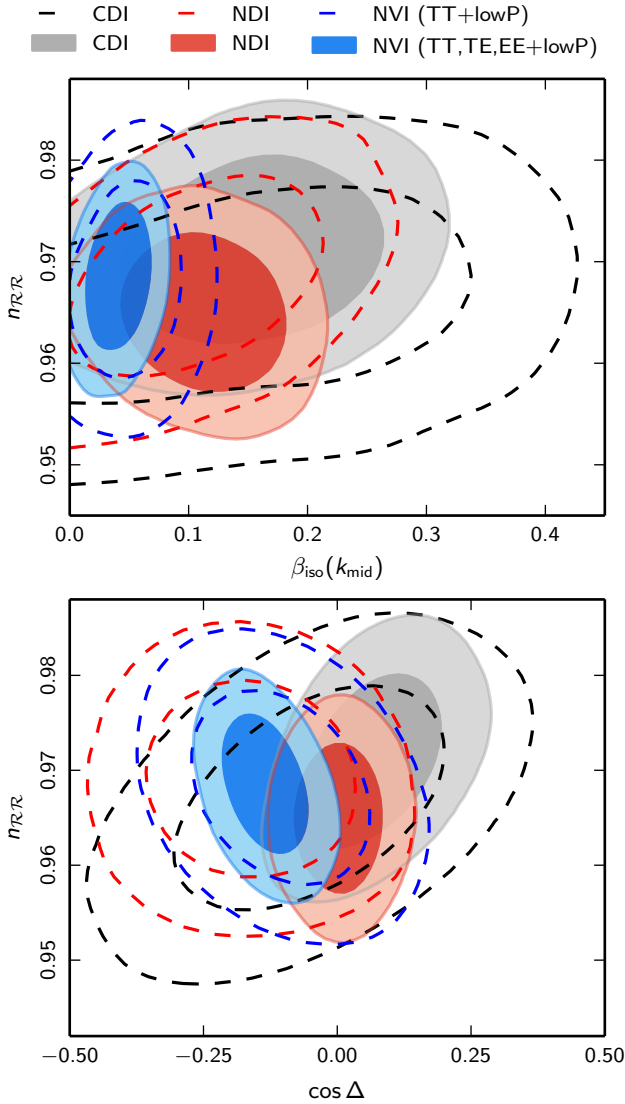
Fig. 49. Dependence of the determination of the adiabatic spectral index n_{RR} (called n_s in the other sections of this paper) on the primordial isocurvature fraction \beta_{iso} and correlation fraction \cos \Delta , with Planck TT+lowP data (dashed contours) and with Planck TT,TE,EE+lowP data (shaded regions).
