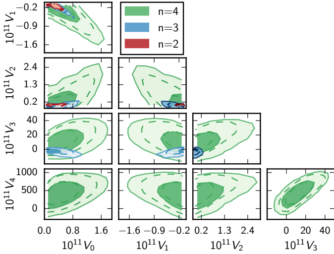
Fig. 14. Posterior distributions for the coefficients of the inflation potential Taylor expanded to n th order (in natural units where \sqrt{8\pi}M_{\text{pl}} = 1 ) reconstructed beyond the slow-roll approximation using Planck TT+lowP+BAO (filled contours) or TT,TE,EE+lowP (dashed contours). The plot shows only half of the results; the other half is symmetric, with opposite signs for V_\phi and V_{\phi\phi\phi} . Note that, unlike Fig. 13, the parameters shown here do not have flat priors, since they are mapped from the slow-roll parameters.
