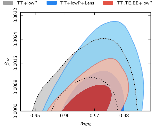
Fig. 52. Fully correlated ADI+CDI with n_{II} = n_{\mathcal{RR}} (“curvaton I”). Since the spectral indices are equal, the primordial isocurvature fraction \beta_{\text{iso}} is scale independent.
