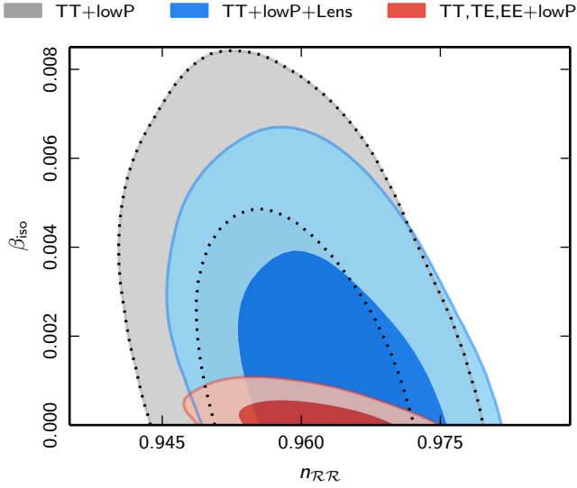
Fig. 53. Fully anticorrelated ADI+CDI with n_{II} = n_{RR} (“curvaton II”).
