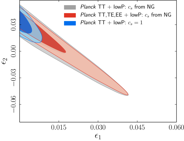
Fig. 35. (\epsilon_1, \epsilon_2) 68 % and 95 % CL constraints for Planck data comparing the canonical Lagrangian case with c_s = 1 to the case of varying c_s with a uniform prior 0.024 < c_s < 1 derived from the Planck NG measurements.
