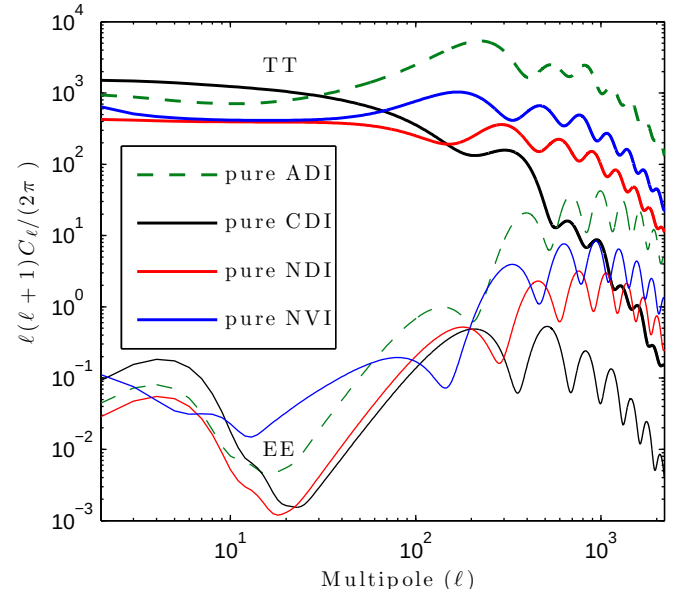
Fig. 43. Angular power spectra for the scale-invariant (i.e., n_{\text{RR}} = 1 ) pure adiabatic mode (ADI, green dashed curves) and for the scale invariant ( n_{\text{II}} = 1 ) pure isocurvature (CDI, NDI, or NVI) modes, with equal primordial perturbation amplitudes. The thick lines represent the temperature auto-correlation (TT) and the thin lines the E -mode polarization auto-correlation (EE).
