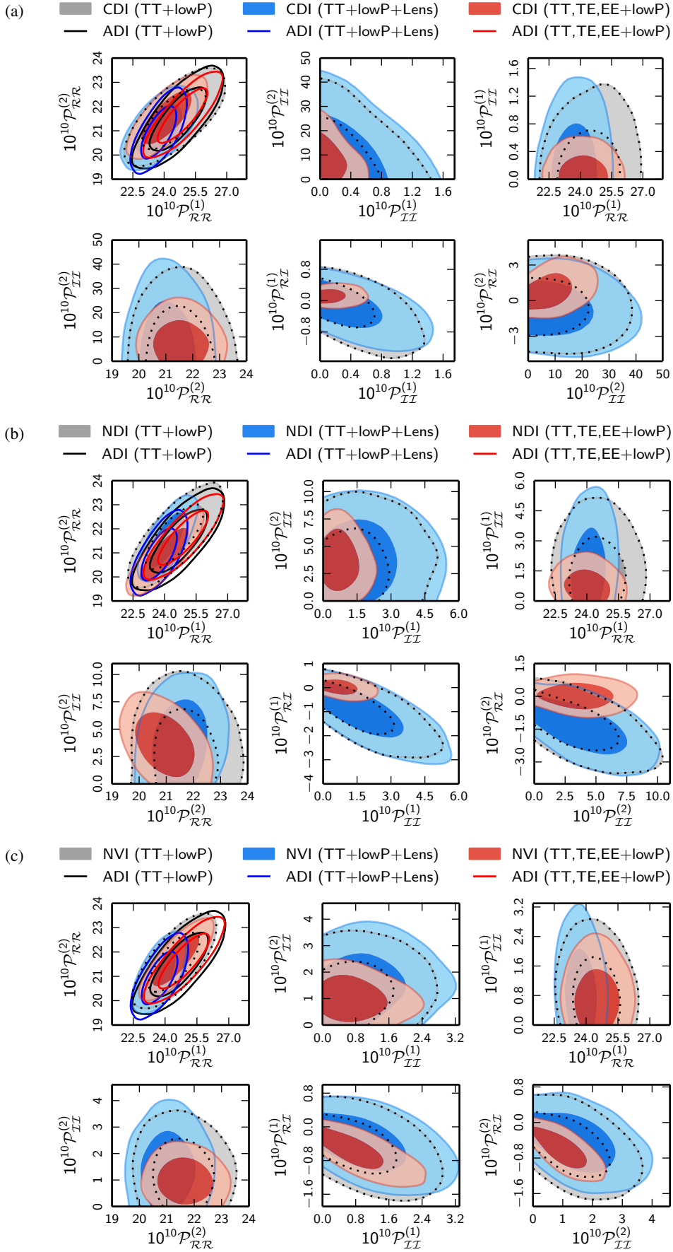
Fig. 44. 68 % and 95 % CL constraints on the primordial perturbation power in general mixed ADI+CDI (a), ADI+NDI (b), and ADI+NVI (c) models at two scales, k_1 = 0.002 \text{ Mpc}^{-1} (1) and k_2 = 0.100 \text{ Mpc}^{-1} (2), for Planck TT+lowP (grey regions highlighted by dotted contours), Planck TT+lowP+lensing (blue), and Planck TT,TE,EE+lowP (red). In the first panels, we also show contours for the pure adiabatic base \Lambda CDM model with the corresponding colours of solid lines.
