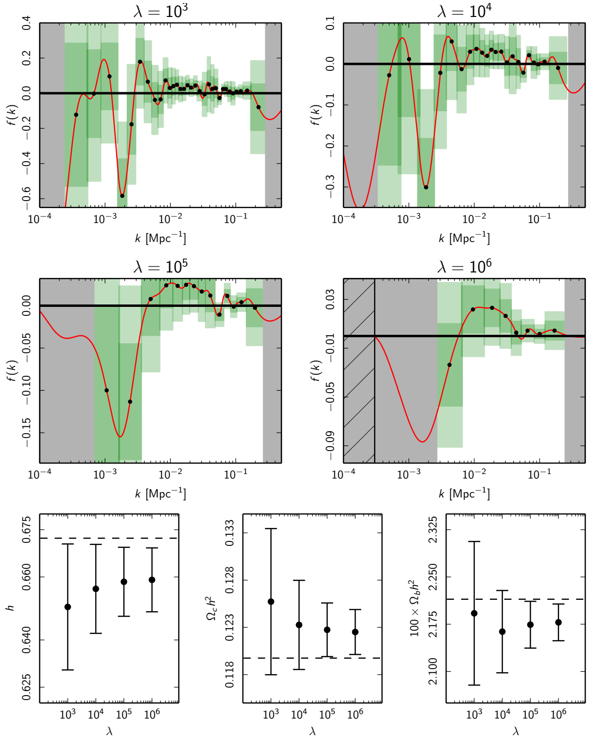
Fig. 21. Planck TT+lowP likelihood primordial power spectrum (PPS) reconstruction results. Top four panels: Reconstruction of the deviation f(k) using four different roughness penalties. The red curves represent the best-fit deviation f(k) using the Planck TT+lowP likelihood. f(k) = 0 would represent a perfectly featureless spectrum with respect to the fiducial PPS model, which is obtained from the best-fit base \Lambda CDM model with a power-law PPS. The vertical extent of the dark and light green error bars indicates the \pm 1\sigma and \pm 2\sigma errors, respectively. The width of the error bars represents the minimum reconstructible width (the minimum width for a Gaussian feature so that the mean square deviation of the reconstruction is less than 10 %). The grey regions indicate where the minimum reconstructible width is undefined, indicating that the reconstruction in these regions is untrustworthy. The hatched region in the \lambda = 10^6 plot shows where the fixing penalty has been applied. These hashed regions are not visible in the other three reconstructions, for which \kappa_{\min} lies outside the range shown in the plots. For all values of the roughness penalty, all data points are within 2\sigma of the fiducial PPS except for the deviations around k \approx 0.002 Mpc ^{-1} in the \lambda = 10^3 and \lambda = 10^4 reconstructions. Lower three panels: \pm 1\sigma error bars of the three non-PPS cosmological parameters included in the maximum likelihood reconstruction. All values are consistent with their respective best-fit fiducial model values indicated by the dashed lines.
