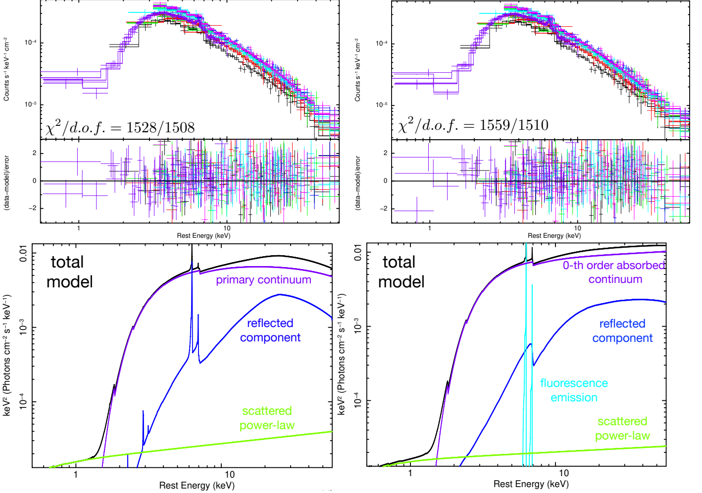
Fig. 10. Left Panels: XMM-Newton / Swift / NuSTAR data best-fit using xillver (top). The different spectral components are reported in the corresponding bottom graph. Right panels: XMM-Newton / Swift / NuSTAR data best-fit (top) and model components (bottom) corresponding to the decoupled MyTorus solution.
