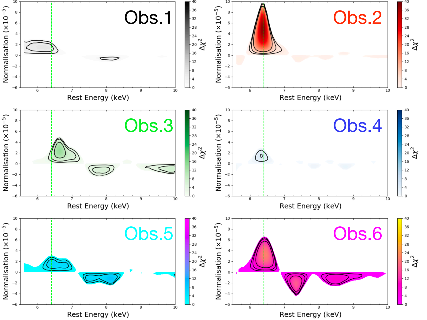
Fig. 6. Result of a blind line scan performed to all six NuSTAR observations plotted between the 5.5 – 10 keV band. The colour bar on the right of each panel indicates the significance of the lines for 2 degree of freedom and the solid black contours correspond to 68%, 90% and 99%. The lime-green vertical dashed line indicates the position of the rest frame energy of the Fe K\alpha emission line at E = 6.4 \text{ keV}
