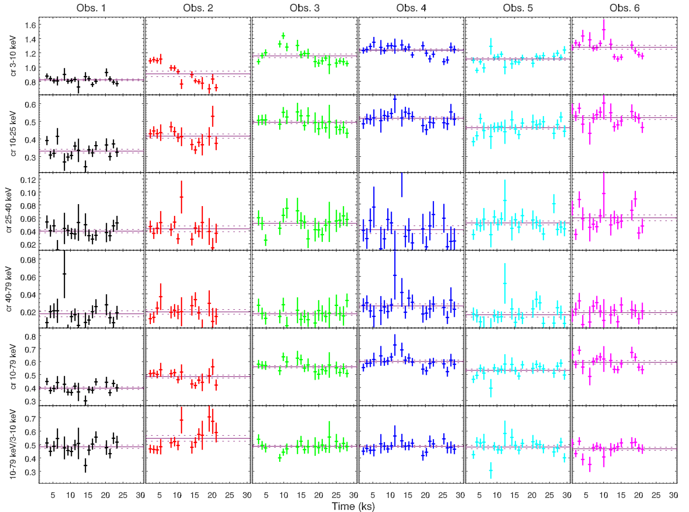
Fig. 2. Background subtracted NuSTAR light curves of MCG-01-24-12 calculated with a temporal bin of 1000 sec. Light curves account for co-added module A and B and the various energy bands are labelled on the y-axis. For each observation a specific colour is used and we adopted such a colour code throughout the whole paper. Orchid horizontal straight lines are used to quantify the average count rate within each observation for the different bands, while dashed ones account for 1\sigma uncertainties around the mean.
