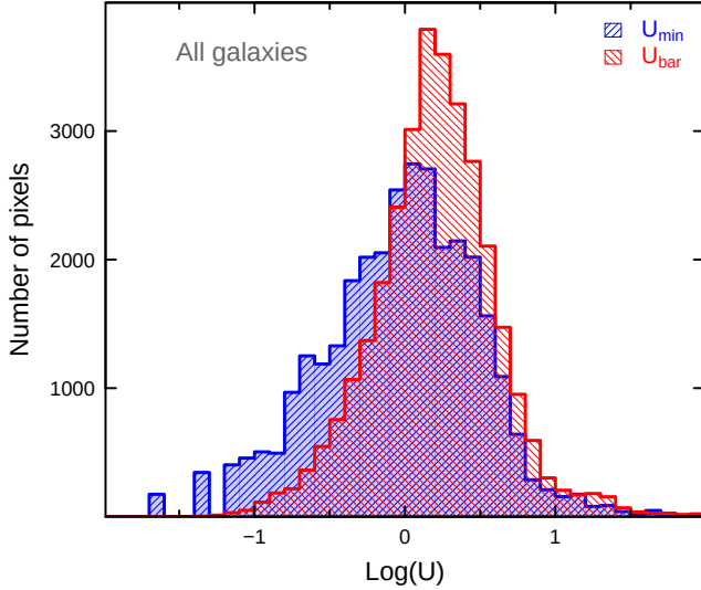
Figure 9. Distributions of U_{\min} and \bar{U} ( U_{\text{bar}} ) for all galaxies. U_{\min} and \bar{U} are the renormalized values (see Eq. 13-16). Both distributions are fairly broad; for a given pixel, \bar{U} - U_{\min} may be smaller than or comparable to U_{\min} given that f_{\text{PDR}} is usually modest. Thus, it is not surprising that the two peaks are similar.
