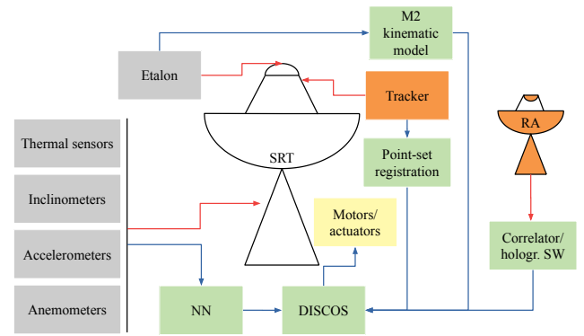
Figure 1. Architecture of the new Sardinia Radio Telescope's metrology system (SMS): In grey are shown the devices used to study pointing effects; in orange is shown the equipment installed to monitor the accuracy of the main reflector. Green are used to identify computer hardware and software dedicated to the management of data collected by the measuring devices. Yellow indicates mechanical drives. In addition, red arrows indicate the active monitoring of the structure, while blue is used to indicate the transmission of collected data to the dedicated management systems.
