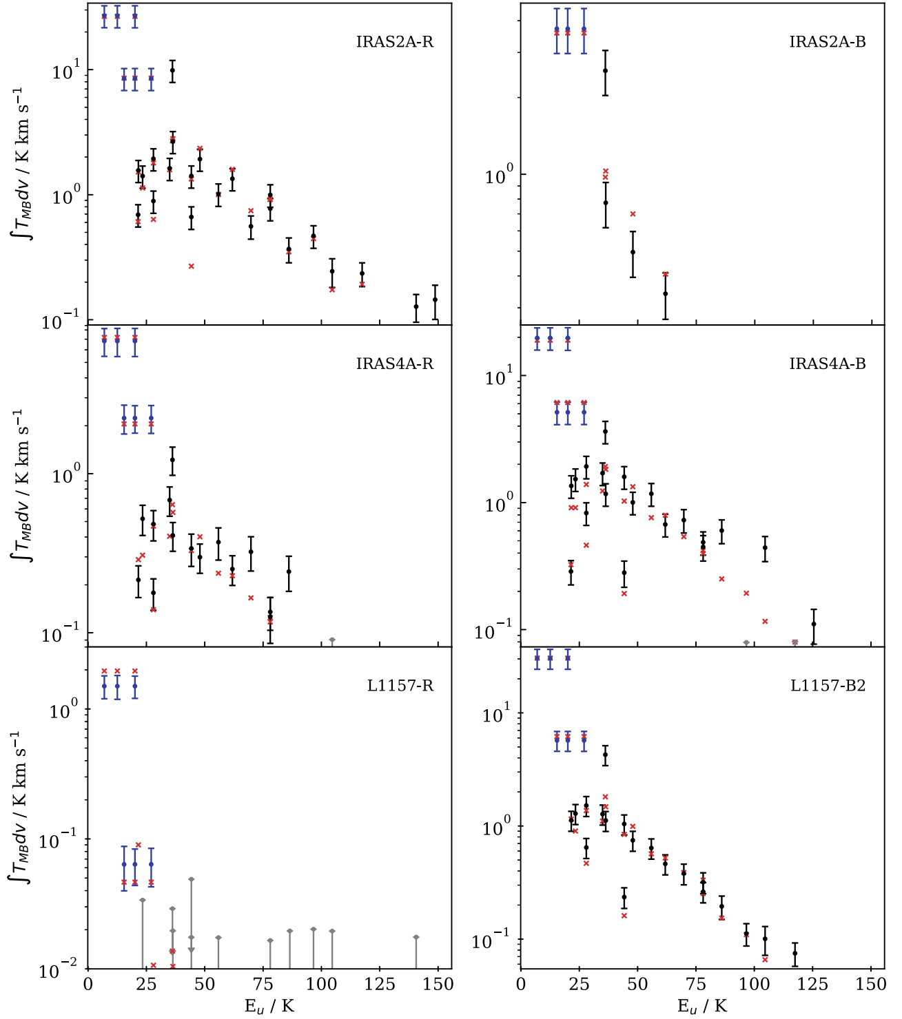
Figure 1. Measured flux (black points and error bars) of \text{CH}_3\text{OH} transitions plotted against E_u . The blue points are those transitions that are blended, and the total emission across all three transitions is plotted in each case along with the sum of the RADEX model emission. The gray upper limits show undetected transitions. The red crosses indicate the fluxes produced by RADEX for the most likely parameter values.
