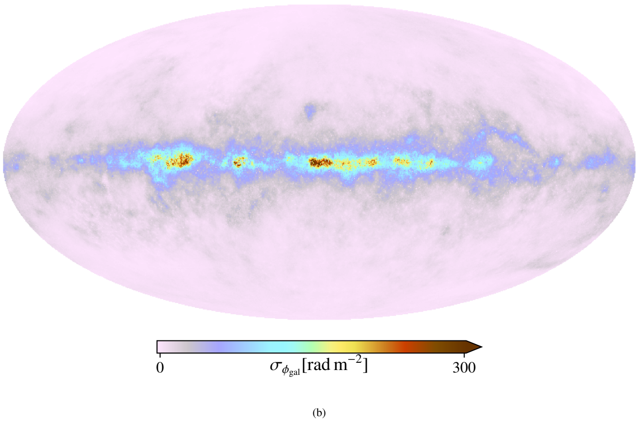
Fig. 3: As for Fig. 2, but the color scale is saturated at \pm 1500 \text{ rad m}^{-2} in the mean and 300 \text{ rad m}^{-2} in the uncertainty to highlight disc features of the Galactic Faraday rotation sky.
