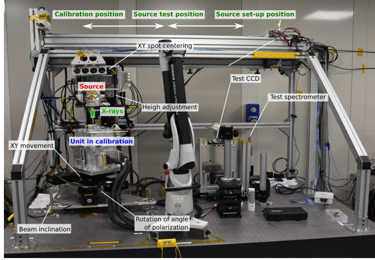
Figure 11. The instrument calibration equipment at INAF-IAPS . On the left a flight DU under calibration with a polarized source. At the center the Romer arm used for metrology is visible. On the right the CCD to study the beam image and the SDD to study the beam spectrum are just visible.
