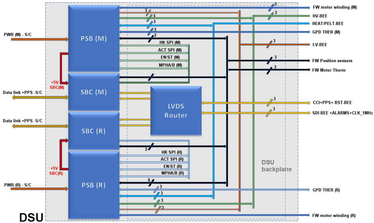
Figure 8. DSU high level architecture.
