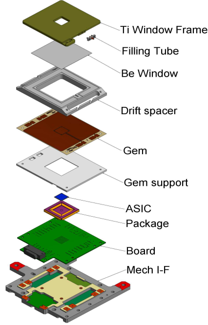
Figure 4. Schematic representation of GPD assembly.
