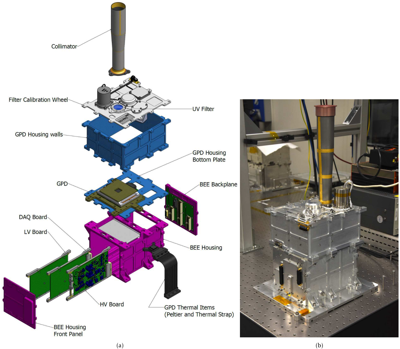
Figure 3. The IXPE Detector Units (a) Exploded view of a Detector Unit, (b) Photograph of a Flight Detector Unit in its handling plane. The thermal environment is controlled by means of a Peltier cooler and a heater. A thermal strap conducts the heat from the GPD Peltier/heater system to the radiator of the spacecraft.
