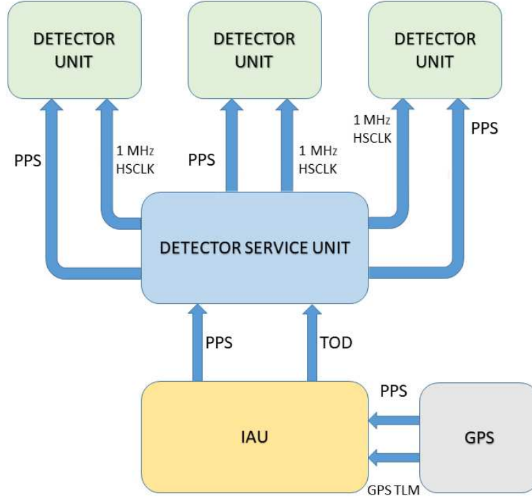
Figure 9. The Architecture of timing for the instrument.
