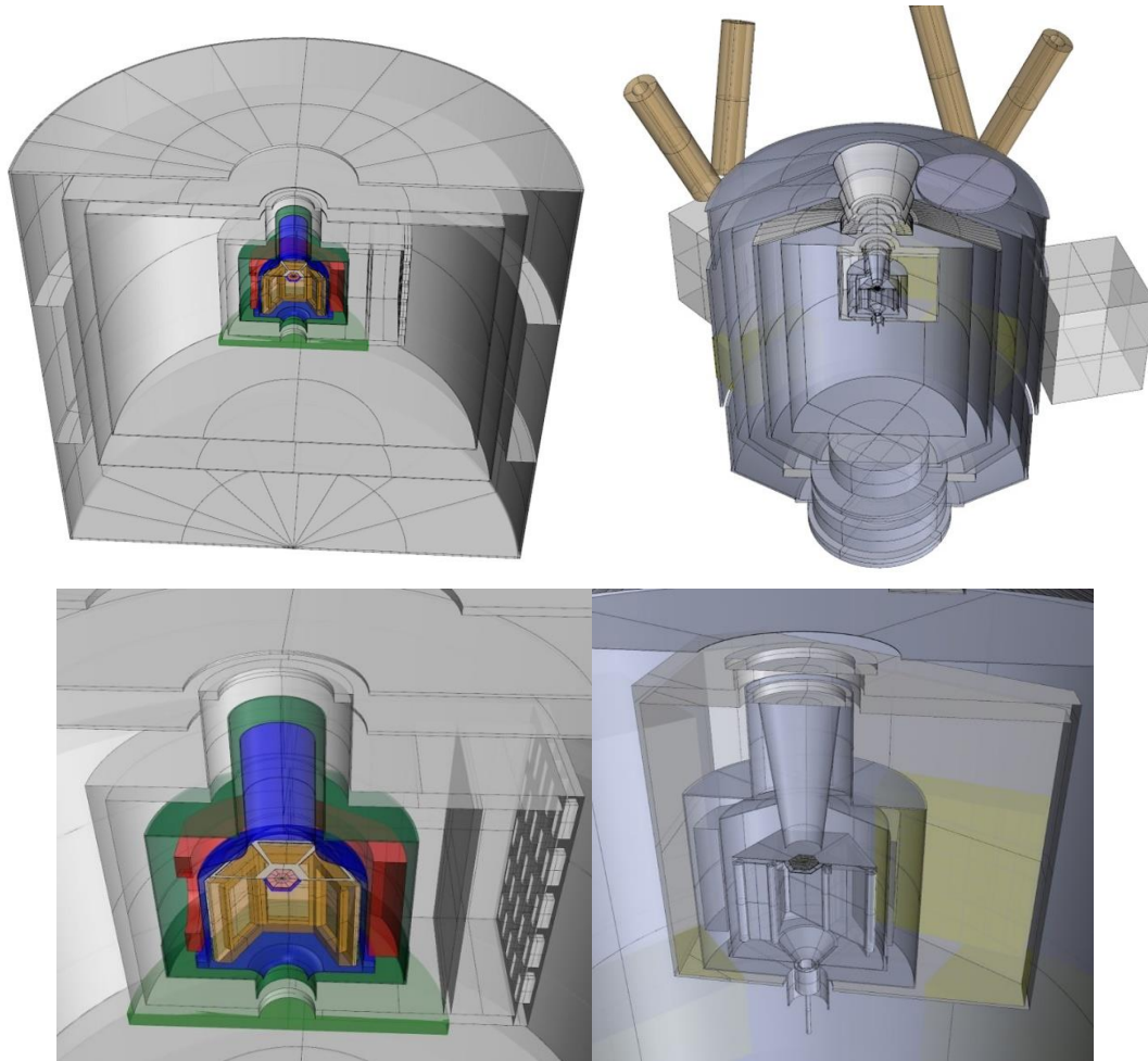
Figure 5 - The old and new cryostat mass models (top left and right, respectively) and FPA (bottom left and right).
