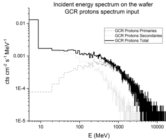
Figure 17. Spectra of incident energies of the particles impacting the silicon wafer supporting the main detector array (GCR protons only).
