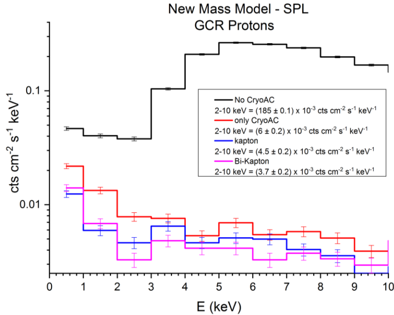
Figure 4 – background levels in different FPA configurations.
