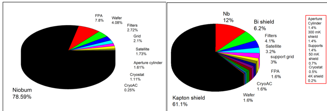
Figure 7 - The residual background origin without passive shielding (left), and after the insertion of the Kapton/Bi shield (right).
