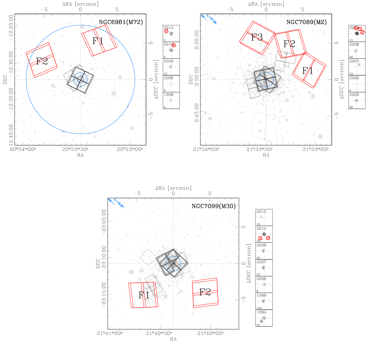
Figure A8. As in Fig. 1 but for NGC 6981, NGC 7089, and NGC 7099.
