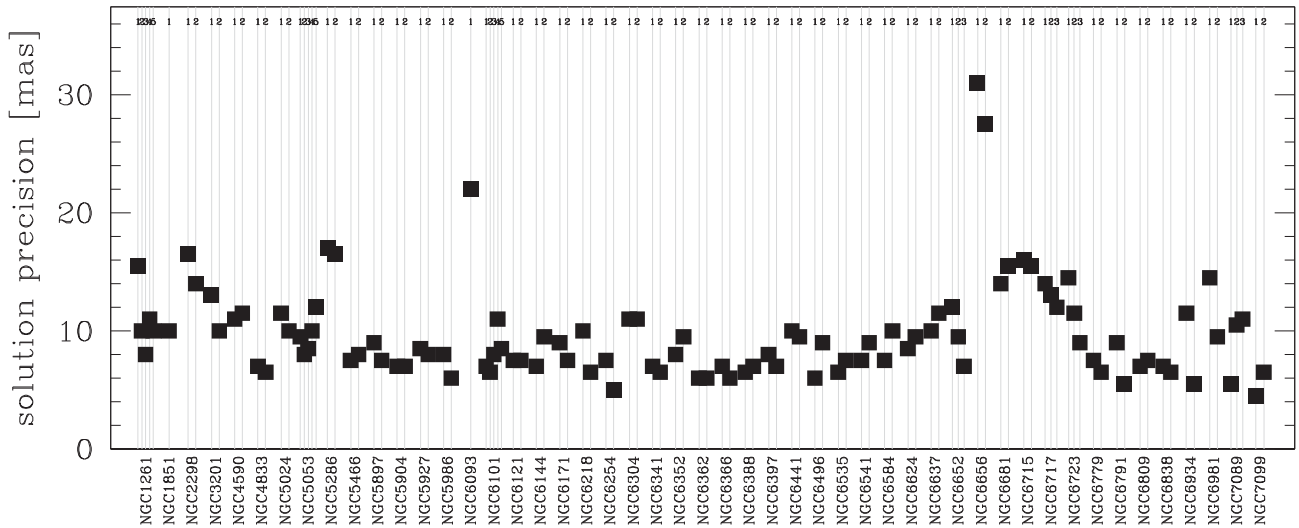
Figure 3. Precision of the redefined astrometric solution for each observed field, see the text for details.
