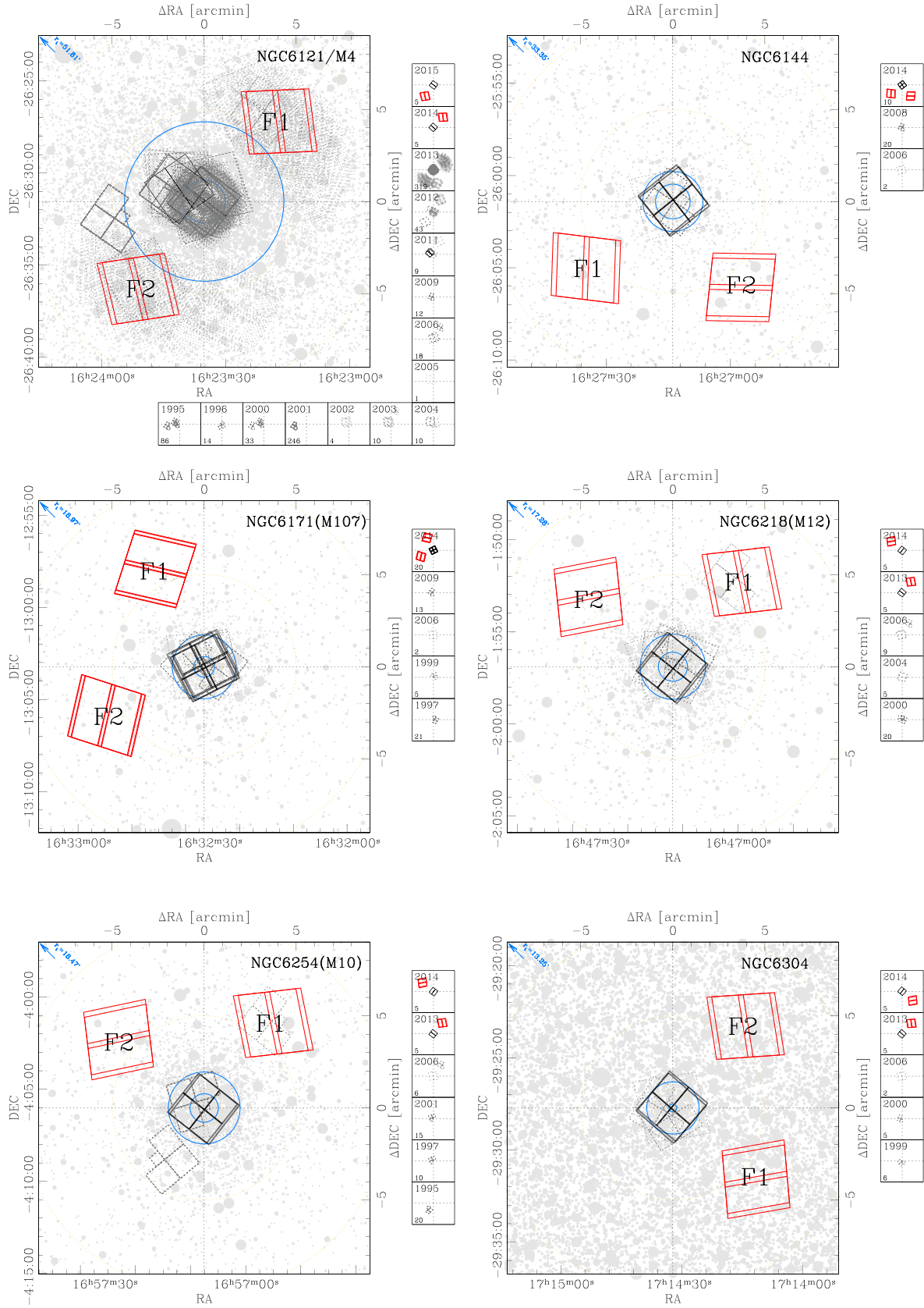
Figure A3. As in Fig. 1 but for NGC 6121, NGC 6144, NGC 6171, NGC 6218, NGC 6254, and NGC 6304.
