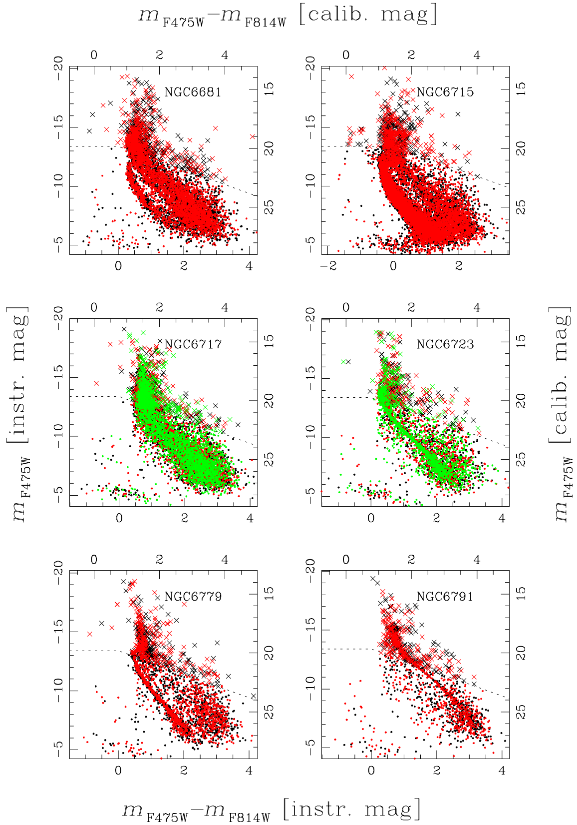
Figure A15. As in Fig. A9 but for NGC 6681, NGC 6715, NGC 6717, NGC 6723, NGC 6779 and NGC 6791.
