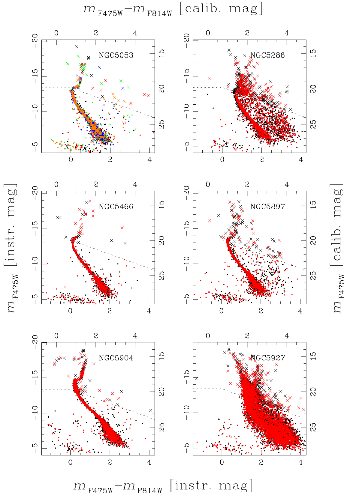
Figure A10. As in Fig. A9 but for NGC 5053, NGC 5286, NGC 5466, NGC 5897, NGC 5904, and NGC 5927.
