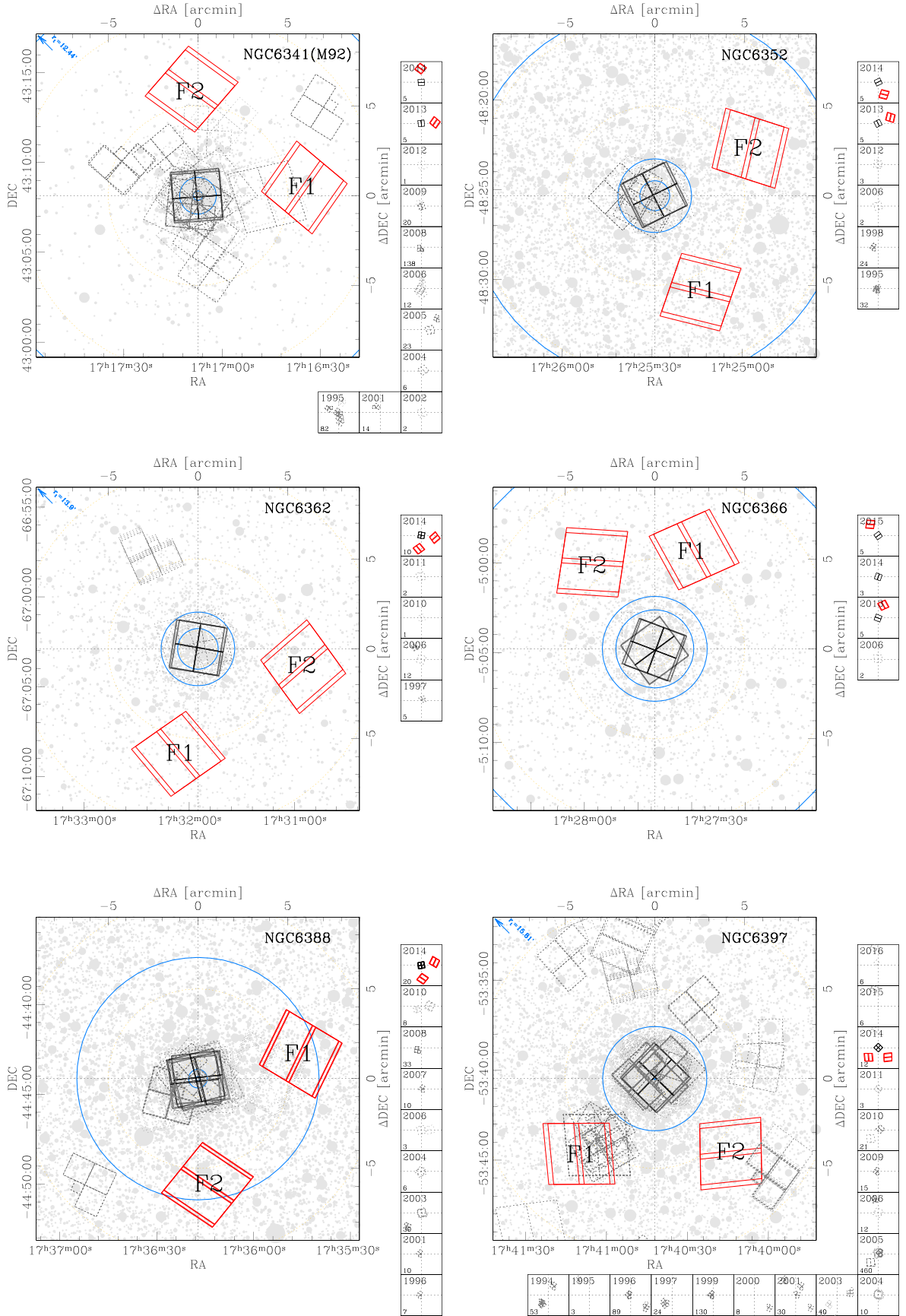
Figure A4. As in Fig. 1 but for NGC 6341, NGC 6352, NGC 6362, NGC 6366, NGC 6388, and NGC 6397.
