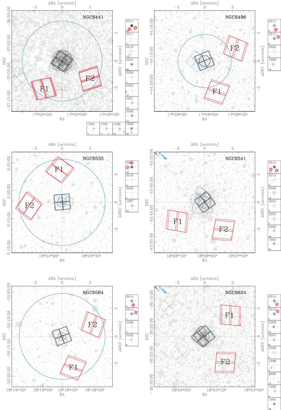
Figure A5. As in Fig. 1 but for NGC 6441, NGC 6496, NGC 6535, NGC 6541, NGC 6584, and NGC 6624.
