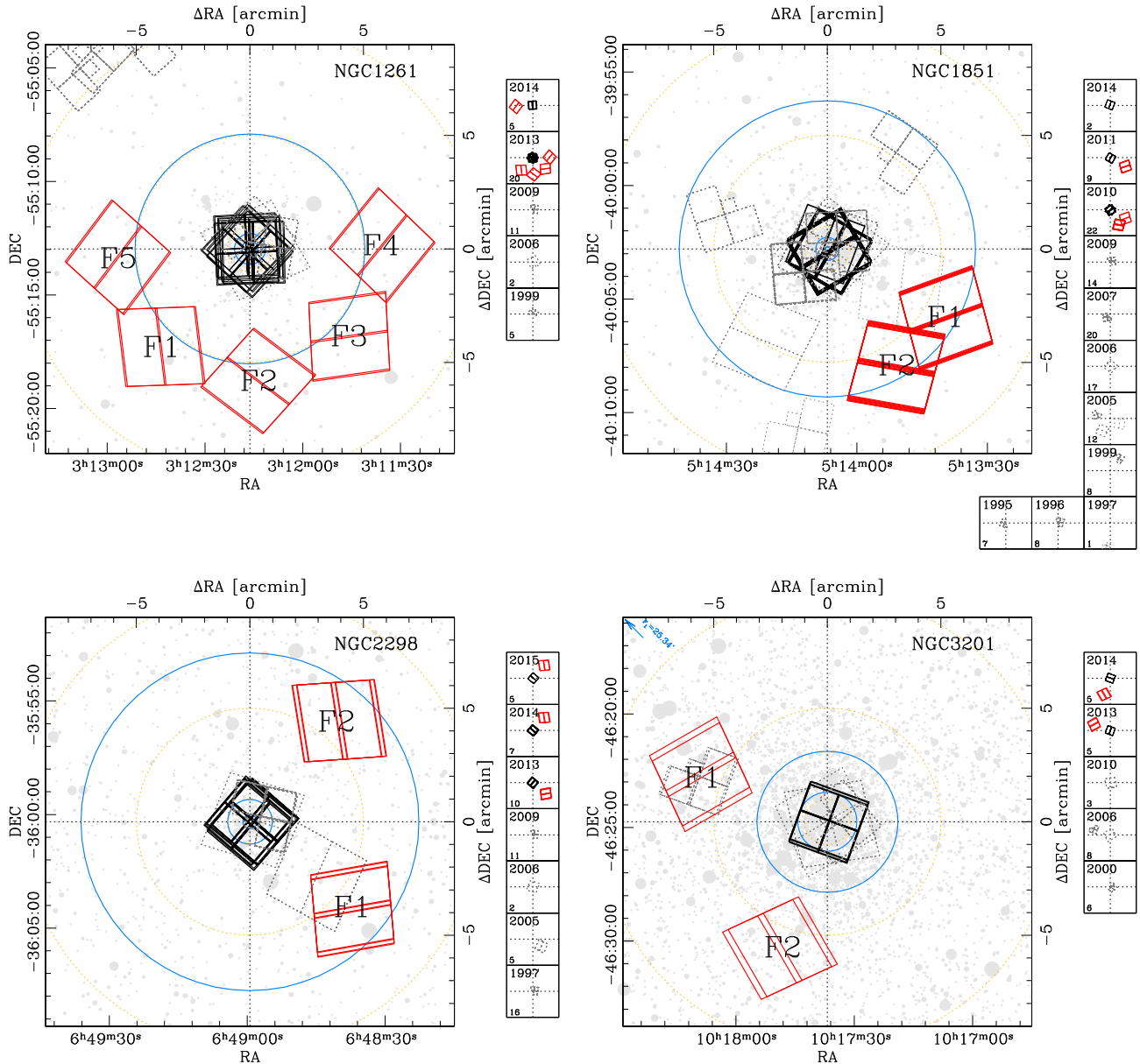
Figure 1. Finding charts for NGC 1261, NGC 1851, NGC 2298, and NGC 3201. Red outlines represent ACS/WFC parallel observations of GO-13297, black outlines refer to WFC3/UVIS observations. Dark grey, dashed outlines represent archive HST observations in the same regions. Footprints are labeled as in Table 1. Observations are subdivided by epoch in the smaller panels. Blue circles mark the position of core radius, half-light radius, and tidal radius for each cluster from Harris 1996 (2010). Where the tidal radius could not be included in the image, its value has been indicated in the upper-left corner of the image. Yellow, dashed circles mark the distances of 1, 5, and 10 arcmin from cluster centres. Grey dots corresponds to 2MASS sources, with brighter sources being larger.
