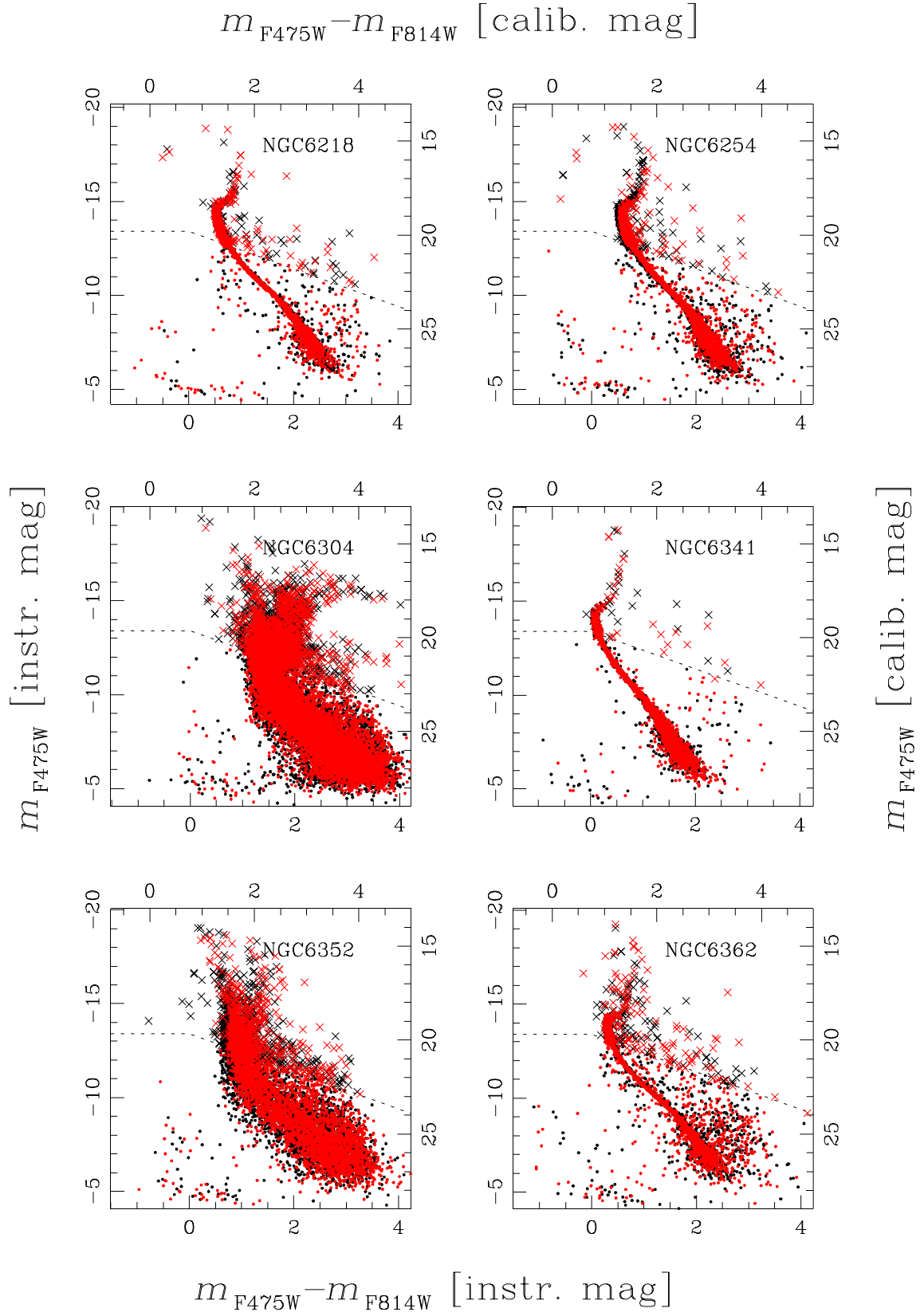
Figure A12. As in Fig. A9 but for NGC 6218, NGC 6254, NGC 6304, NGC 6341, NGC 6352, and NGC 6362.
