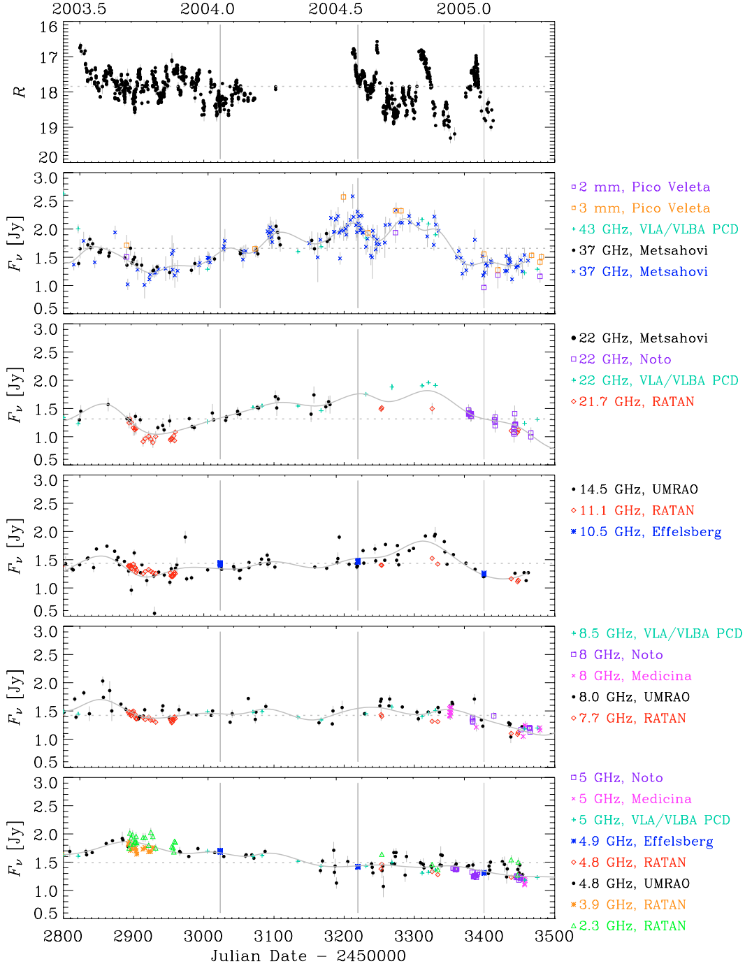
Fig. 3. R -band magnitudes ( top ) and radio fluxes (Jy) at different frequencies during the 2003–2005 WEBT campaign. Vertical lines mark the times of the three XMM-Newton pointings. Cubic splines on the radio data at 37, 22, 14.5, 8, and 5 GHz are plotted to better see the long-term trend. Horizontal lines indicate the mean fluxes at these frequencies. Two different symbols are used for the 37 GHz data from Metsähovi since they come from different datasets.
