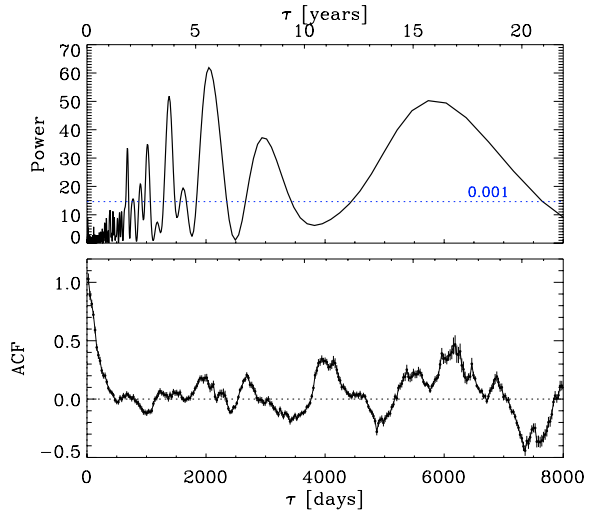
Fig. 9. Power spectrum of the discrete Fourier transform ( top ) and auto-correlation function ( bottom ) obtained from the historical 8 GHz light curve. In the top panel the blue dotted line indicates the level above which the significance is better than 0.001.
