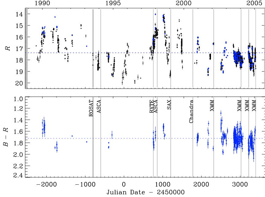
Fig. 4. B - R colour indices ( bottom ) compared to the R -band light curve ( top ); in the top panel blue (larger) dots indicate the R data used to derive the colour indices. Horizontal lines are drawn through average values; vertical lines indicate the times of the X-ray satellite pointings, discussed in Sect. 5.
