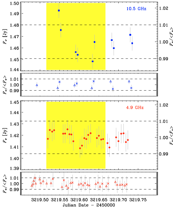
Fig. 5. Radio light curves of the source and calibrators at 10.5 GHz ( top , blue symbols) and 4.9 GHz ( bottom , red symbols) obtained with the 100 m radio telescope at Effelsberg on August 2, 2004. The two calibrators are 3C 067 (triangles) and 4C +09.11 (crosses). The horizontal lines indicate deviations of 1% from the mean flux densities, while the yellow areas highlight the period of the X-ray observations.
