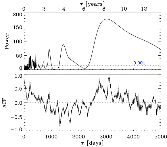
Fig. 8. Power spectrum of the discrete Fourier transform ( top ) and auto-correlation function ( bottom ) obtained from the historical R -band light curve. In the top panel the blue dotted line indicates the level above which the significance is better than 0.001.
