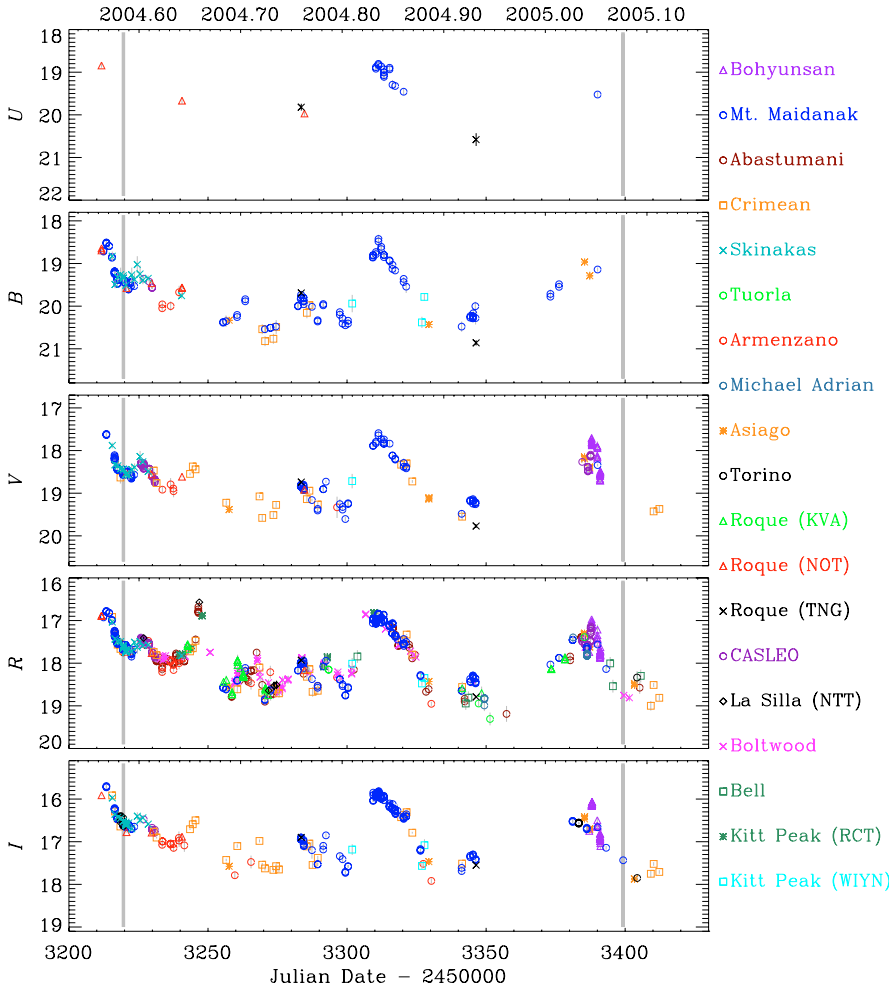
Fig. 1. UBVR light curves of AO 0235+164 during the observing season 2004–2005; vertical lines indicate the XMM-Newton pointings of August 2, 2004 and January 28, 2005. The ELISA contribution has been subtracted as explained in Raiteri et al. (2005).
