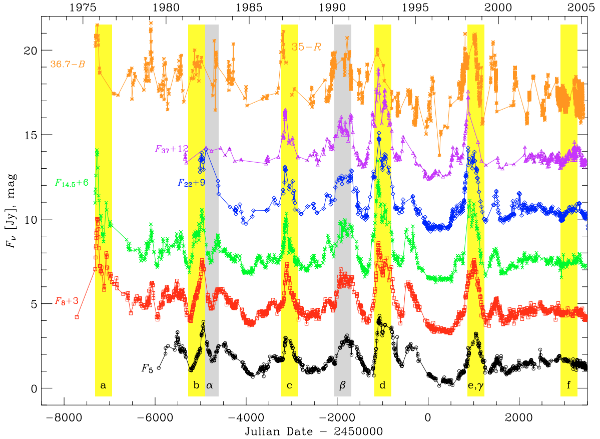
Fig. 7. Historical optical (mag) and radio (37, 22, 14.5, 8, and 5 GHz, flux density in Jy) light curves of AO 0235+164 shifted by the indicated amount; to increase the sampling in the optical, we show R -band data after JD = 2 447 000 and R -converted B -band data before. Yellow strips highlight the periods (a, b, c, d, e, f) where a major radio (and optical) outburst is expected on the basis of a 5.6 \pm 0.5 yr quasi-periodicity; periods \alpha , \beta , and \gamma belong to an \sim 8 yr characteristic time scale of variability.
