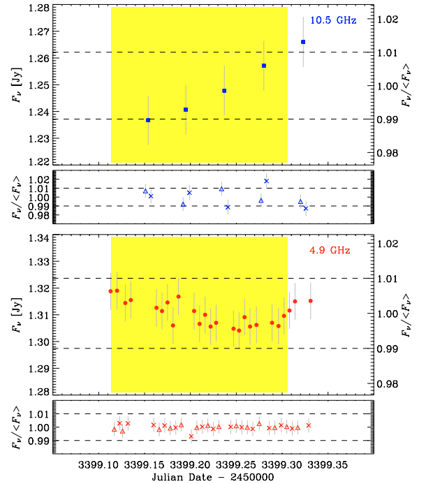
Fig. 6. Radio light curves of the source and calibrators at 10.5 GHz ( top , blue symbols) and 4.9 GHz ( bottom , red symbols) obtained with the 100 m radio telescope at Effelsberg on January 28, 2005. The two calibrators are 3C 067 (triangles) and 4C +09.11 (crosses). The horizontal lines indicate deviations of 1% from the mean flux densities, while the yellow areas highlight the period of the X-ray observations.
