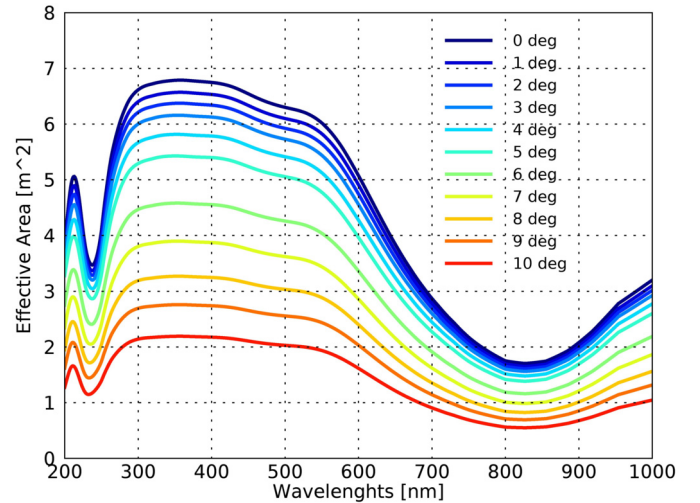
Fig. 13. The effective area of the ASTRI telescope as a function of wavelength. The different curves refer to different angular positions on the field of view.
