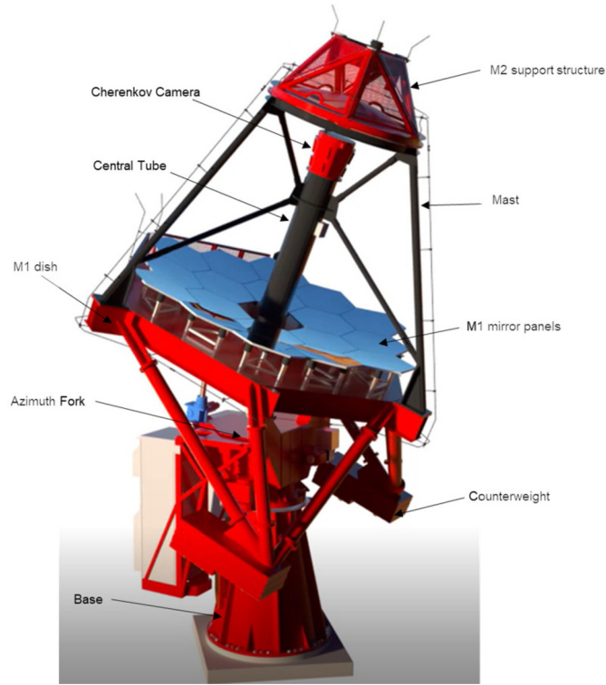
Fig. 10. 3D model of a telescope of the ASTRI mini-array. Some of the opto-mechanical components are explicitly listed.
