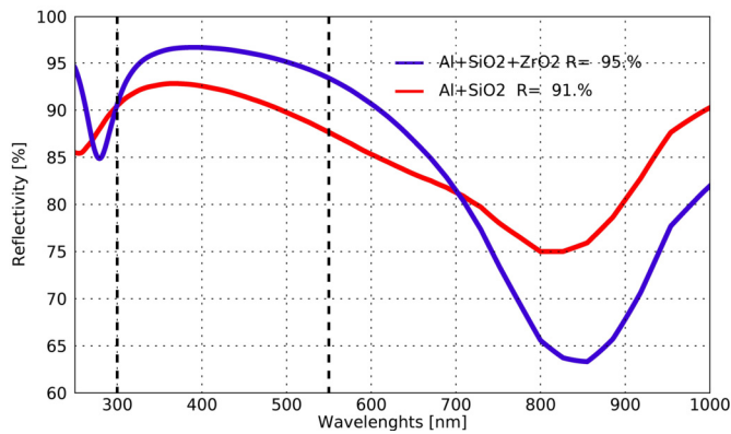
Fig. 11. Comparison between the Al+SiO 2 coating used in the ASTRI-Horn prototype telescope and the one (Al+SiO 2 +ZrO 2 ) used for the mirrors of the ASTRI Mini-Array telescopes. The vertical dashed lines mark the region of interest of Cherenkov astronomy.
