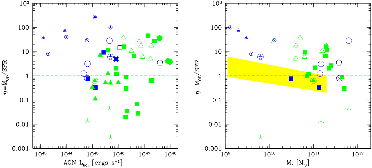
Fig. 4. Mass-loading factor \eta = \dot{M}_{\text{OF}}/\text{SFR} as a function of AGN bolometric luminosity ( left panel ), host galaxy stellar mass ( right panel ). The yellow band in the right panel is the range found by Heckman et al. (2015) for starburst driven galactic winds in a sample of local star-forming galaxies. Symbols as in Fig. 1.
