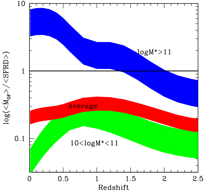
Fig. 12. Average mass-loading factor \langle \eta \rangle = \langle \dot{M}_{\text{OF}} D \rangle / \langle \text{SFR} D \rangle as a function of the redshift. Red = average; blue = M_* > 10^{11} M_\odot ; green = 10^{10} < M_* < 10^{11} M_\odot .
