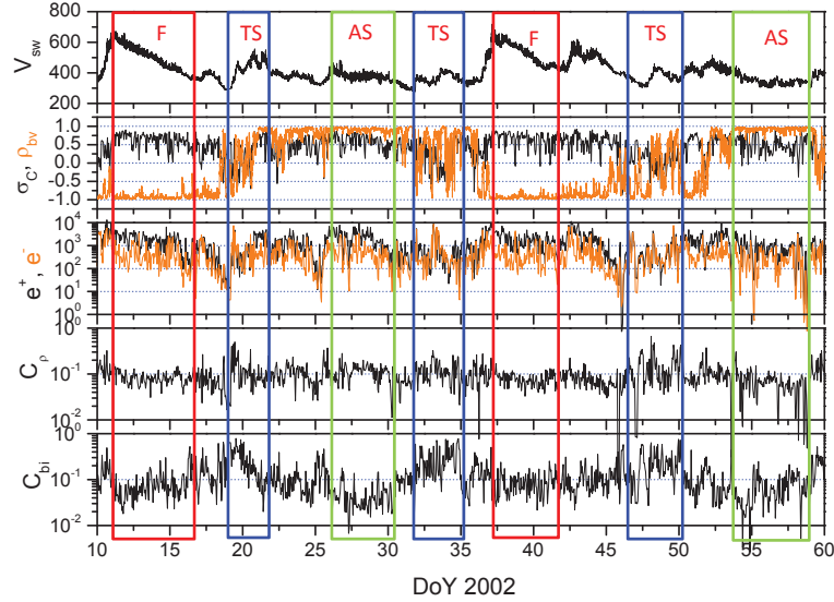
FIGURE 3. From top to bottom: proton bulk speed V_{sw} (in km/s), \sigma_C and \rho_{vb} (black and orange line respectively), e^+ and e^- in \text{km}^2/\text{s}^2 (black and orange line respectively), density compression C_\rho and magnetic field compression C_{bi} for fast ('F', red box), typical slow ('TS', blue box) and Alfvénic slow ('AS', green box) wind.
