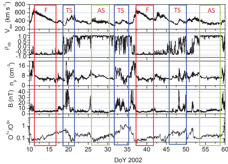
FIGURE 1. From top to bottom: bulk speed V_{sw} , correlation coefficient at 1 hr scale \rho_{vb} , proton number density n_p , magnetic field magnitude B, O^{7+}/O^{6+} for fast ('F', red box), typical slow ('TS', blue box) and Alfvénic slow ('AS', green box) wind.
