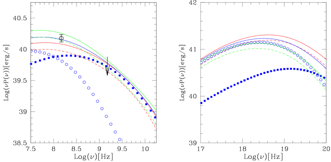
FIG. 3. Synchrotron (left) and IC (right) spectra obtained for \eta_B = 0.02 (red), 0.03 (blue), and 0.05 (green). Dashed lines (for \eta_B = 0.02 and 0.05 ) mark models assuming only primary electrons. The contribution from regions with larger (85% of cells in the volume) and shorter acceleration times (15% of the volume) are also marked with open and filled points, respectively, considering \eta_B = 0.03 . Radio data are taken from [14].
