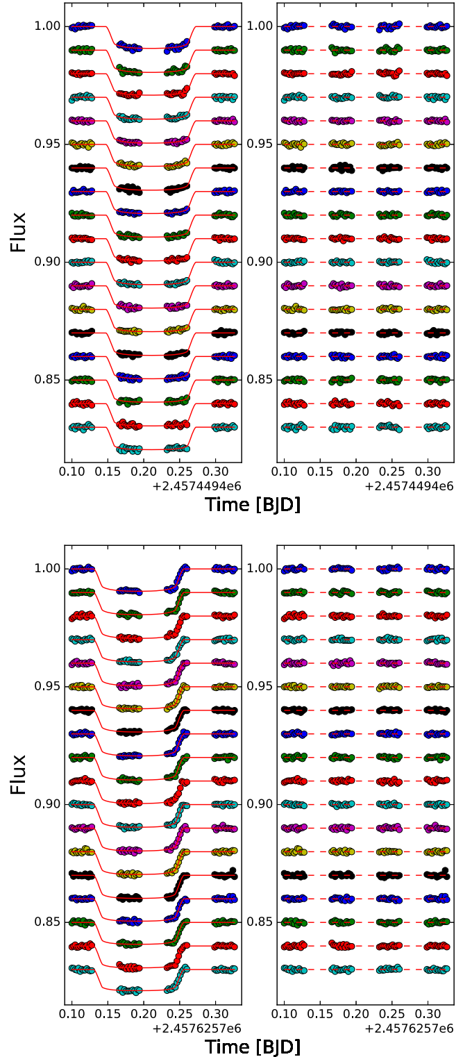
Figure 9. Same as Figure 8 but for HAT-P-38 b. First and second visit in top and bottom panel, respectively.
