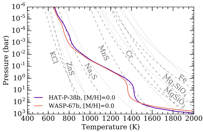
Figure 1. The P - T profiles of the two planets from this work and condensation curves from various molecules. From the intersection of the curves, alkali-bearing condensates are expected in the atmospheres of the planets. WFC3 observations probe the pressures between about 1 and 100 mbar.
