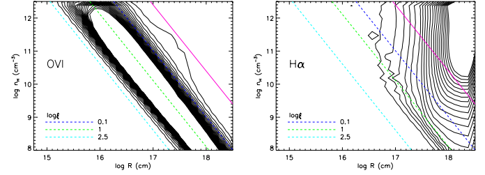
Fig. 5. Contour profiles of O VI and H \alpha as a function of density and distance, here using a radial slope \gamma of 0.10. The dashed lines indicate constant ionization parameters as detailed in the legend. The solid magenta line follows the density prediction of the pressure confined emission model of Baskin et al. (2014).
