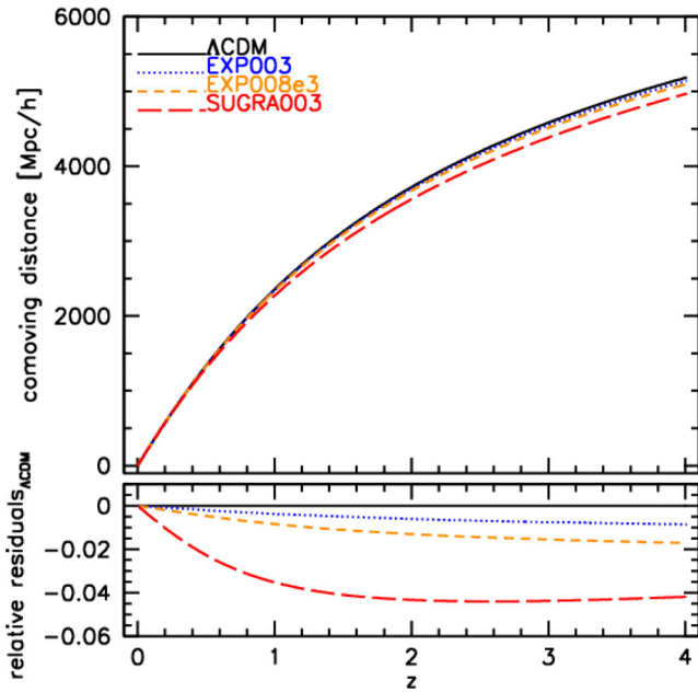
Figure 1. Comoving distances as a function of redshifts for the four considered models of the CoDECS suite. The bottom panel shows the relative difference of the models with respect to \Lambda\text{CDM} .
