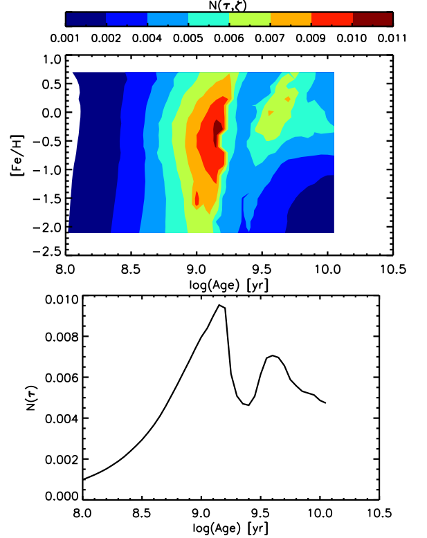
FIG. 13.— The expected distribution, N(\tau, \zeta) , for a sample of evolved stars selected with the same criteria as the local red giant sample in age, \tau , and metallicity, \zeta (top). We also examine the expected age distribution, N(\tau) , assuming a solar neighborhood MDF similar to that found by Hayden et al. (2015, bottom).
