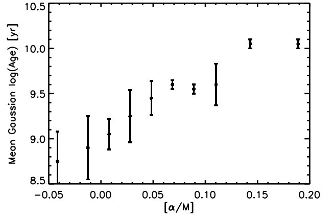
FIG. 14.— The mean \log(\text{age}) , \tau , of the \alpha -dependent Gaussian+uniform SFH models as a function of \alpha -abundance bin. The error bars indicate the dispersion of each Gaussian model. The mean age of the models increases continuously with \alpha -abundance, even at the youngest ( < 1 Gyr) ages.
