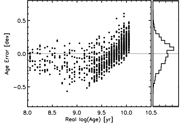
FIG. 9.— Age error as a function of true age for the simulated sample found using [\text{Fe}/\text{H}] , T_{\text{eff}} , M_{V_T} , and \log g as measured parameters for a Bayesian analysis. Using this method of age estimation, the young stars are assigned ages that are preferentially too old and the old stars are assigned ages that are preferentially too young. The right panel shows the histogram of age errors as shown in the lower right panel of Figure 7.
