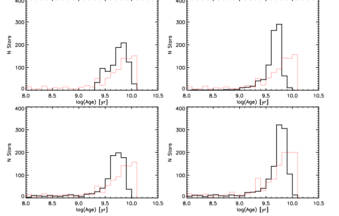
FIG. 8.— The distribution of the recovered ages from the simulated sample found using [\text{Fe}/\text{H}] and M (top left), [\text{Fe}/\text{H}] , T_{\text{eff}} , and \log g (top right), [\text{Fe}/\text{H}] , T_{\text{eff}} , and M_{V_T} (bottom left), [\text{Fe}/\text{H}] , T_{\text{eff}} , M_{V_T} , and \log g (bottom right). The red dashed line shows the distribution of true ages. The top panels are highly peaked around 4-6 Gyr. The bottom panels recover younger ages for the older stars, despite the narrower error distribution.
