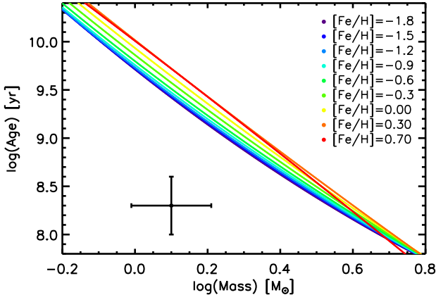
FIG. 4.— Each line represents the isochrone derived mass-age relation for a representative sample of metallicities. The color represents metallicity as indicated. The mass-age relation was fit to the PARSEC isochrone points of a single metallicity with a quadratic function in logarithmic space. Representative error bars are shown.
