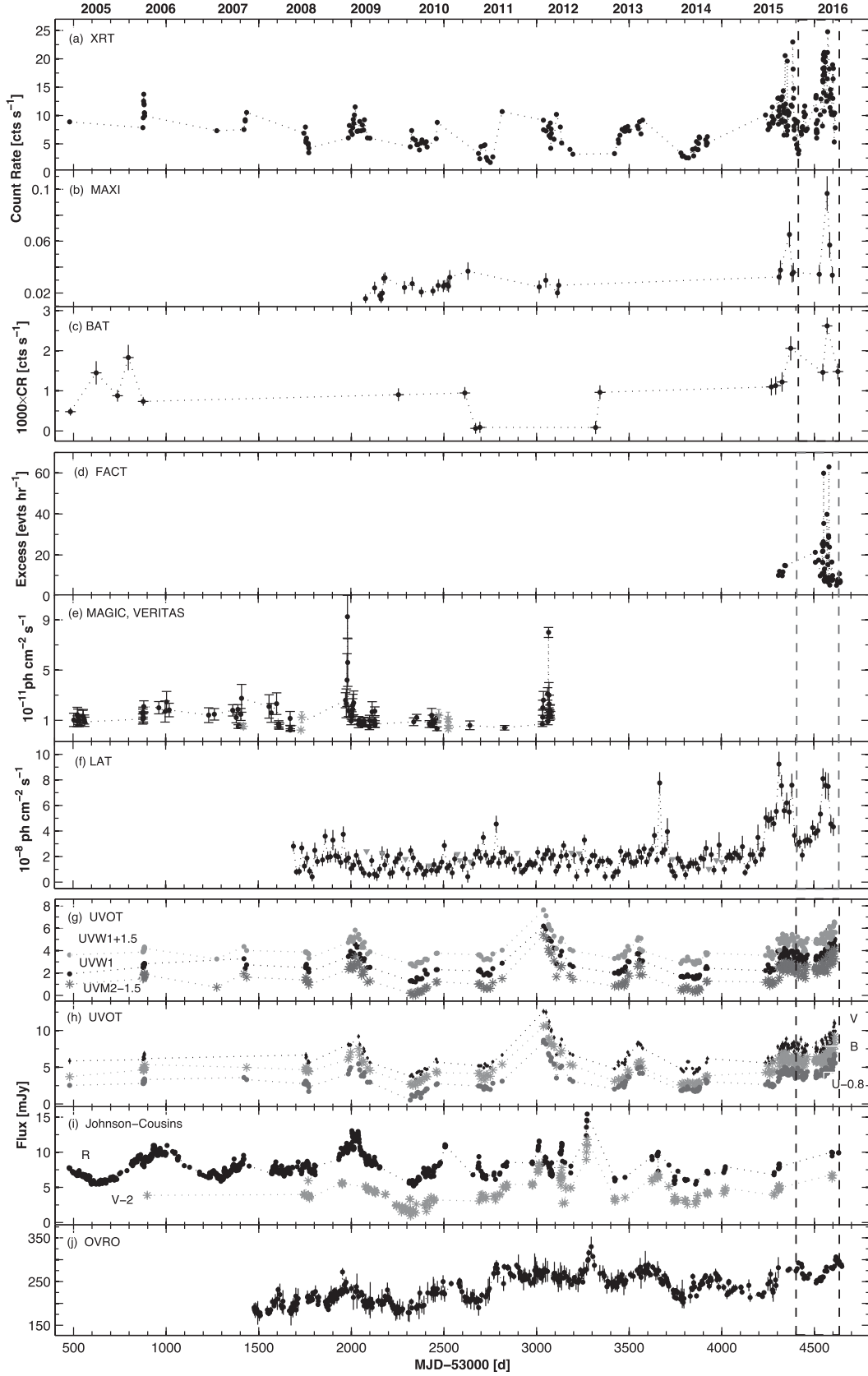
Figure 1. The historical light curves of 1ES 1959+650 from the MWL observations in 2005–2016 with XRT (top panel), MAXI (panel b), BAT (panel c), FACT (panel d), MAGIC and VERITAS (panel e), Fermi – LAT (panel f), UVOT (panels g and h), ground-based telescopes (panel i) and OVRO (panel j). We used daily bins for XRT, BAT , FACT , UVOT , Steward , OVRO data; 1 2 and 4-week bins for those of MAXI , LAT and BAT observations, respectively. The light curves between the vertical dashed lines correspond to the period 2016 January–August.
