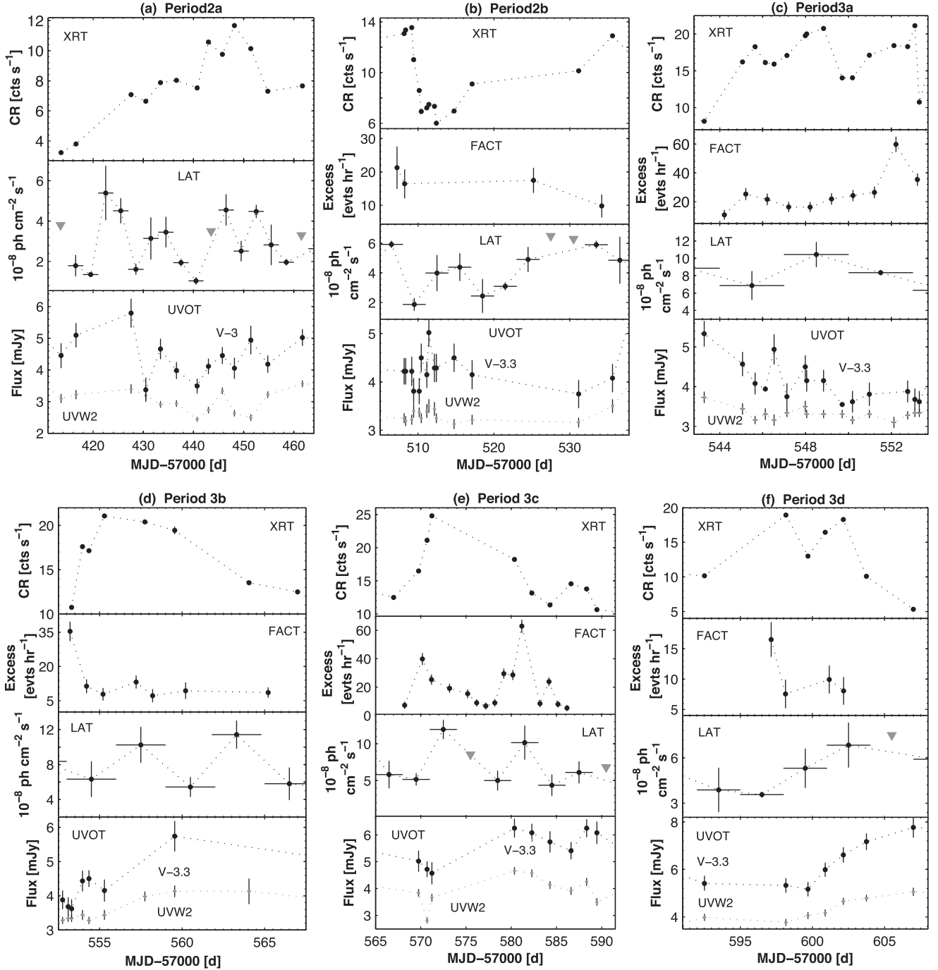
Figure 3. Multiwavelength variability of 1ES 1959+650 in different sub-periods. Grey triangles in panel b stand for upper limits to the LAT flux when the source was detected below the 3\sigma significance.
