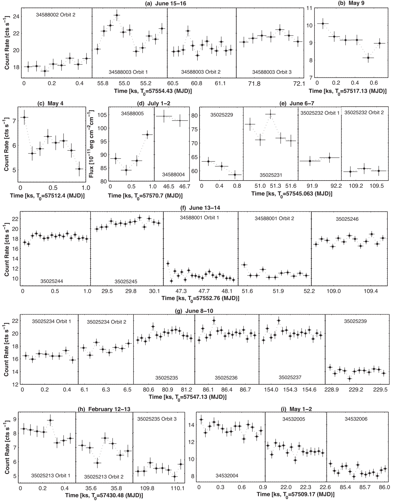
Figure 4. The most notable X-ray IDVs of 1ES 1959+650 in 2016 January–August.
