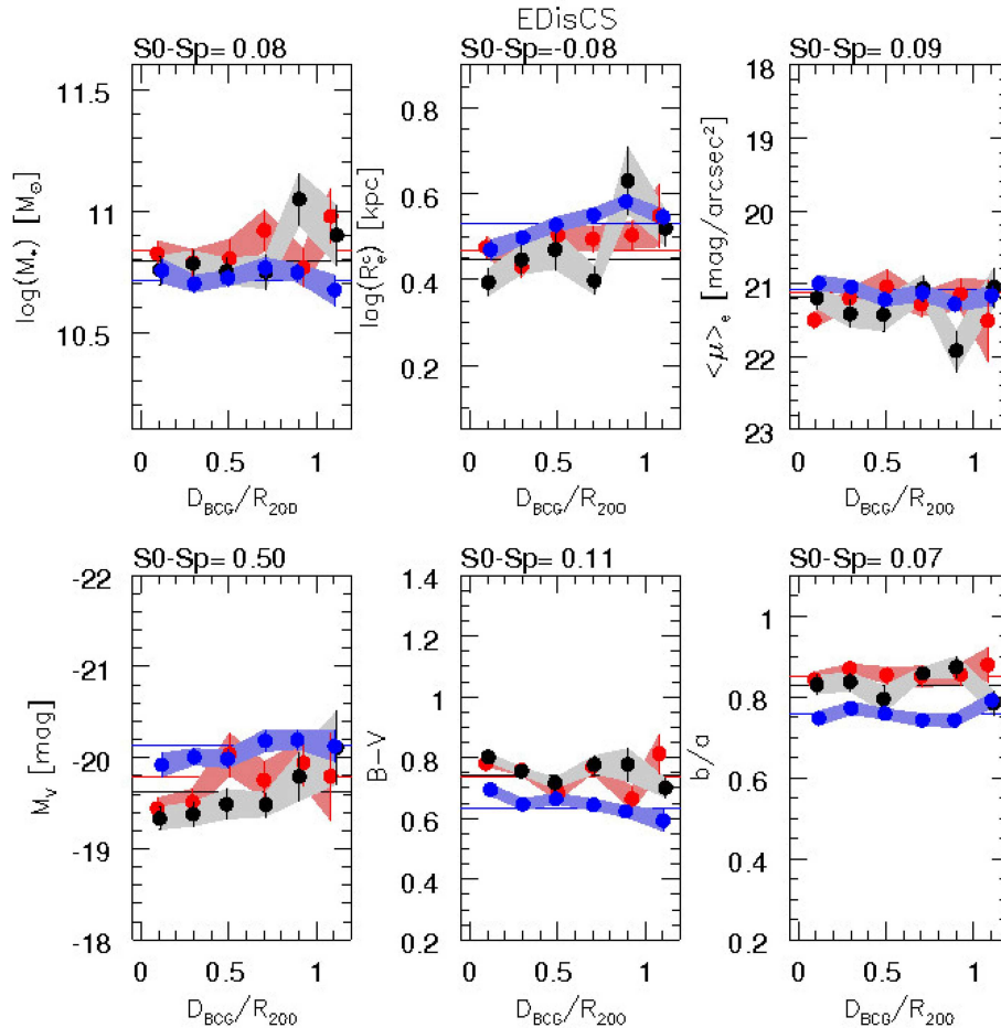
FIGURE 10 | The trend of the measured parameters for the EDisCS sample as a function of the cluster-centric distance.
