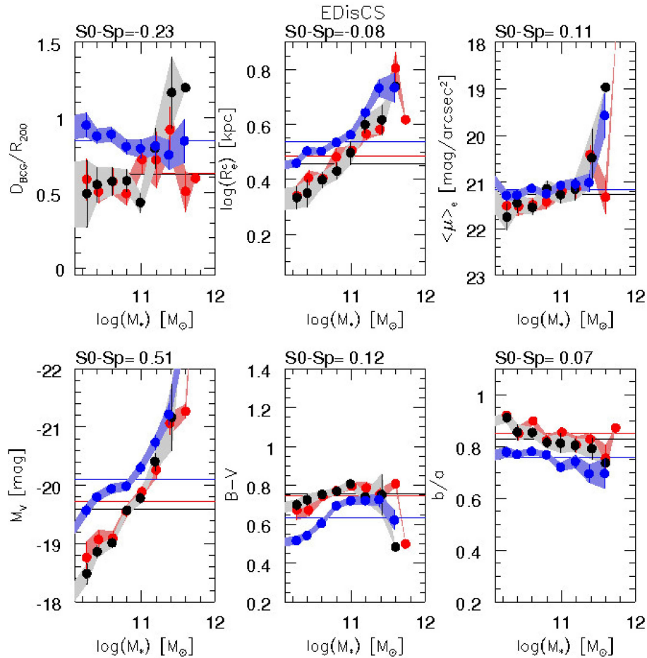
FIGURE 11 | The same trends as a function of galaxy masses.
