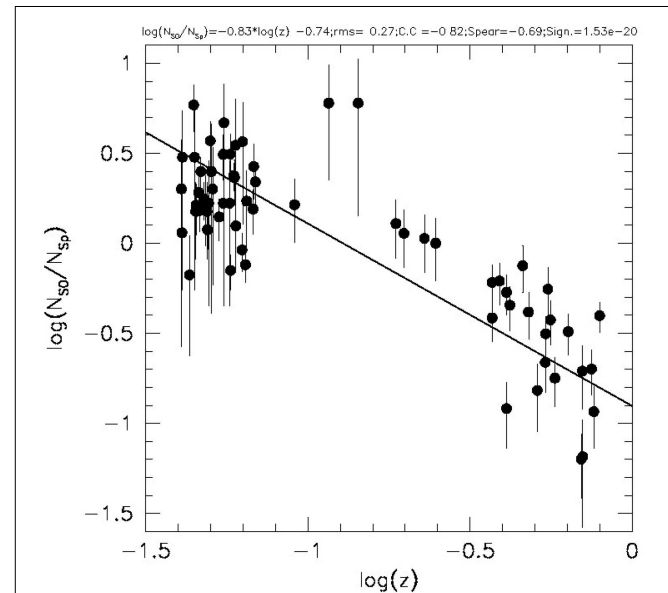
FIGURE 4 | The log of the N_{S0}/N_{Sp} ratio vs. the log of the redshift z . The solid line gives the best fit. Poissonian error bars mark the 1\sigma uncertainty of the observed counts.
