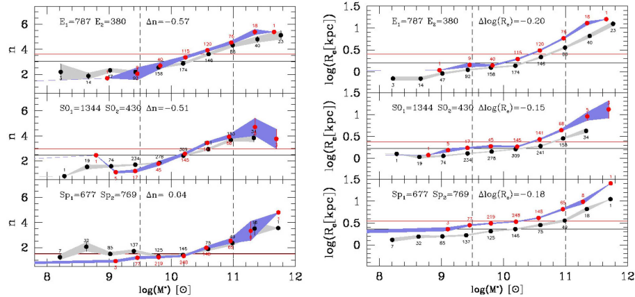
FIGURE 20 | Left: The Sérsic index of E's (upper panel), S0's (middle panel), and Spirals (lower panel) of galaxies in clusters (back dots and gray strips) and in the field (red dots and blue strips). Right: The effective radius in log units. Symbols as in the left panel.
