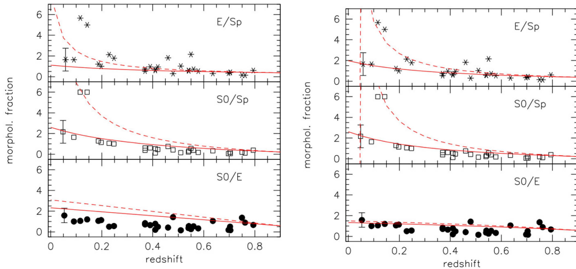
FIGURE 3 | Trend of the morphological fractions (E/Sp, S0/Sp, and S0/E) with redshift in various clusters. The WINGS stacked sample is shown with its 1\sigma error bar. The plotted lines mark the evolution of the morphological fractions for a hypothetical cluster that at high redshift has the mean morphological fractions of the EDisCS sample. Spirals transform into S0's and E's at different rates per interval of redshift. Left: The solid lines
