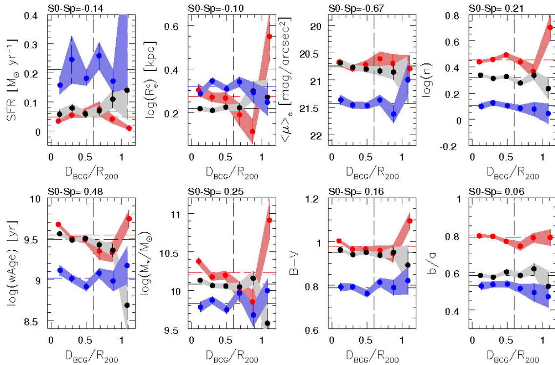
FIGURE 6 | From top left to bottom right we plot here vs. the cluster-centric distance in R_{200} units the following average quantities derived for the different morphological types in various bins of D_{BCG}/R_{200} : the star formation rate (SFR), the log of the circularized effective radius ( \log(R_e) ), the mean effective surface brightness ( \langle \mu \rangle_e ), the log Sersic index ( \log(n) ), the log of the luminosity weighted age ( \log(wAge) ), the log total mass ( \log(M_*) ),
