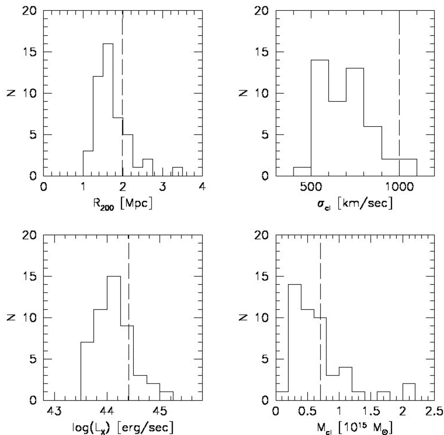
FIGURE 2 | From top left to bottom right we plot here the observed distributions of R_{200} , \sigma_{cl} , \log(L_X) , and M_{cl} for the WINGS clusters that belong to the stacked sample. The dashed line mark the values for the Coma cluster.
