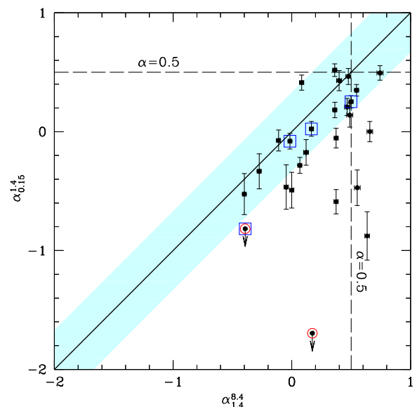
Figure 6. Radio spectral indices between 150 MHz and 1.4 GHz versus spectral indices between 1.4 GHz and 8.4 GHz of the AGN in CLASS with z > 4 (from Tables 1 and 2). Arrows indicate upper limits on \alpha_{0.15}^{1.4} (i.e. sources not detected in the TGSS at 150 MHz). The boxes mark the objects already confirmed as blazars in the literature while the red open circles mark the sources (GB6J090631+693027, GB6J160608 + 312504) classified as peaked radio spectrum by Coppejans et al. (2017). The continuous line is the 1:1 relation while the light blue shaded area indicates the expected spread (90 per cent confidence level) due to variability (see the text for details).
