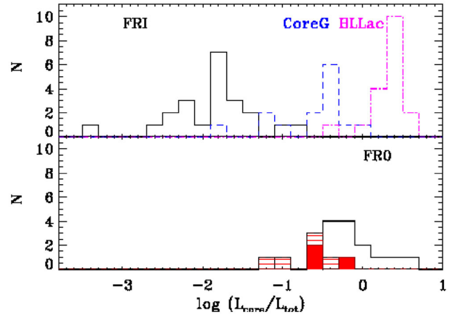
Figure 2. Histograms of the core dominance (adapted from B15) for – upper panel – 3CR/FRI (black solid line), CoreG (blue dashed line), and low-luminosity BL Lacs (magenta dot-dashed line). Lower panel – FR0s of B15 (red ticked line) and our sample of FR0s (black solid line). The red filled histograms are the sources in common with B15.
