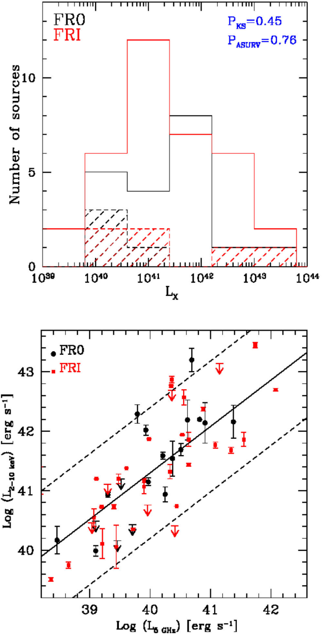
Figure 4. Upper panel: histogram of the X-ray luminosity for the FR0s of our sample (black solid line) and the comparative sample of FRIs (red solid line). No significant difference is observed between the two samples. The dashed histograms represent upper limits in each sample. In the plot the probabilities from the Kolmogorov–Smirnov test ( P_{\text{KS}} ) and the twost test in ASURV ( P_{\text{ASURV}} ) are also reported. Lower panel: 2–10 keV X-ray luminosity versus 5 GHz radio core luminosity for FR0s (black circles) and FRIs (red squares). Arrows indicate upper limits. The black solid line is the linear regression for the overall sample of FR0s and FRIs (excluding the upper limits): \log L_X = (7.8 \pm 0.6) + (0.8 \pm 0.1)\log L_{5\text{ GHz}} (see also Hardcastle et al. 2009). The black dashed lines are the uncertainties on the slope.
