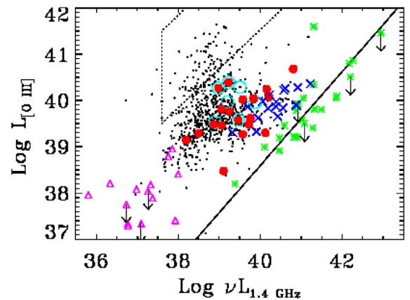
Figure 1. FIRST versus [O\text{ III}] luminosities (both in \text{erg s}^{-1} ) adapted from B15. Red points are the FR0s presented in this paper, while empty cyan circles are the FR0s of B15. The black dot points correspond to the SDSS/NVSS sample analysed by Baldi & Capetti (2010), the blue crosses are the low-luminosity BL Lacs studied by Capetti & Raiteri (2015), the empty pink triangles are the CoreG galaxies (Balmaverde & Capetti 2006), and the green stars are the FRIs of the 3CR sample. The dashed line marks the boundary of the location of Seyfert galaxies. The solid line represents the line-radio correlation followed by the 3CR/FRIs.
