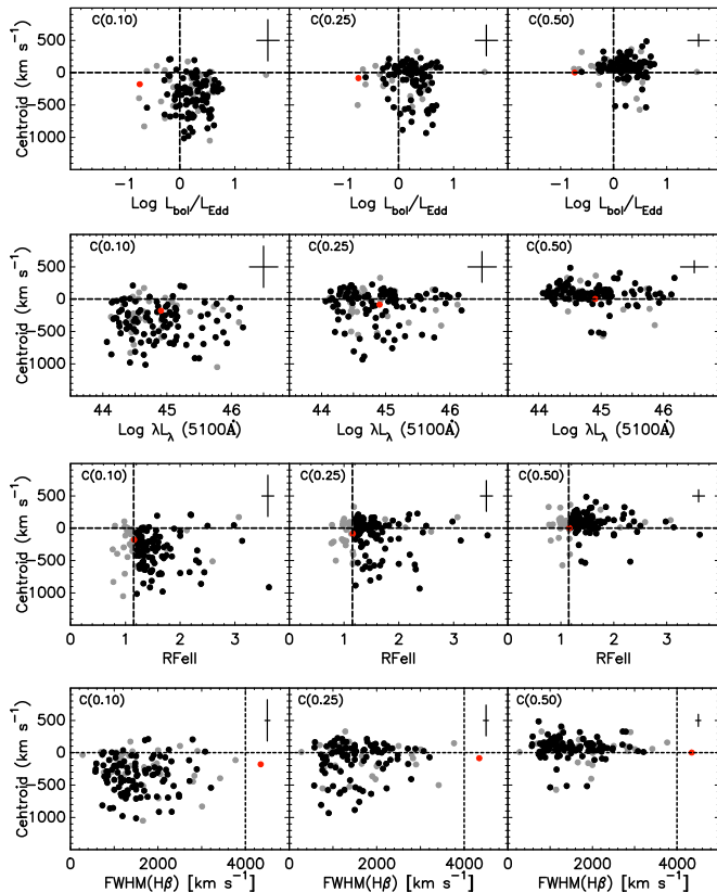
Fig. 10. Dependence of H\beta_{BC+BLUE} centroids c(0.10) , c(0.25) and c(0.50) on Eddington ratio (top row), luminosity at 5100 Å (second row from top), and the 4DE1 parameters R_{FeII} and FWHM(H\beta) (third and fourth rows, respectively). We note that almost all objects with H\beta_{BLUE} are Pop. A sources. Meaning of symbols is as in Fig. 1.
