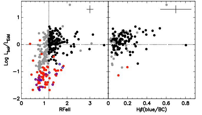
Fig. 9. Behavior of Eddington ratio as a function of R_{FeII} (left panel) and fraction of H \beta BLUE intensity (right). The black crosses are the average errors. Meaning of symbols is as in Fig. 1.
