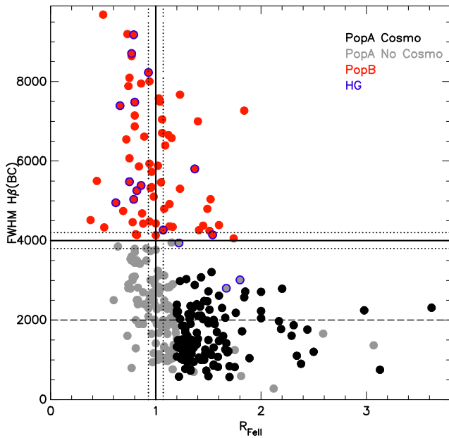
Fig. 1. Optical plane of the 4DE1 parameter space, \text{FWHM}(\text{H}\beta) vs. R_{\text{FeII}} , for the present sample. Black dots indicate sources chosen for the “Cosmo” sample, i.e., with R_{\text{FeII}} \geq 1.2 , and gray dots indicate the remaining Pop. A sources. Population B sources are indicated in red. A blue contour identifies sources with weak host galaxy contaminations in their spectrum (labeled as HG). Vertical line separates the objects with R_{\text{FeII}} > 1 . This criteria is used to identify the extreme accretors. The filled horizontal line separates populations A and B, according to Sulentic et al. (2000). Dotted lines indicate the typical error associated to R_{\text{FeII}} and the \text{FWHM}(\text{H}\beta) . Dashed horizontal line delimits the region of NLSy1s ( \text{FWHM}(\text{H}\beta) < 2000 \text{ km s}^{-1} ).
