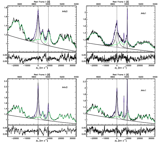
Fig. 6. As in Fig. 4, but for spectral type A4.
