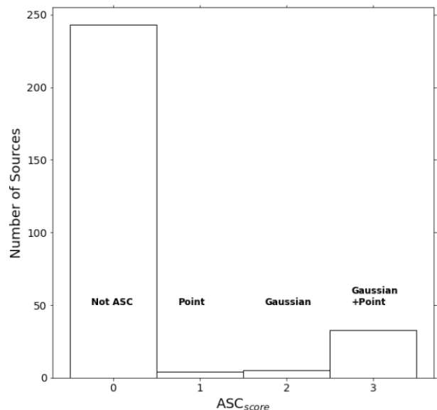
Figure 14. Distribution of ASC_{\text{score}} assigned to the TEMPO detected fragment sample. Individual scores per source are given in Table 4.
