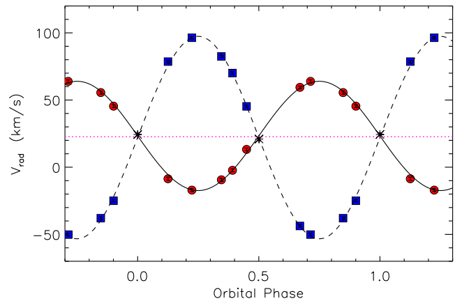
Figure 5. RV curve of the binary system V1481 Ori phased with the orbital period P = 4.433 d. Circles and squares refer to the primary and the secondary components, respectively, while asterisks are used when the two components were not resolved in the spectra. The RV errors are also shown and are smaller than the symbol size. The solid and dashed lines represent the circular orbital solutions for the primary and secondary components, respectively, whereas the dotted line is the mean barycentric RV value.
