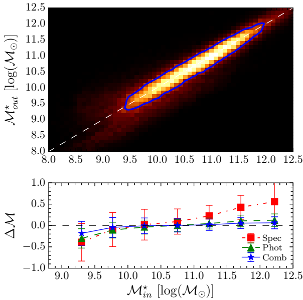
Fig. 4. Comparison of the stellar mass measurements M_{\text{out}}^* obtained using GOSSIP+ on the 180 000 simulated M_{\text{in}}^* sample with the input values. Top panel: the density plot represents the measurement of M_{\text{out}}^* from the combined fit versus the input M_{\text{in}}^* . The highest density is represented by the brightest colour, while the lowest density is represented in black. The blue line represents the 1\sigma contour of the distribution. The combined fit is able to find the correct M_{\text{out}}^* at any mass in the simulated range. Bottom panel: evolution of the quantity \Delta M = M_{\text{in}}^* - M_{\text{out}}^* over the stellar mass range. The points in red, green, and blue represent the fit on the spectroscopy only, photometry only and on the combined data, respectively. The combined fit leads to the most accurate M_{\text{out}}^* computation with \Delta M_{\text{out}}^* < 0.1 dex.
