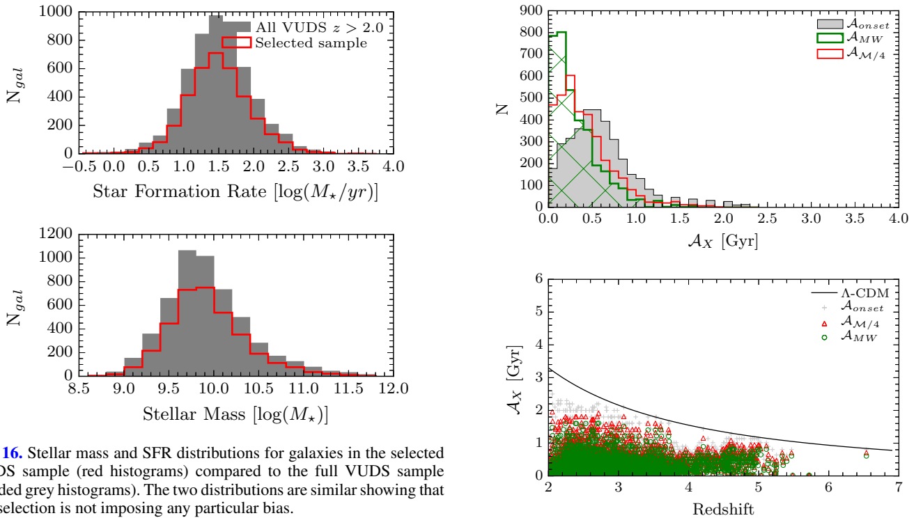
Fig. 17. Age distributions of 3597 VUDS galaxies computed from the combined fit of the spectroscopy and the photometry as described in Sect. 3. Top panel: the three distributions in red, hatched green, and filled grey histograms correspond to the three definitions of age we use in our paper and defined in Sect. 4, \mathcal{A}_{\text{onset}} , \mathcal{A}_{\text{MW}} , and \mathcal{A}_{\text{M}/4} , respectively. Bottom panel: age distributions of VUDS galaxies as a function of observed redshift z_{\text{obs}} . The three age definitions, \mathcal{A}_{\text{onset}} , \mathcal{A}_{\text{MW}} , and \mathcal{A}_{\text{M}/4} are presented in red, green, and grey, respectively. The line represents the age of the Universe in the \Lambda -CDM cosmological model. The lowest age corresponds to the smallest possible age allowed by our model library (50 Myr). The upper limit is in general lower than the age of the Universe.
