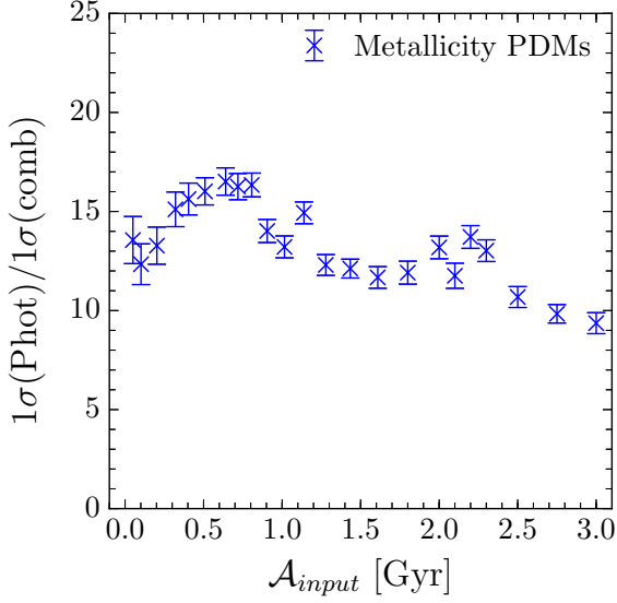
Fig. 12. Comparison of the 1\sigma area from fit on the photometry and the fit on the combined data as function of the input \mathcal{A}_{\text{onset}} for the age-metallicity relation. At any age, the 1\sigma(\text{phot}) area based on the photometry is on average 13.3 times bigger than the 1\sigma(\text{comb}) area, based on the combined fit. The error bars are computed from the median absolute deviation.
