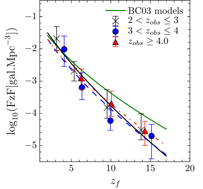
Fig. 24. Comparison of the FzFs from different stellar population synthesis models. In green, a global FzF computed from all the point presented in Fig. 22, derived with exponentially delayed SFH and BC03 models. In black, blue and red, we show the FzFs derived from M05 models as well as their fits in 3 observed redshift bins: 2 < z_{\text{obs}} \leq 3 , 3 < z_{\text{obs}} \leq 4 , and z_{\text{obs}} \geq 4.0 , respectively.
