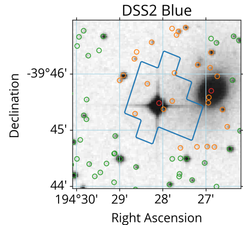
Figure 1. 3' \times 3' DSS2 (blue filter) image with the Sectors 10 SPOC photometric aperture outlined in blue. Colored circles denote the positions of Gaia DR2 sources within 2' of TOI-763; the red circle inside the aperture is TOI-763 (6140553127216043648), the red circle outside the aperture is a galaxy (6140553157278886400), the orange circles are potentially diluting sources, and other sources are in green. We establish a dilution of < 1\% for TOI-763 based on the flux contributions of all sources.
