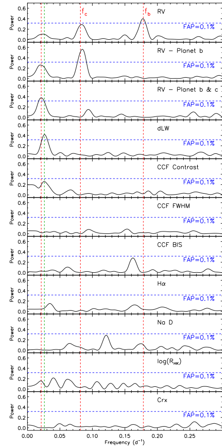
Figure 4. From top to bottom: GLS periodogram of: the HARPS RV measurements (upper panel); the RV residuals following the subtraction of the signal of TOI-763 b (second panel); the RV residuals following the subtraction of the signals of TOI-763 b and c (third panel); the dLW (fourth panel); the CCF's contrast (fifth panel); the CCF's FWHM (sixth panel); the CCF's BIS (seventh panel); the H \alpha line index (eighth panel); the Na D lines index (ninth panel); the Ca II H & K lines activity indicator (tenth panel); the Crx index (bottom panel). The dashed vertical red lines mark the orbital frequencies of TOI-763 b and c ( f_b = 0.178 \text{ days}^{-1} and f_c = 0.081 \text{ days}^{-1} , respectively), and of the additional signal found in the HARPS RVs ( 0.021 \text{ days}^{-1} ). The dashed green line is the frequency of the dLW peak (fourth panel from the top). The horizontal dashed blue lines mark the false alarm probability of \text{FAP} = 0.1\% , determined using the bootstrap randomization method described in Sect. 3.2.
