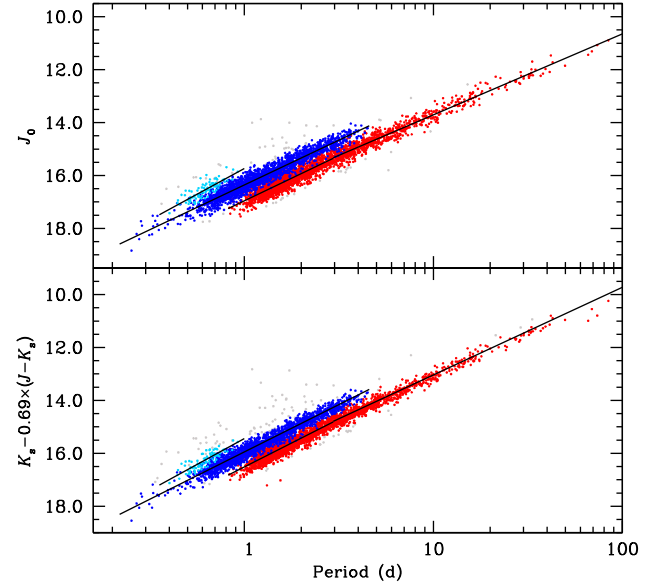
Figure 5. As in Fig. 4, but for the J filter.
