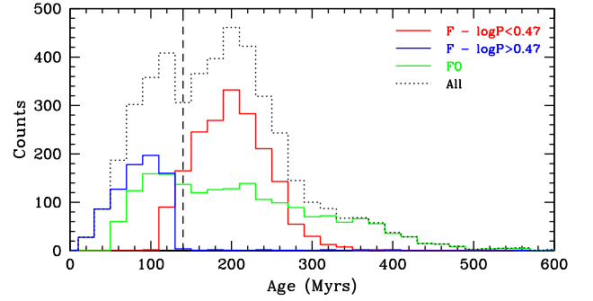
Figure 9. Distribution of the individual ages for the CCs analysed in this work as obtained by means of the PAC relations (after Bono et al. 2005). The vertical dashed line at 140 Myr is the boundary between young and old CCs.
