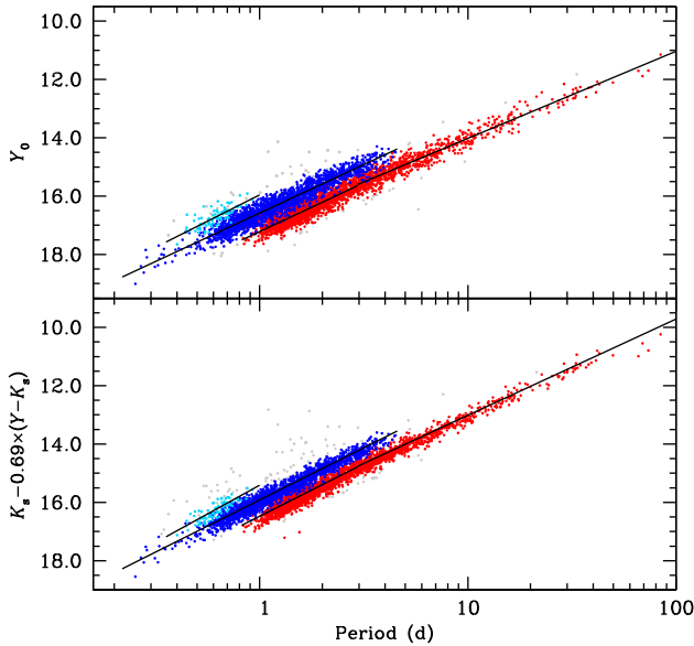
Figure 4. PL(Y) and PW(K_s, Y) relations for the SMC CCs investigated in this paper. F, 10 and 20 pulsators are shown as red, blue and light blue filled circles, respectively. The grey filled circles show objects excluded from the analysis because they deviate more than 3.5\sigma from the best fits to the data represented by solid lines.
