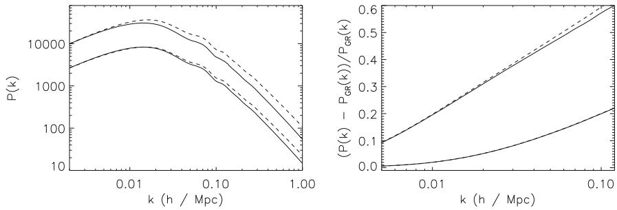
Fig. 32 Left panel: Linear matter power spectra for \Lambda\text{CDM} (solid line; M_0^{-1} = 0 , \nu = 1.5 ) and scalaron (dashed line; M_0^{-1} = 375 [10^{28} \text{ h}^{-1} \text{ eV}^{-1}] , \nu = 1.5 ) cosmologies. The modification to gravity causes a sizeable scale dependent effect in the growth of perturbations. The redshift dependence of the scalaron can be seen by comparing the top and bottom pairs of power spectra evaluated at redshifts z = 0.0 and z = 1.5 , respectively. Right panel: The environmental dependent chameleon mechanism can be seen in the mildly nonlinear regime. We exhibit the fractional difference (P(k) - P_{\text{GR}}(k)) / P_{\text{GR}}(k) between the f(R) and GR power spectra for the model (1.8.37) with parameters M_0^{-1} = 375 [10^{28} \text{ h}^{-1} \text{ eV}^{-1}] and \nu = 1.5 . The dashed lines represent linear power spectra ( P(k) and P_{\text{GR}}(k) calculated with no higher order effects) and the solid lines are the power spectra calculated to second order. We see that the nonlinearities decrease the modified gravity signal. This is a result of the chameleon mechanism. The top set of lines correspond to z = 0 and the bottom to z = 0.9 ; demonstrating that the modified gravity signal dramatically decreases for larger z . This is due to the scalaron mass being much larger at higher redshifts. Furthermore, nonlinear effects are less significant for increasing z
