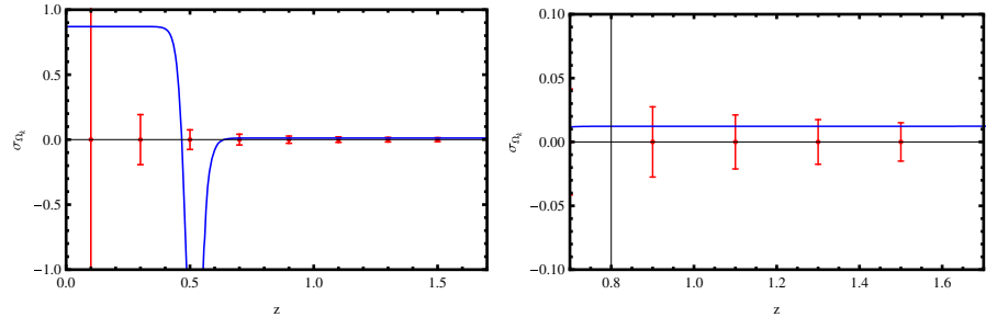
Fig. 60 Left: same as Fig. 59 but now with superimposed the prediction for the Lemaître–Tolman–Bondi model considered by García-Bellido and Haugbølle (2008a). Right: zoom in the high-redshift range
