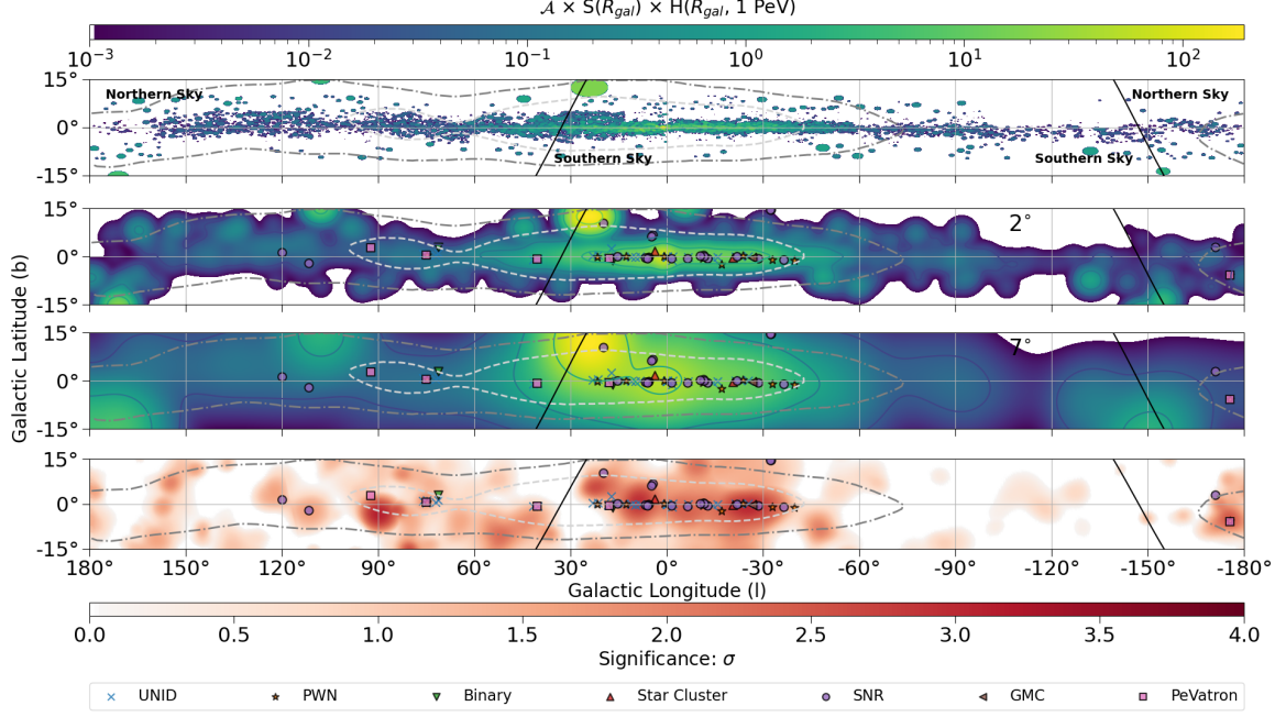
Figure 12. Top panel: the density distribution of \mathcal{A} \times S(R_{gal}) \times H(R_{gal}, 1 \text{ PeV}) in the Galactic plane for [96] type GCR source distribution (i.e., Case-IIb). Middle panels: the angular size of the GMCs are smeared by 2 and 7^\circ to include an angular uncertainty of their positions. Bottom panel: the neutrino significance map of the Galactic plane as recently observed by the IceCube detector [1]. The TeVcat & LHAASO PeVatrons gamma-ray sources, which are spatially correlated with the observed neutrino significance, are also plotted here.
