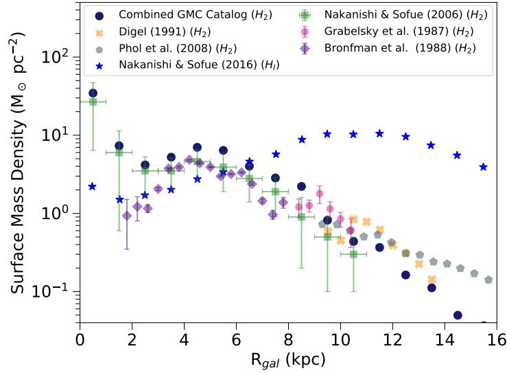
Figure 3. The distribution of H_2 surface mass density ( \Sigma_{H_2}^{\text{GMC}} ) along the galactocentric radius ( R_{\text{gal}} ). The blue star markers represent the variation in surface mass density of diffused atomic hydrogen gas in the MW Galaxy. The data points are extracted from figure 9 in [54] and figure 3.5 in [70], and corresponds to [64] in orange colour, [65] in gray colour, [66] in blue colour, [61] in green colour, [63] in pink colour and [62] in violet colour points respectively.
