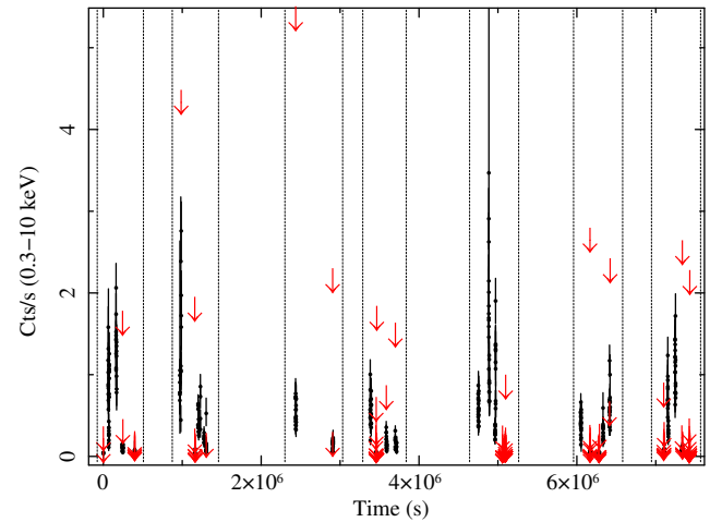
Figure 1: XRT lightcurve of IGR J18027-2016 in the 0.3-10 keV energy band. The bin time of the lightcurve is 100 s. The source count-rate estimated in the time bins where a detection above 3\sigma was achieved is represented in black, together with the corresponding uncertainty. Upper limits on the source non-detection are indicated with red arrows. The 7 orbital periods of the source monitored by XRT are separated by vertical dashed lines.
