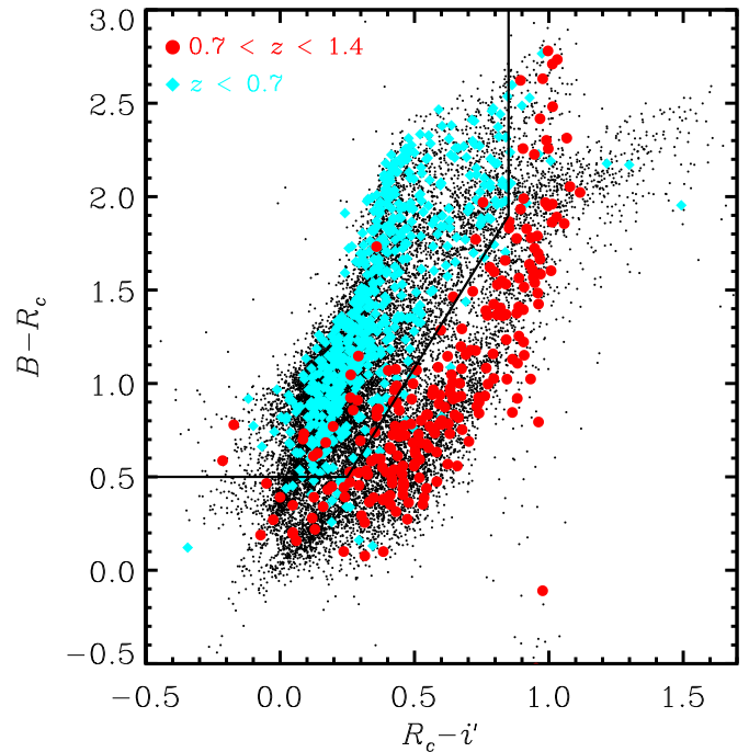
Figure 10. B - R_c vs. R_c - i' color-color distribution for all sources with R_c < 23.5 in the Subaru imaging catalogs of Furusawa et al. (2008). The cyan and red points correspond to those objects with spectroscopic redshifts in the ranges z < 0.7 and 0.7 < z < 1.4 , respectively. The solid black lines show the color cuts employed to prioritize target selection (see Equation (A3)).
