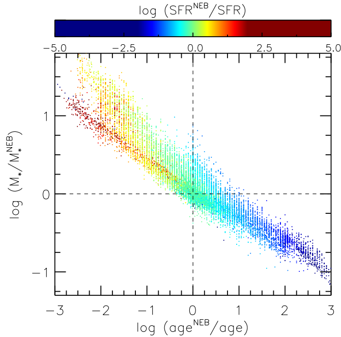
Figure 5. Ratio between masses estimated without ( M_* ) and with ( M_*^{\text{NEB}} ) nebul emission as a function of the ratio between ages as inferred from the fit with ( \text{age}^{\text{NEB}} ) and without ( \text{age} ) nebul emission, for the GOODS-S field and using the estimates from Methods 6a r and 6a r NEB . Symbols are color-coded according to the ratio of their SFRs.
