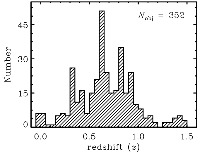
Figure 11. Distribution of the 352 unique, secure ( Q = -1, 3, 4 ) redshifts included in the Magellan/IMACS redshift catalog.
