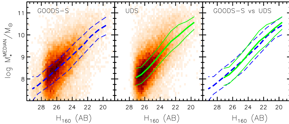
Figure 6. Reference median stellar mass (see Section 5.1) as a function of the observed H_{160} band magnitude in GOODS-S (left panel) and UDS (central panel). The color reflects the density of sources, increasing from lightest to darkest on a linear scale. Thick lines show the median mass in bins of one magnitude, while thin lines show the semi interquartile range in the same bins. Medians and semi interquartile ranges are also reported in the right panel for a direct comparison between the two fields (GOODS-S: blue dashed; UDS: green solid).
