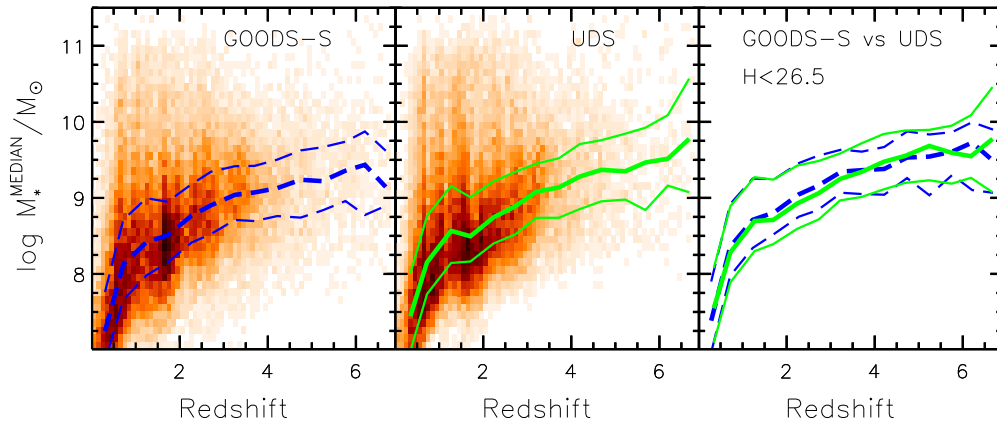
Figure 7. Reference median stellar mass (see Section 5.1) as a function of redshift in GOODS-S (left panel) and UDS (central panel). Colors and line styles are as in Figure 6. Thick lines show the median mass in bins of redshift ( \Delta z = 0.5 ), while thin lines show the semi interquartile range in the same bins. The right panel shows medians and semi interquartile ranges for the two samples cut at H_{160} < 26.5 .
