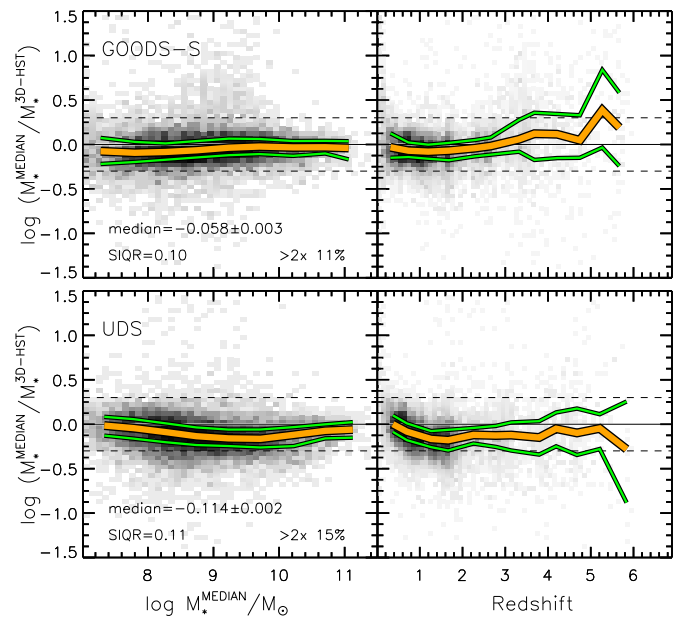
Figure 9. Ratio between CANDELS median masses and 3D-HST masses as a function of CANDELS median masses (left panels) and CANDELS redshifts (right panels) for the GOODS-S field (upper panels) and the UDS field (lower panels). Only sources whose redshifts differ by less than 0.1 have been considered. Colors and line styles are as in Figure 2.
