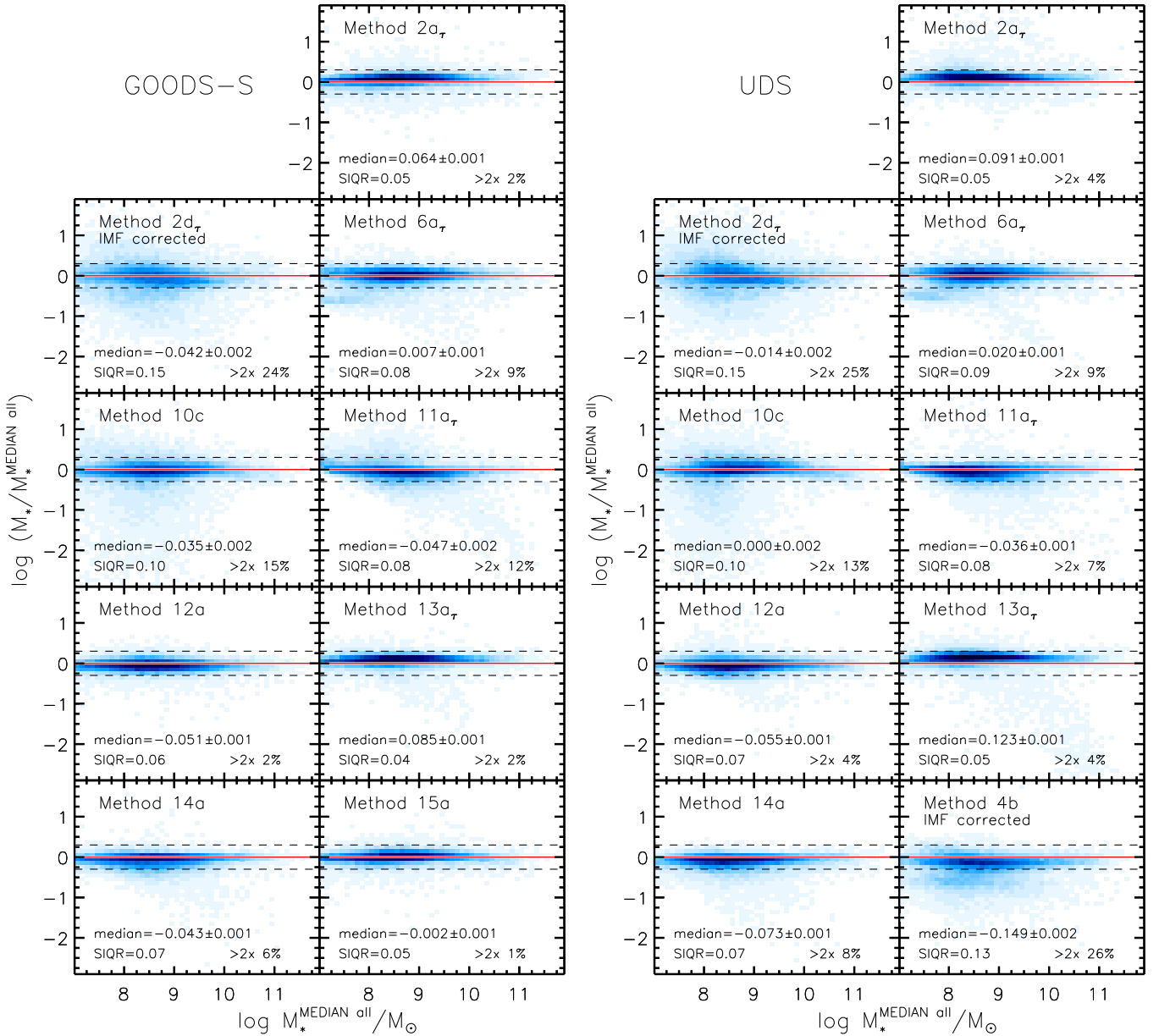
Figure 1. Comparison between the ratio of the different stellar mass estimates and the median mass for the GOODS-S (left panels) and the UDS (right panels) samples. All masses have been rescaled to the same Chabrier IMF. The plane is colored according to the density of sources, increasing from lightest to darkest shades on a linear scale. The red solid horizontal line indicate null difference with respect to the median mass, while the black dashed lines enclose the region where the difference is within a factor of 2. The median logarithmic ratio with the associated error and the semi interquartile range (SIQR, see text) are printed in each panel, as well as the fraction of sources differing from the median value by more than a factor of 2 (i.e., falling beyond the dashed lines).
