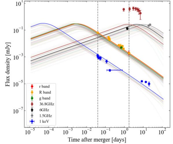
Figure 6. Multiwavelength afterglow light curves (see Section 3.2.3). For each band, the light curves predicted by the standard model are shown: r , R , and g bands (red, yellow, and green, respectively), 36.8 GHz (brown), 6 GHz (black), 1.5 GHz (grey), X-ray light curve (blue colour). The vertical lines pinpoint the epochs of the SEDs, illustrated in Fig. 7.
