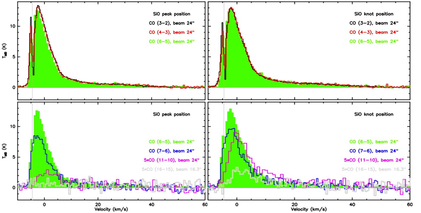
Fig. 3. CO transitions in the SiO peak (left panels) and knot (right panels) positions indicated in figure 2: APEX (3–2), black line ; (4–3), red line ; (6–5), green line and histograms (upper panels); (7–6), dark blue lines ; SOFIA (11–10), pink lines and (16–15), grey lines (lower panels, overlaid on the green histograms of the 6–5 transition). The last two were multiplied by five for comparison purposes. Respective spectral resolutions are 0.33, 0.50, 0.64, 0.54, 0.90 and 0.62 km s -1 . The vertical dotted line marks the cloud velocity, -4.5 km s -1 (Bourke et al. 1995b).
