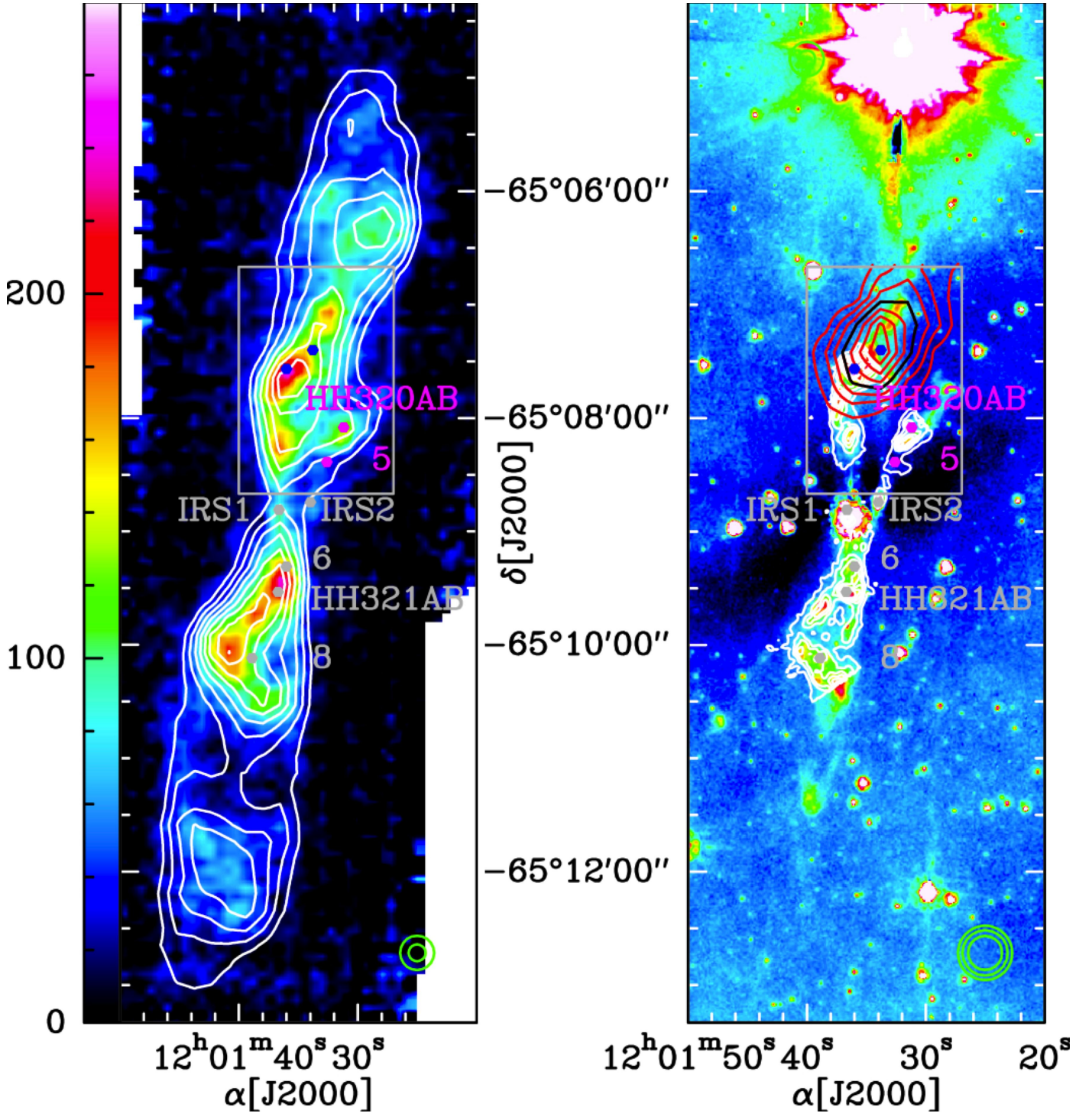
Fig. 1. The BHR71 bipolar outflow in its entirety, in Left : CO (6–5) (colours, associated with the wedge, in main beam temperature units, \text{K km s}^{-1} ) and (3–2) (white contours, from 30% to 100% of the signal in steps of 10%), both observed by the APEX telescope and integrated between -50 and +50 \text{ km s}^{-1} , with the resolutions indicated by green circles in the lower right corner; Right : the 8 \mu\text{m} emission detected by the Spitzer /IRAC receiver (colours, N09), with the \text{H}_2 0–0 S(5) emission as observed by the Spitzer /IRS receiver in the inner parts of the outflow (white contours, from G11), and the SiO (5–4) emission (red and black contours, G11) in the upper lobe (the green circles in the lower right corner show the respective resolutions of CO (3–2), (11–10), and SiO (5–4)). On both maps, the grey inset is the field shown in figure 2, the SiO peak and knot positions are indicated in blue, the knot 5 and HH320 region are in pink, and the IRS 1&2, knots 6, 8, and HH321 region are indicated by grey dots.
