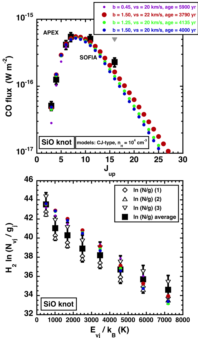
Fig. 6. Our model-observations comparisons. Upper panel: CO flux diagram over a beam of 24'' ; the observations in the SiO knot position are the black squares, and the model results are the coloured circles (see text). The CO (16–15) observational point is corrected for beam-size effect. The uncorrected point is the upper limit (see text), indicated by the grey arrow in this panel. Lower panel: \text{H}_2 excitation diagram for the SiO knot position, extracted following the different procedures described in the text (empty symbols), global average in black squares, and model results in coloured circles (see text, with the same code as in the upper panel).
