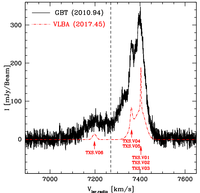
Fig. 7. Comparison between the total intensity spectra ( I ) of the H 2 O gigamaser detected towards TXS 2226-184 with the GBT in epoch 2010.94 (black histogram) and the combination (red dot-dashed line) of all the eleven Gaussian components determined for the six H 2 O maser features (TXS.V01–TXS.V06) detected with the VLBA in epoch 2017.45. The red arrows indicate the velocities of the total intensity peak of the different maser features (see Table 3). The dashed black line indicates the systemic velocity of the galaxy in the radio convention (i.e., 7270 km s -1 ).
