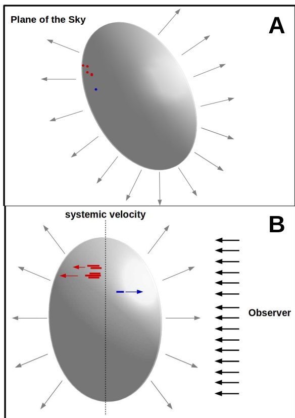
Fig. 10. Drawing sketch of the proposed location of the \text{H}_2\text{O} maser features. The gray ellipsoid represents the molecular gas where the maser emission originates, the gray arrows around the ellipsoid represent the expansion directions of the shock that inverted the population of the maser levels. The top panel (A) shows the location of the maser features as projected on the plane of the sky (see Fig. 9). The red dots are the red-shifted maser features (TXS.V01 – TXS.V05) with respect to the systemic velocity of the galaxy, the blue dot is the blue-shifted maser feature (TXS.V06). The bottom panel (B) shows the proposed location of the maser features as seen from east, therefore the point of view of the observer is on the right of the image (black arrows). The red segments are the amplification paths of the red-shifted maser feature (TXS.V01 – TXS.V05), the blue segment is the amplification path of the blue-shifted maser feature (TXS.V06). The length of the segments are not physical, the different length indicates the different peak flux density (see Table 6). The size and versus of the red and blue arrows (pointing towards left and right, respectively) indicate the velocity difference between the maser features and the systemic velocity (dotted vertical line) of the galaxy.
